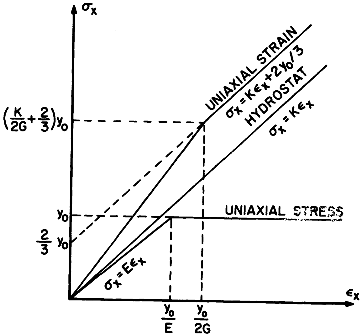
Figure 5. Stress-strain Behavior for an Elastic-perfectly Plastic Material in Uniaxial Stress and Uniaxial Strain.
