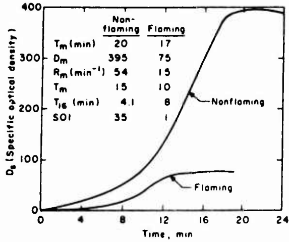
Figure 3. Typical smoke development from red oak.
