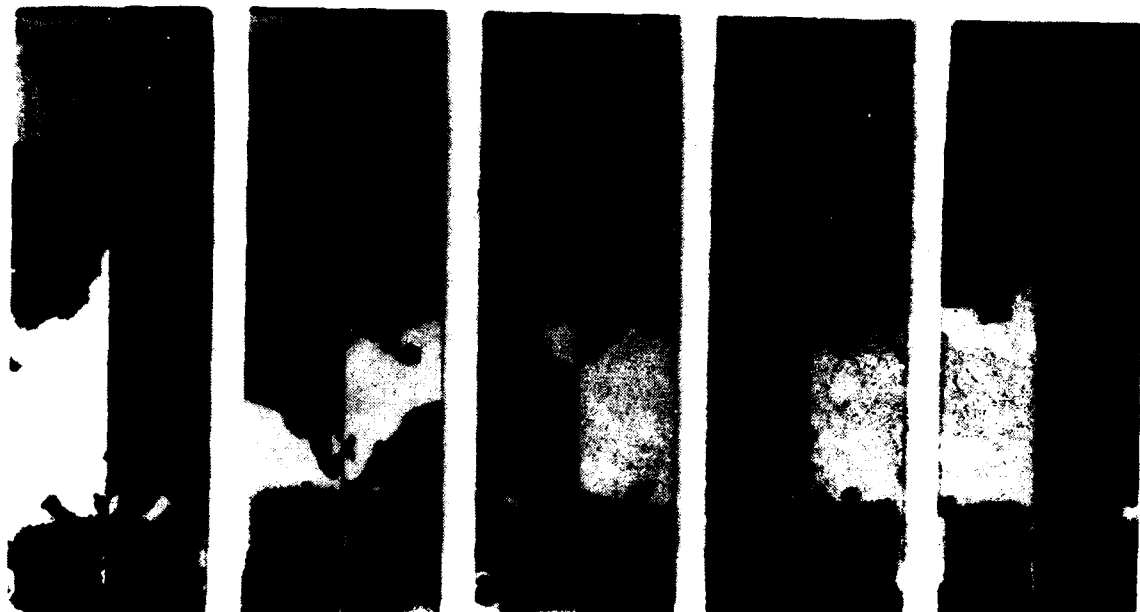
FIGURE 19. OPENED WEDGE SPECIMENS WITH PF-4 PHOSPHATE FLUORIDE PRETREATMENT AND BR127/FM300K ADHESIVE SYSTEM
