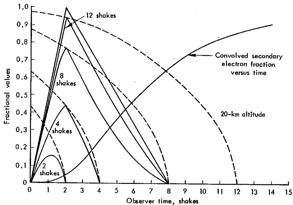
Fig. 19—Fraction of secondary electrons produced versus time for time-dependent \dot{\gamma} source (Fig. 10)
