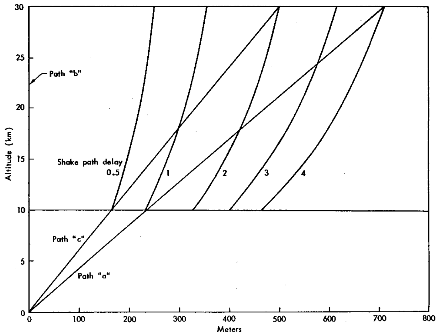
Fig. 17 — Illustrative path delay ellipsoids and geometry for absorption calculations
