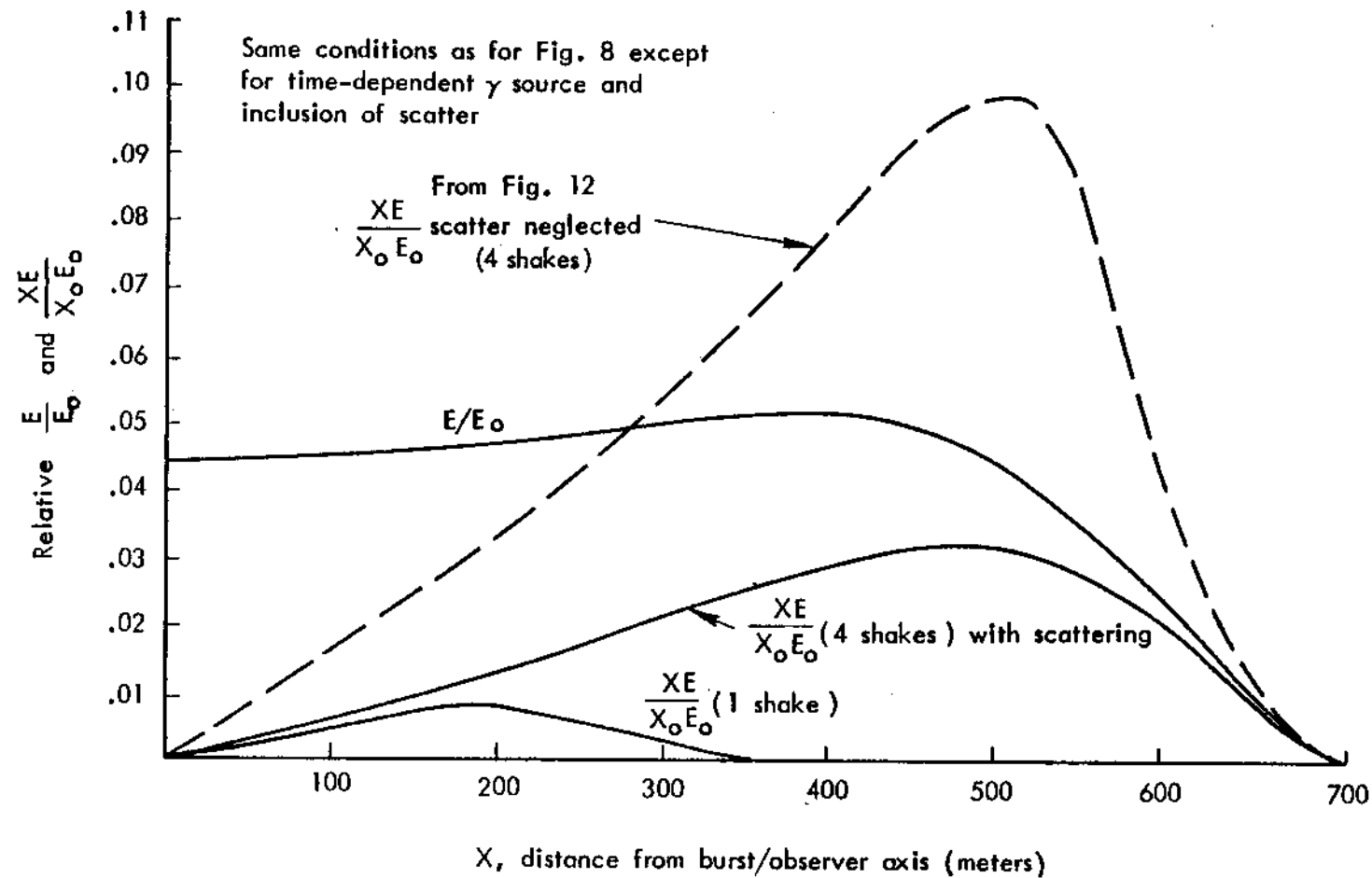
Fig. 16 — Radiation distribution at 1 and 4 shakes from electrons at 30-km altitude
