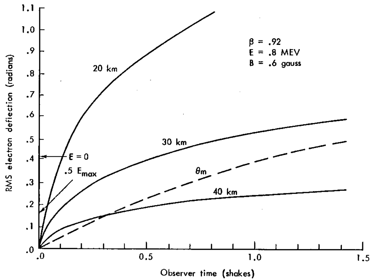
Fig. 13 — Electron deflection vs time due to scattering and to magnetic field
