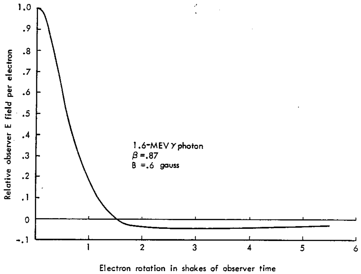
Fig. 7 — Lienard-Wiechert relative E field vs electron rotation time
