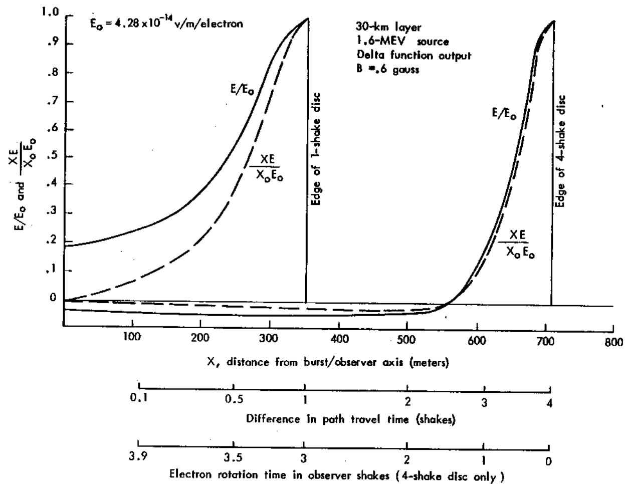
Fig. 8 - Radiation distribution at 1 and 4 shakes from electrons at 30 - km altitude
