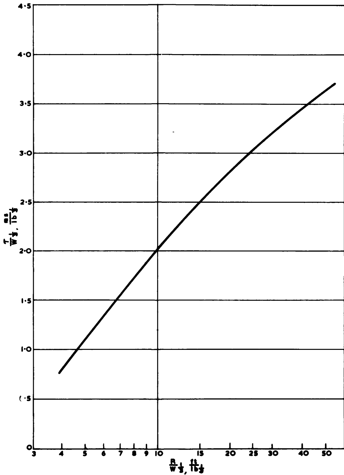
FIGURE 8(a) DURATION OF POSITIVE PHASE - DISTANCE FOR RDX/TNT 60/40
