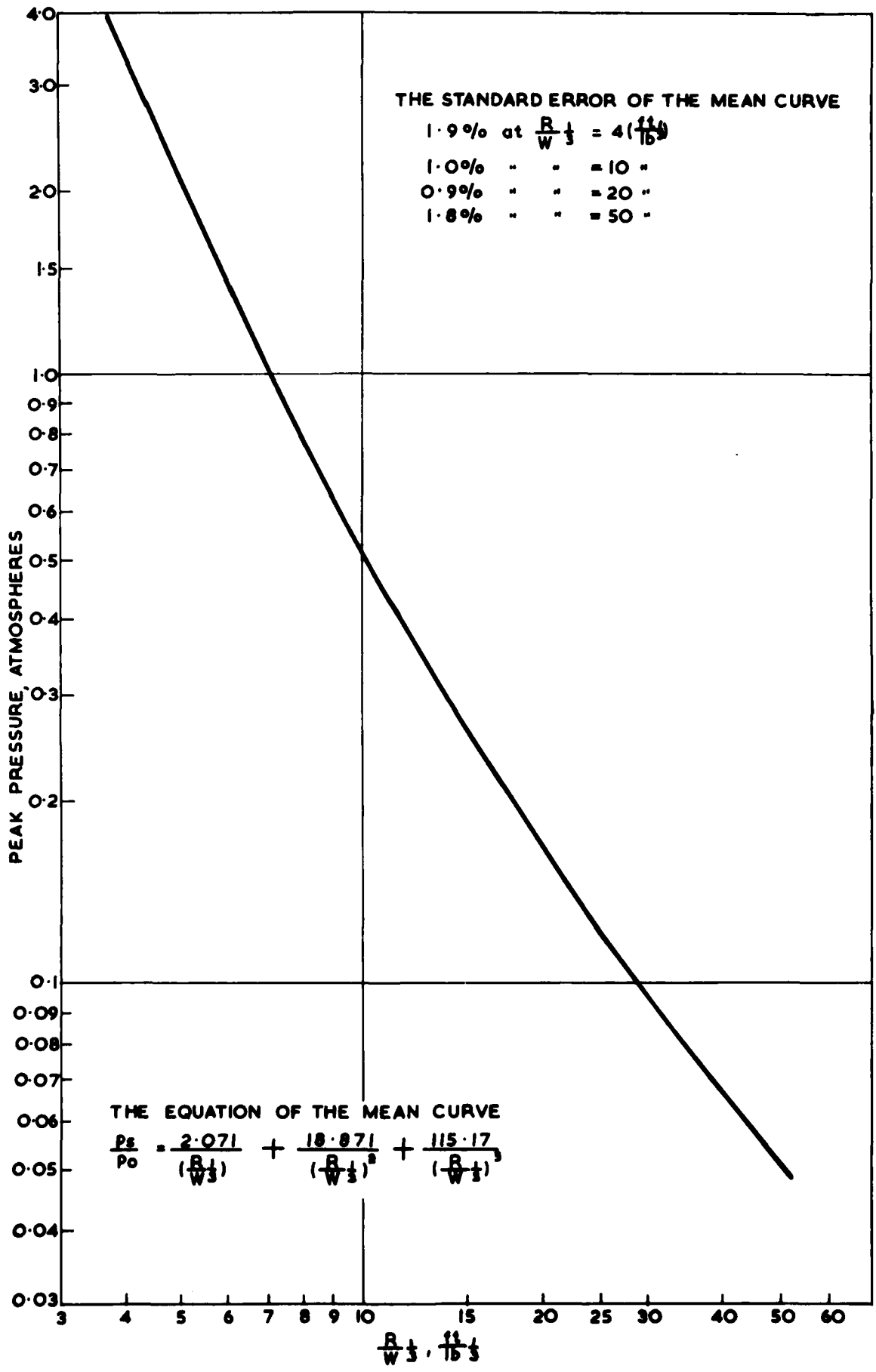
FIGURE 4 (d) PEAK PRESSURE - DISTANCE FOR RDX/TNT 60/40
