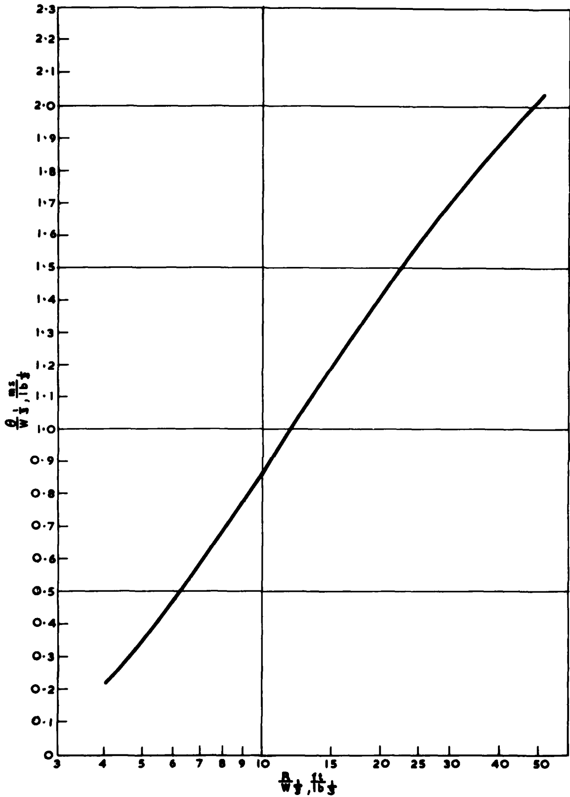
FIGURE 9(a) DECAY CONSTANT-DISTANCE, FOR RDX/TNT 60/40
