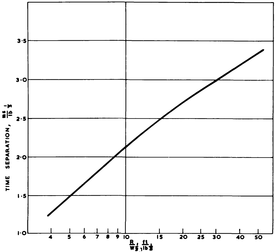
FIGURE II(a) TIME SEPARATION OF PRIMARY & SECONDARY SHOCKS FOR RDX/TNT
