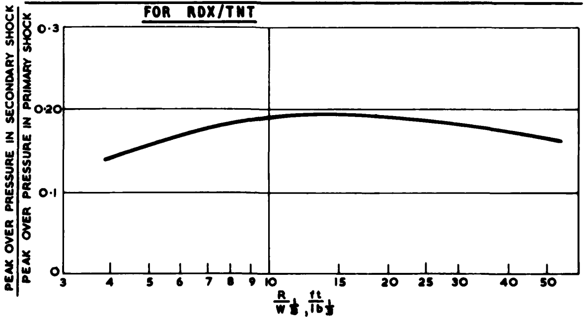
FIGURE II(b) RATIO OF PEAK OVER PRESSURES IN PRIMARY & SECONDARY SHOCKS FOR RDX/TNT
