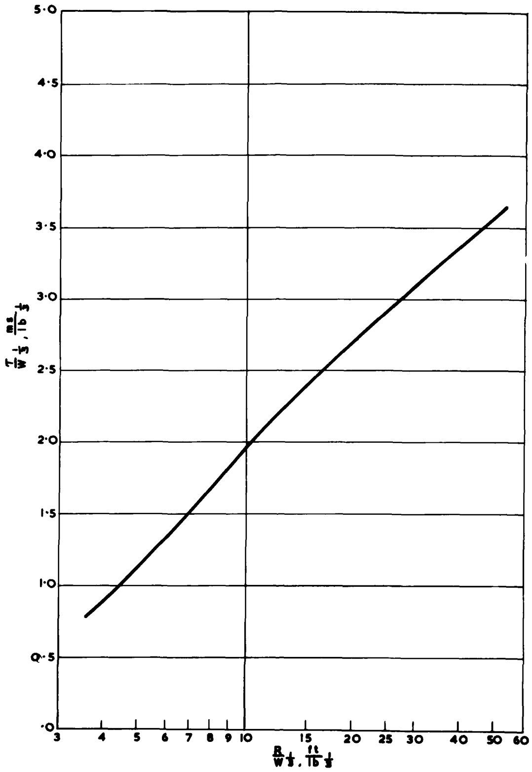
FIGURE 8 (b) DURATION OF POSITIVE PHASE - DISTANCE FOR TNT
