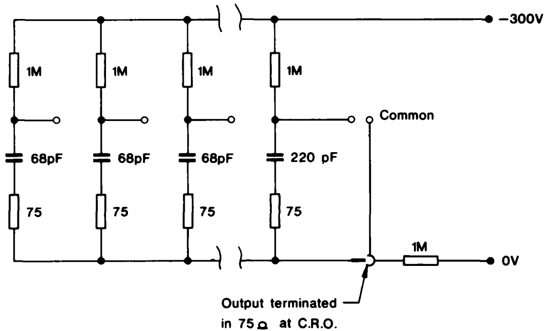
FIG. 5 - Event Pulse Circuit for Multilayer Board.
