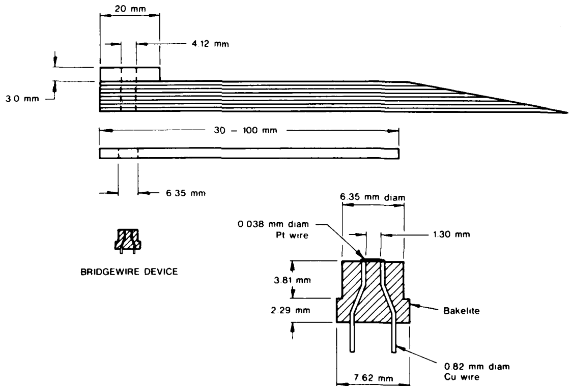
(b) For charges to be initiated by hot wire (electrical leads are not shown). The bridgewire device is shown enlarged in inset.
