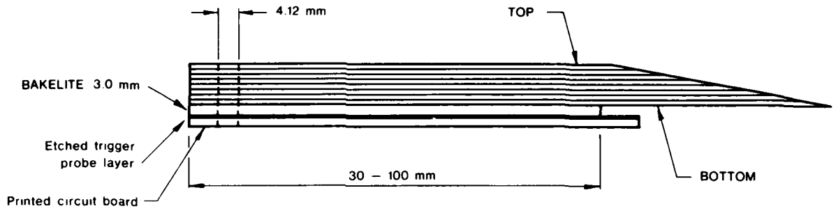
(a) For charges to be initiated by Lead Azide fusehead (electrical leads are not shown).
