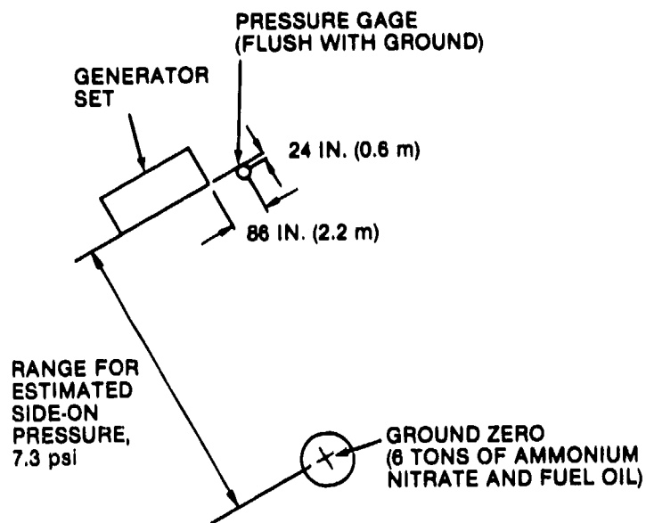
Figure 8. Sketch of airblast test setup for Hol-Gar model CE-301-AC/WK1 generator set.
