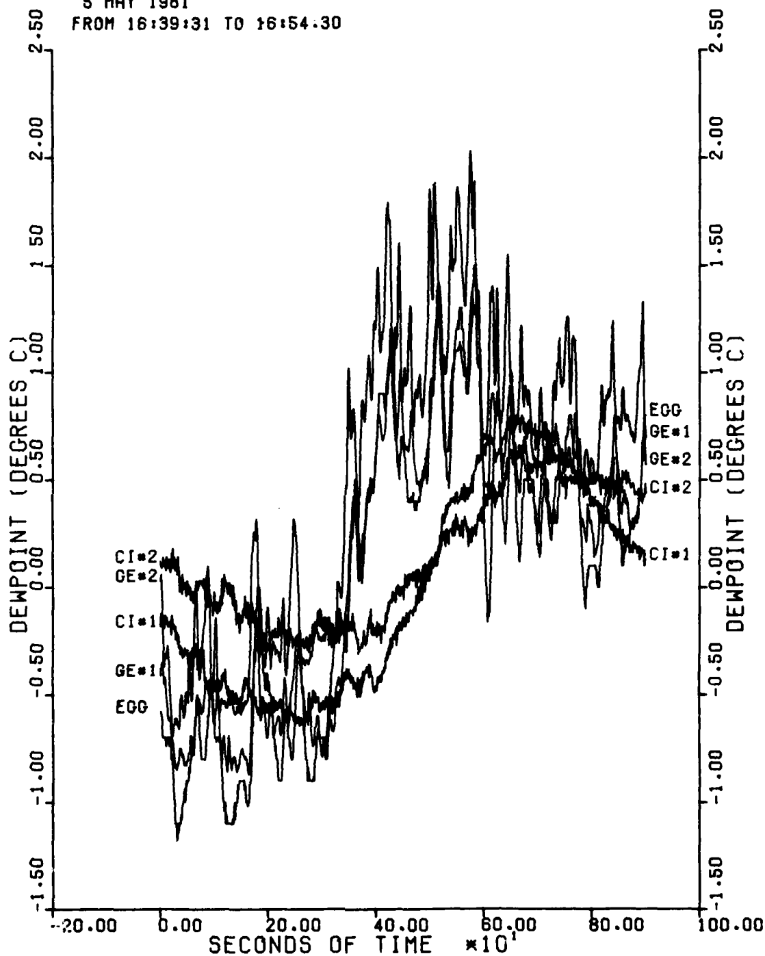
FIGURE 68. DEWPOINT VS TIME FOR SELECTED INSTRUMENTS.
