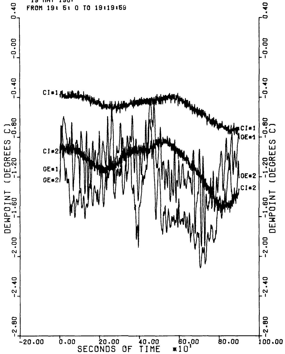
FIGURE C13. DEWPOINT VS TIME FOR SELECTED INSTRUMENTS.
