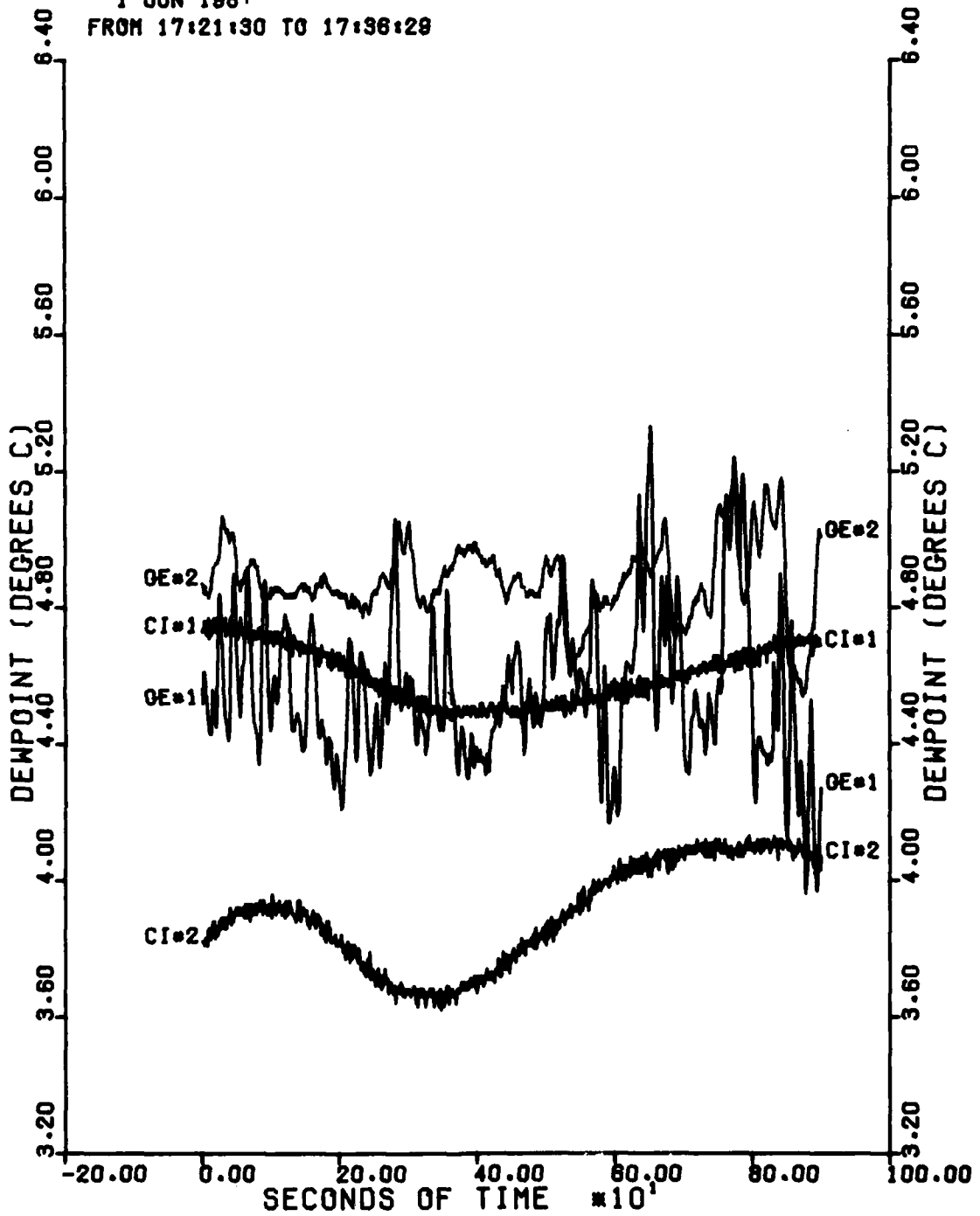
FIGURE C-21. DEWPOINT VS TIME FOR SELECTED INSTRUMENTS.
