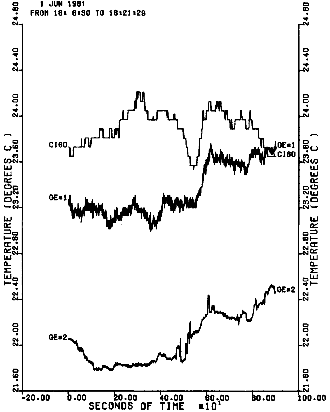
FIGURE C-20. TEMPERATURE VS TIME FOR SELECTED INSTRUMENTS.
