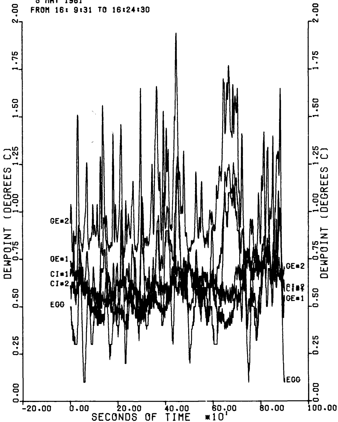
FIGURE 66. DEWPOINT VS TIME FOR SELECTED INSTRUMENTS.
