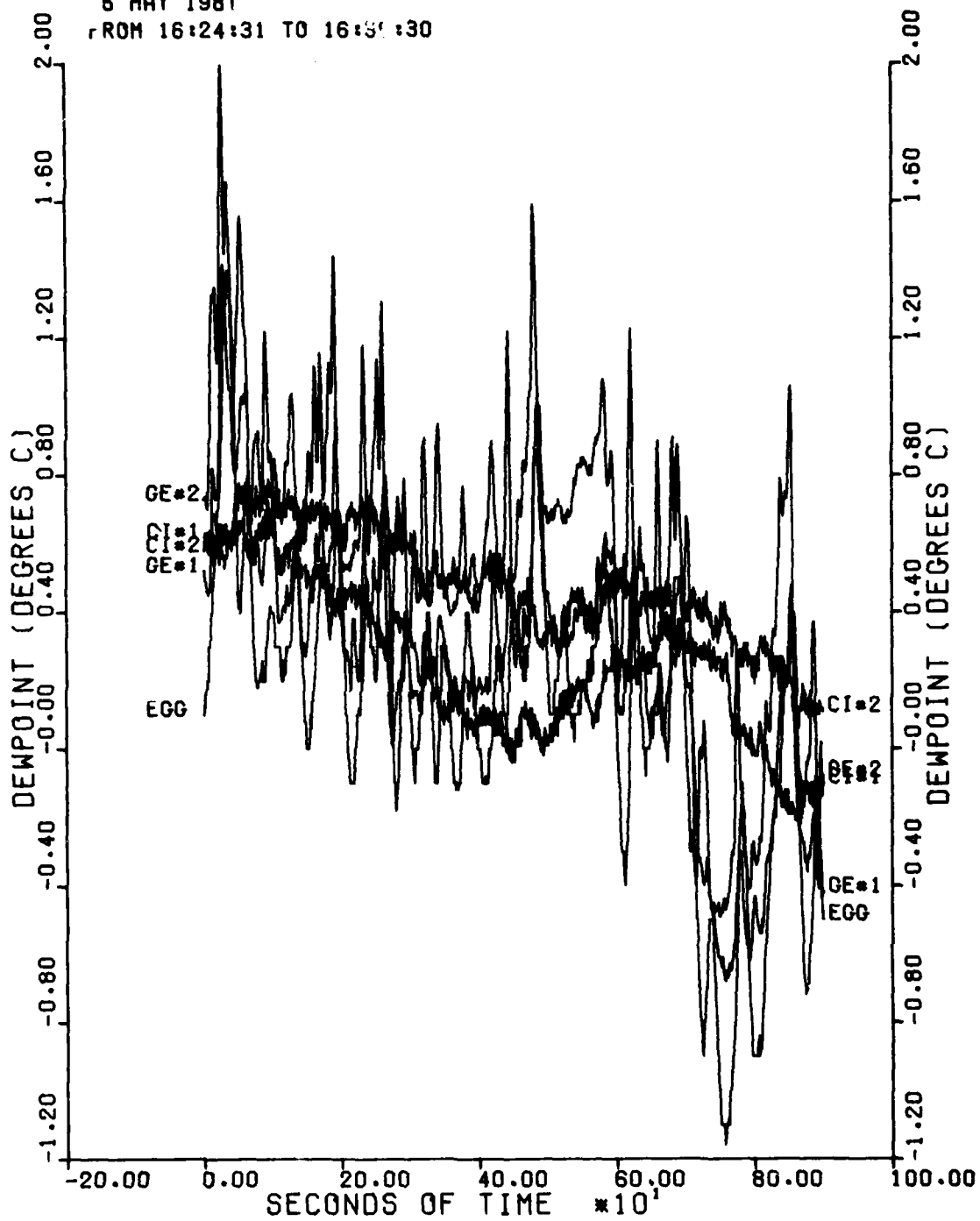
FIGURE 67. DEWPOINT VS TIME FOR SELECTED INSTRUMENTS.
