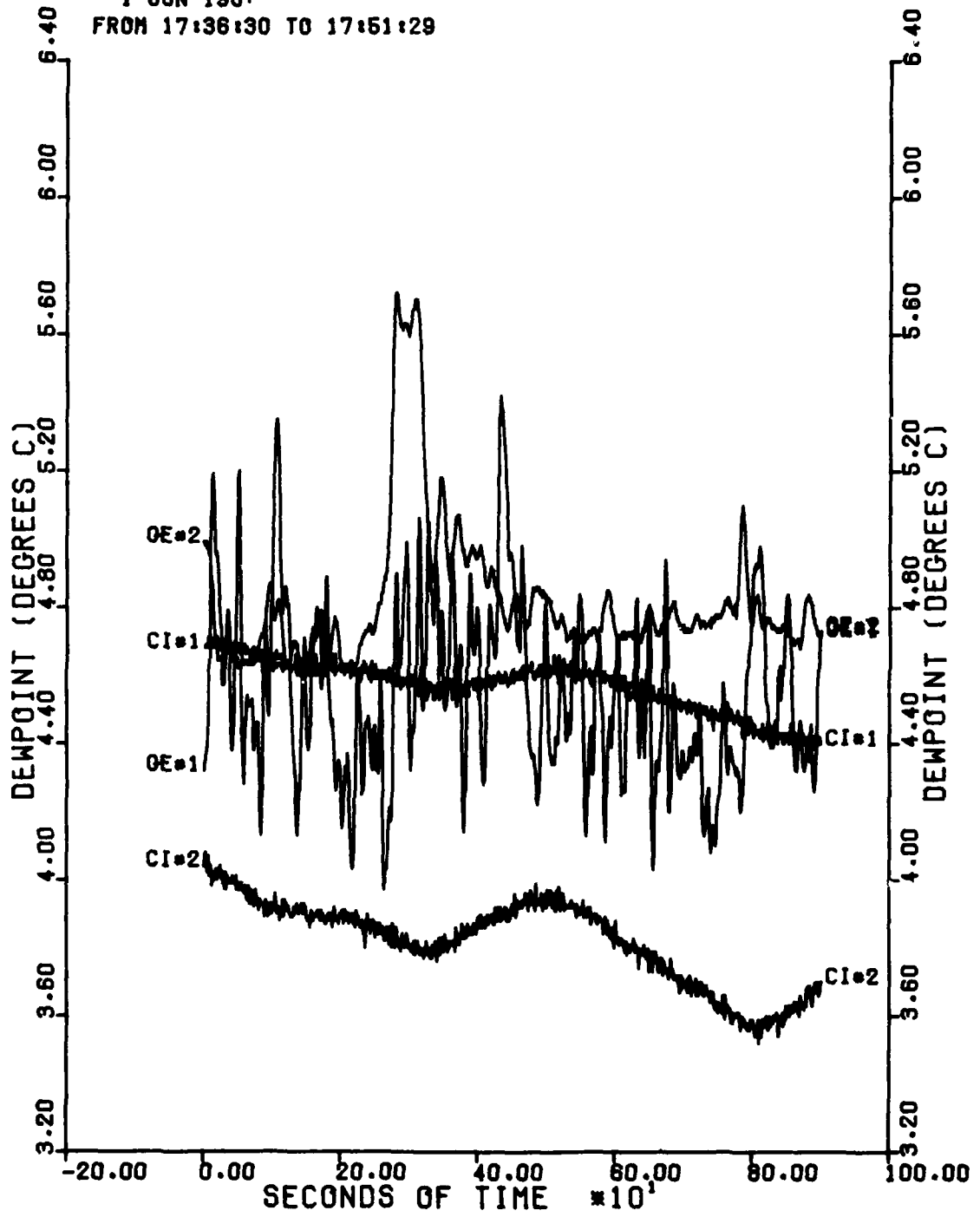
FIGURE 2. DEWPOINT VS TIME FOR SELECTED INSTRUMENTS.
