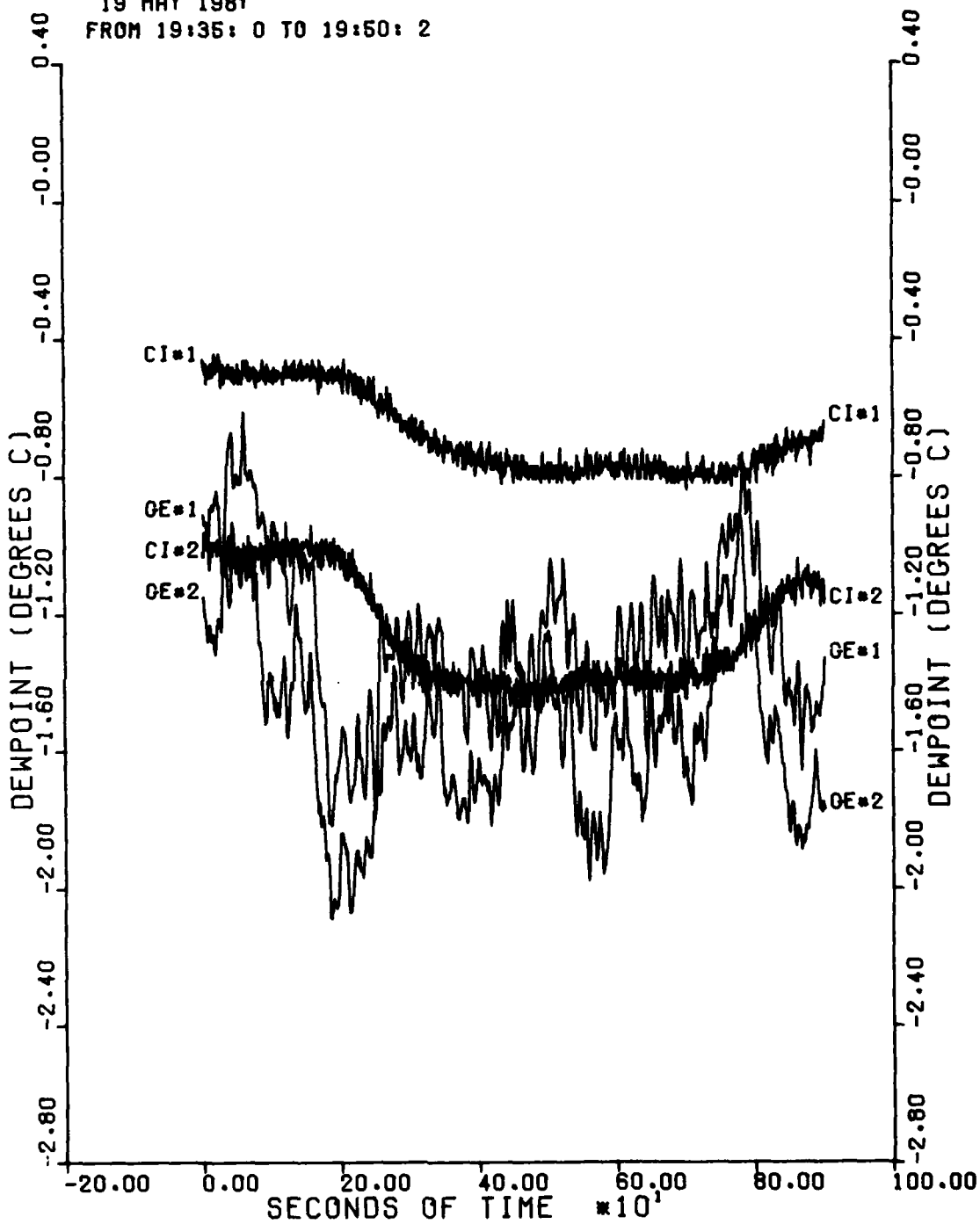
FIGURE 15. DEWPOINT VS TIME FOR SELECTED INSTRUMENTS.
