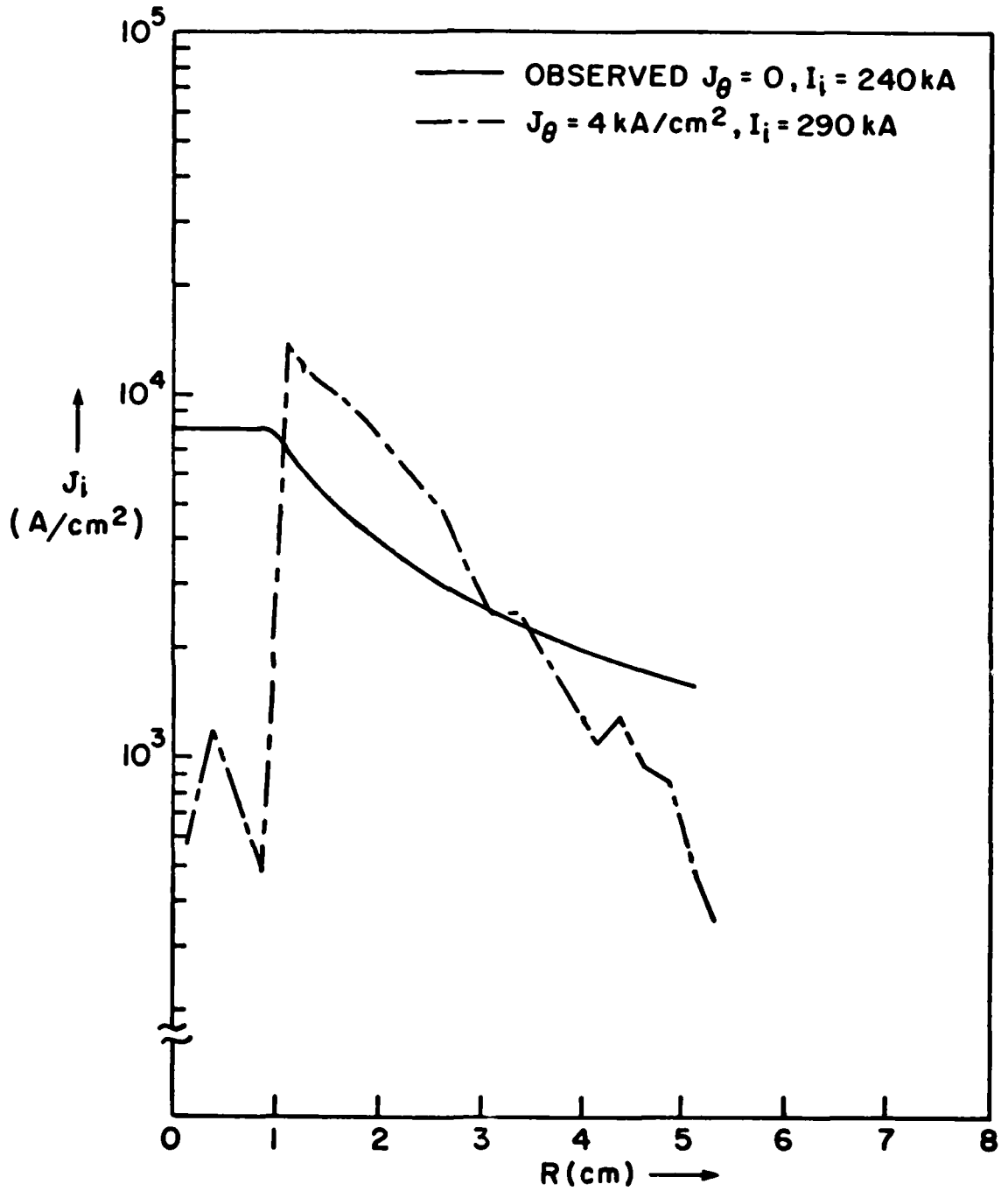
Fig. 18 - Radial profiles of PBFA-1 ion current density
