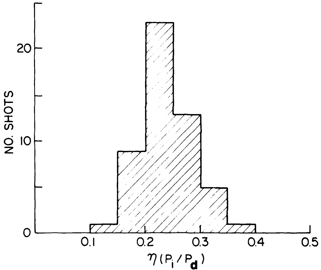
Fig. 13 — Statistical distribution of \eta , for the 4\Omega diode (courtesy of S. J. Stefanakis).
