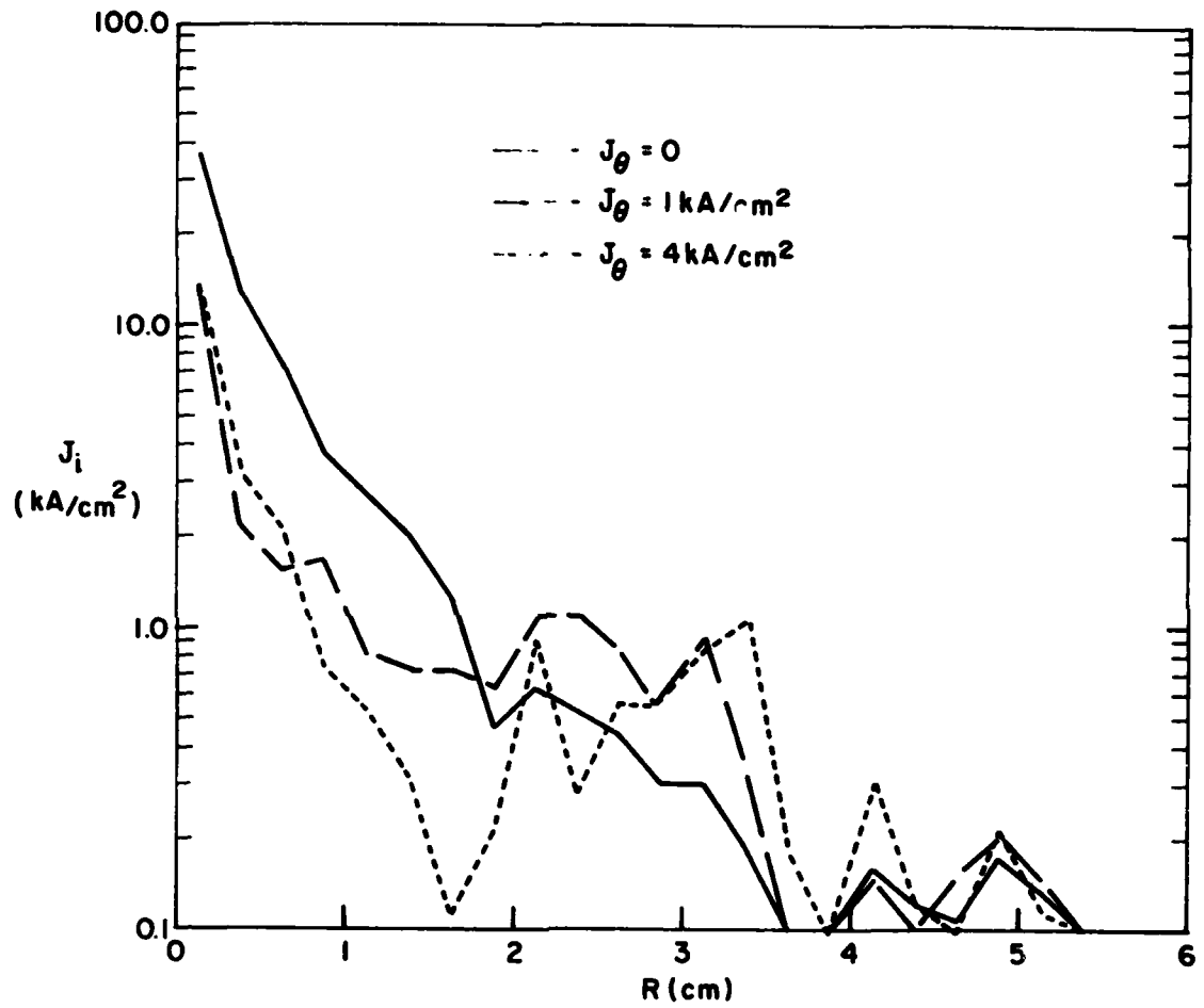
Fig. 11 - Radial profiles of AURORA ion current density collected at cathode
