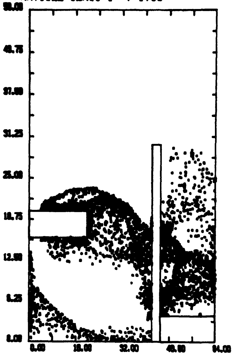
Fig. 7 - AURORA electrons-only flow for J_a = 1 \text{ kA/cm}^2
