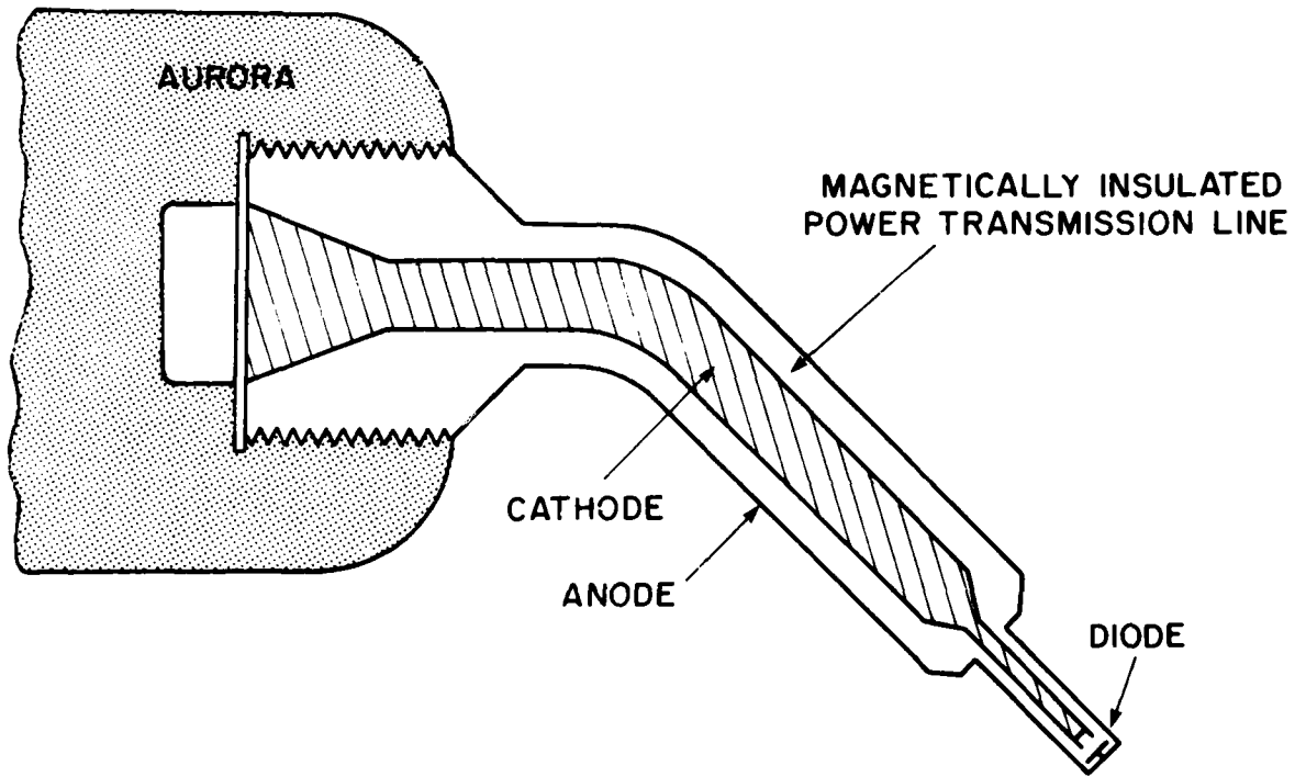
Fig. 3 — The NRL-AURORA ion diode experiment
