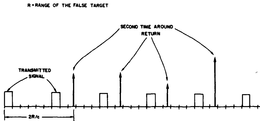
Fig. 1 - Second time around return
