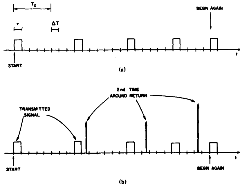
Fig. 2 (a) — Modulated PRI; n = 4 , \Delta T = \tau ; (b) sliding second time around return
