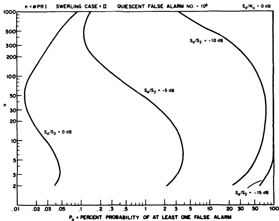
Fig. 11 — P_2 vs n with S_d/S_2 as a parameter
