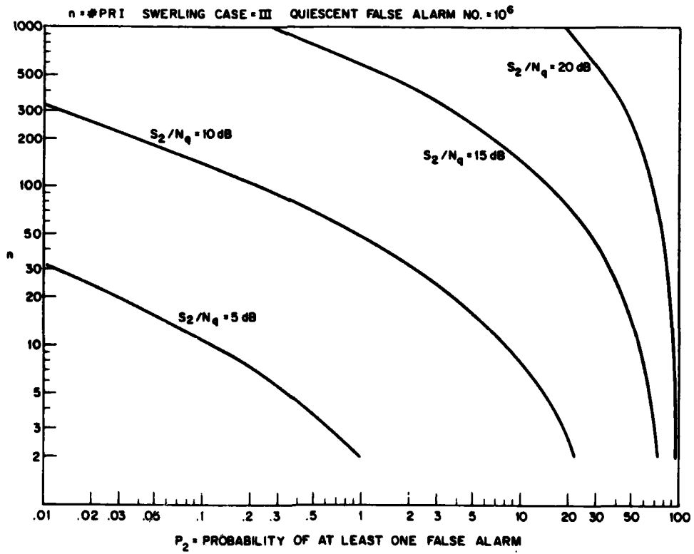
Fig. 7 - P_2 vs n , Swerling case III
