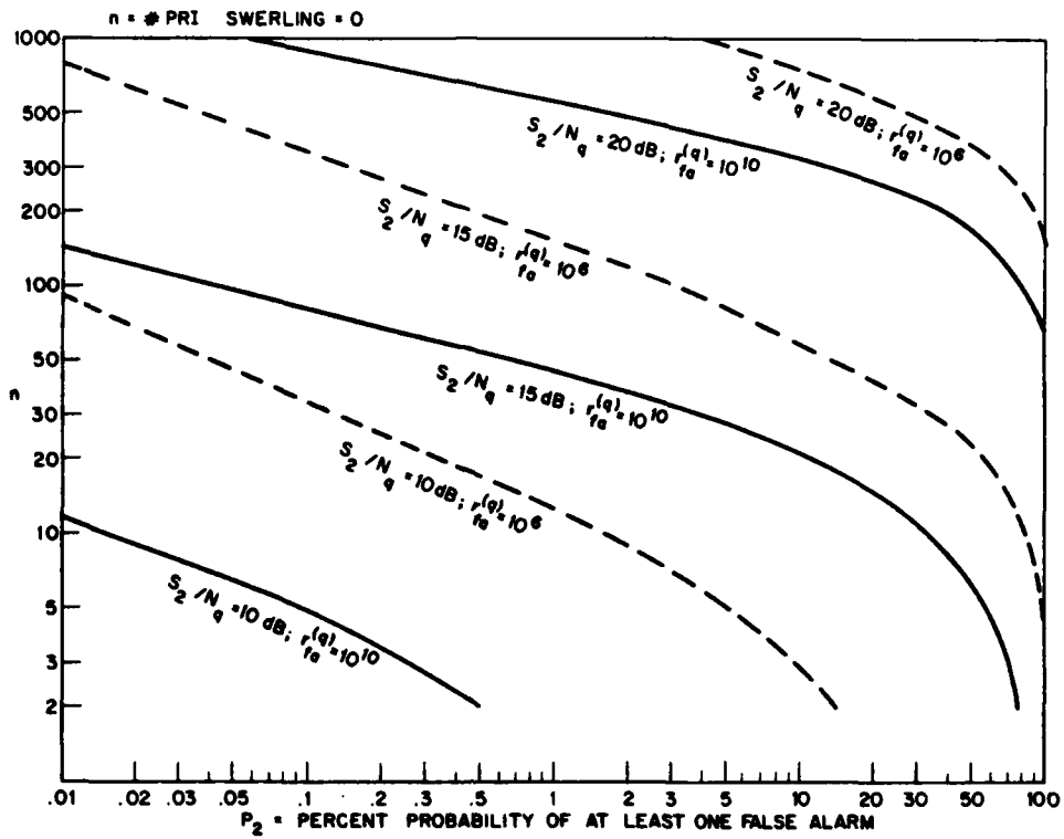
Fig. 4 - P_2 vs n , Swerling case 0
