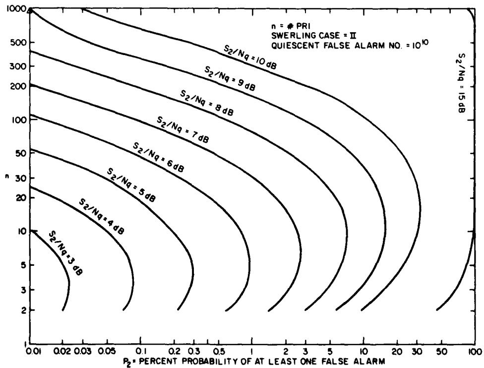
Fig. 9 — P_2 vs n , Swerling case II, r_p^{(q)} = 10^{10}
