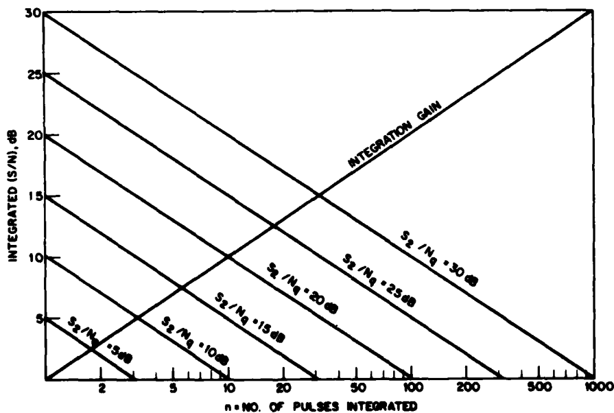
Fig. 3 - Integrated (S/N) vs no. of pulses with (S_2/N_q) as a parameter
