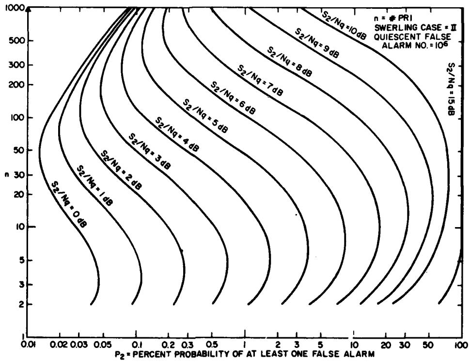
Fig. 6 - P_2 vs n , Swerling case II, r_{f0}^{(q)} = 10^6
