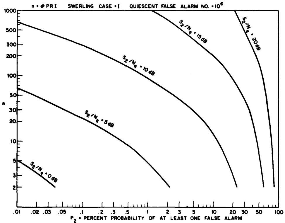
Fig. 5 - P_2 vs n , Swerling case I
