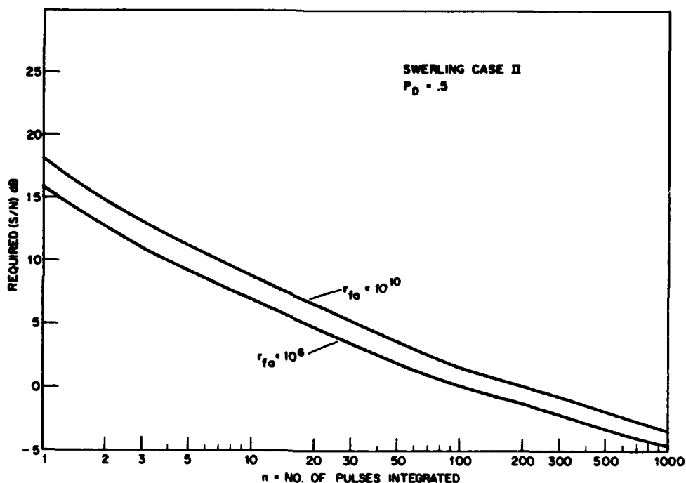
Fig. 10 - Required (S/N) vs n
