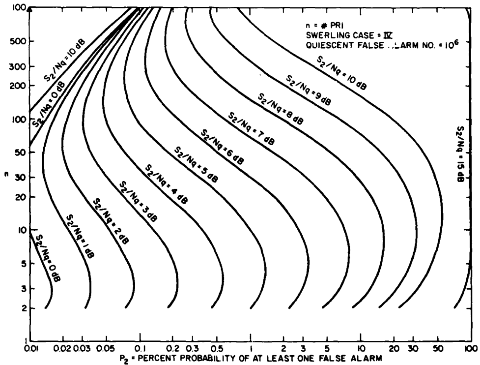
Fig. 8 — P_2 vs n , Swerling case IV
