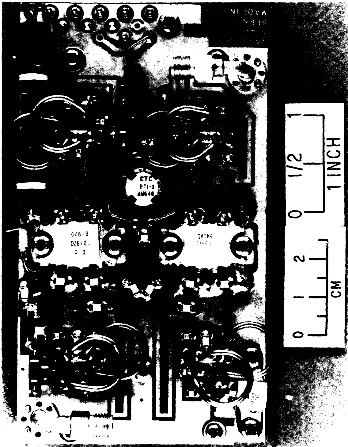
Figure 5. 120 Watt Module
