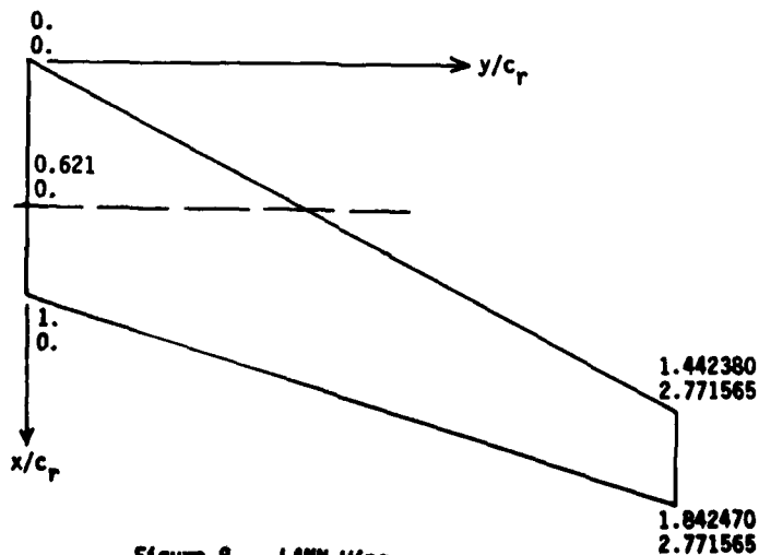
Figure 8.- LANN Wing.
