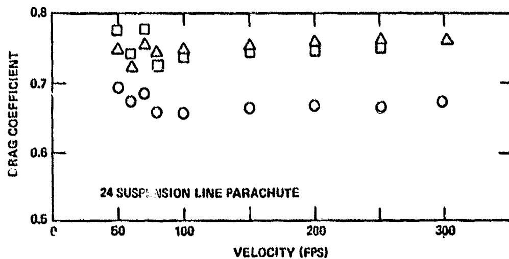
FIGURE 14 DRAG COEFFICIENT TEST DATA CANOPY CLOTH, MIL-C-7020, TYPE I PERMEABILITY = 88 CFM/FT 2
