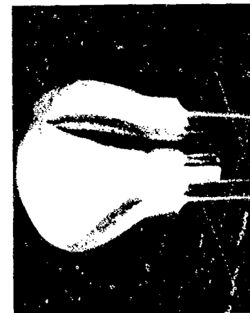
FIGURE 27 REEFED CANOPY INFLATED SHAPES; CLOTH PERMEABILITY = 98 CFM/FT 2 ; 16 SUSPENSION LINE PARACHUTE; SUSPENSION LINE LENGTH = 1.4 L; TEST VELOCITY = 293 FPS
