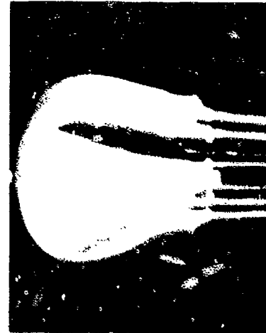
FIGURE 32 REEFED CANOPY INFLATED SHAPES; CLOTH PERMEABILITY = 225 CFM/FT 2 ; 12 SUSPENSION LINE PARACHUTE; SUSPENSION LINE LENGTH = 1.0 L; TEST VELOCITY = 293 FPS
