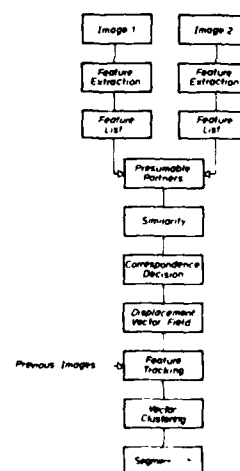
Fig. 23: Flow chart of the algorithm
