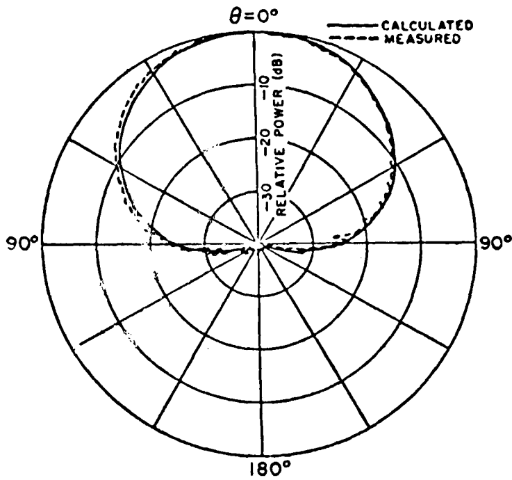
Figure 5c. Roll plane pattern ( E_\theta ) for a KA-band circular waveguide forward of the wings.
