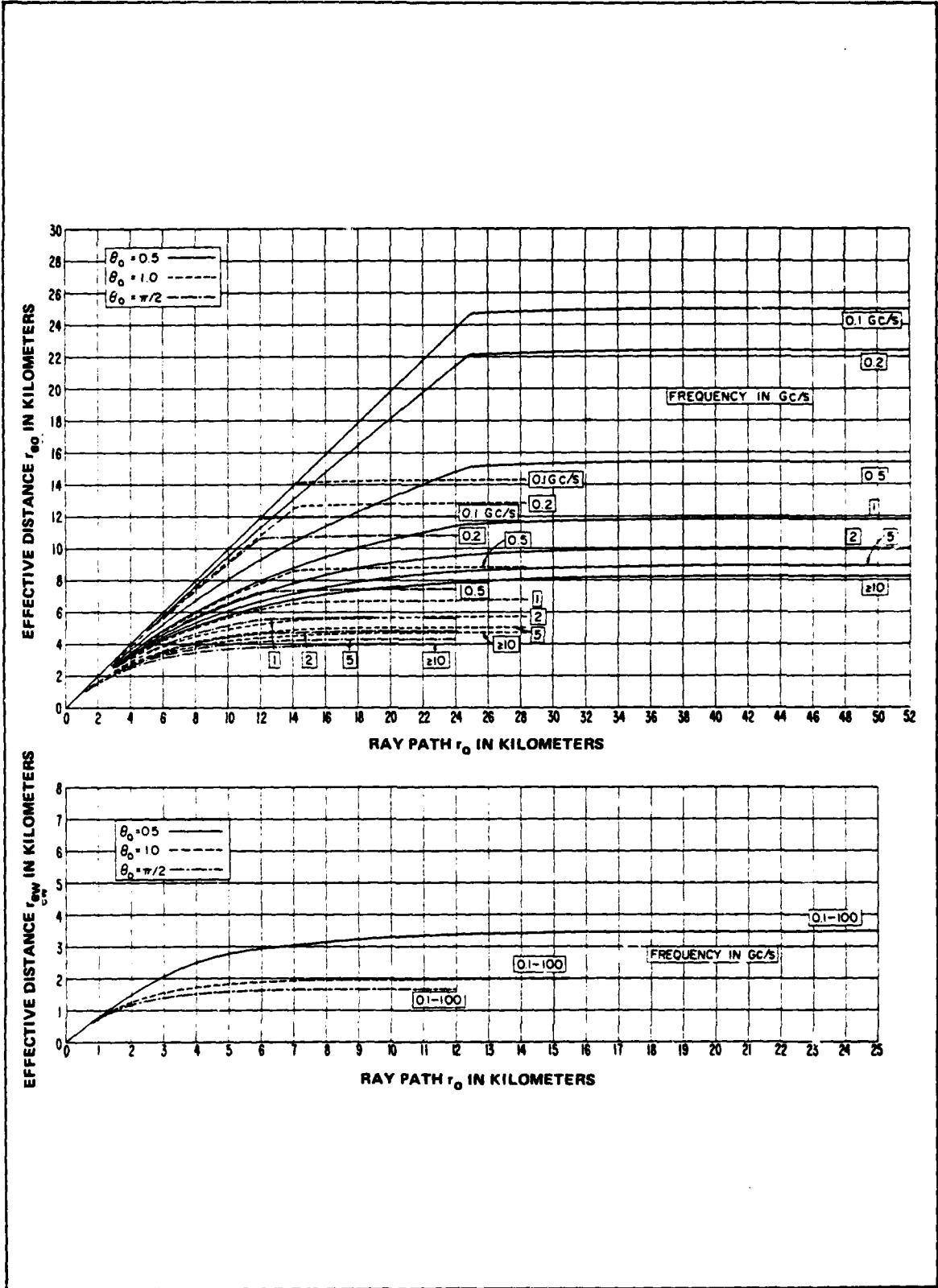
Figure 1-15. Effective distances r_{eo} and r_{ew} for absorption by oxygen and water vapor, \theta_o = 0.5, 1, \pi/2 .
