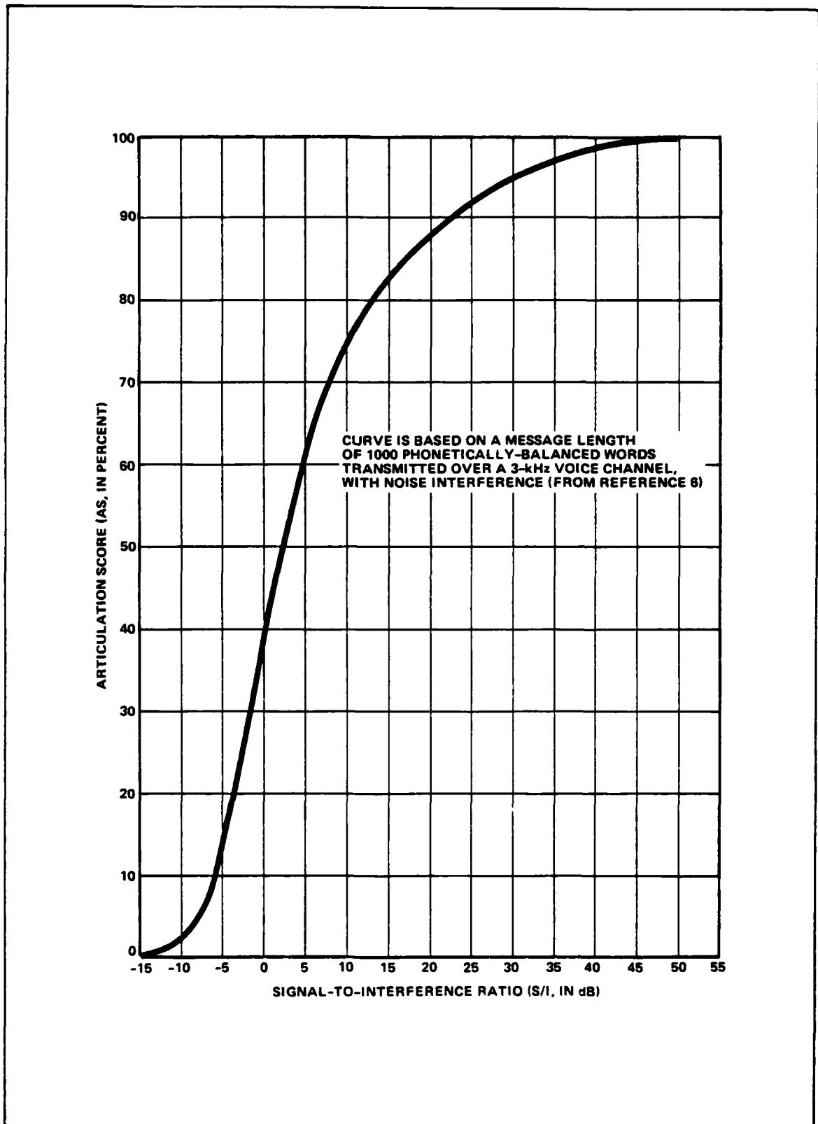
Figure 2-1. Articulation score versus noise interference.
