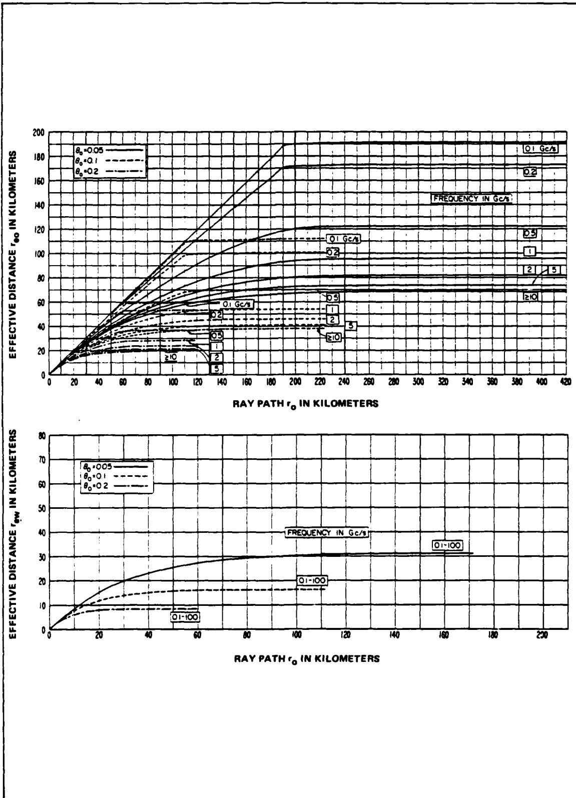
Figure 1-14. Effective distances r_{eo} and r_{ew} for absorption by oxygen and water vapor, \beta_o = 0.05, 0.1, 0.2 .
