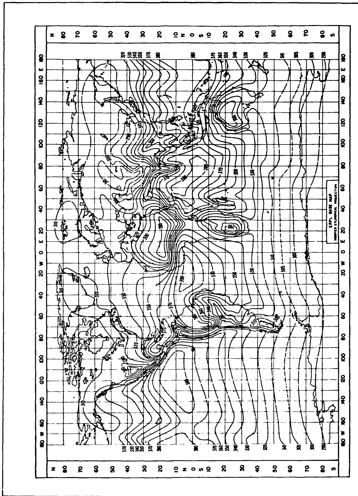
Figure 1-3. Minimum monthly surface refractivity values referred to mean sea level.
