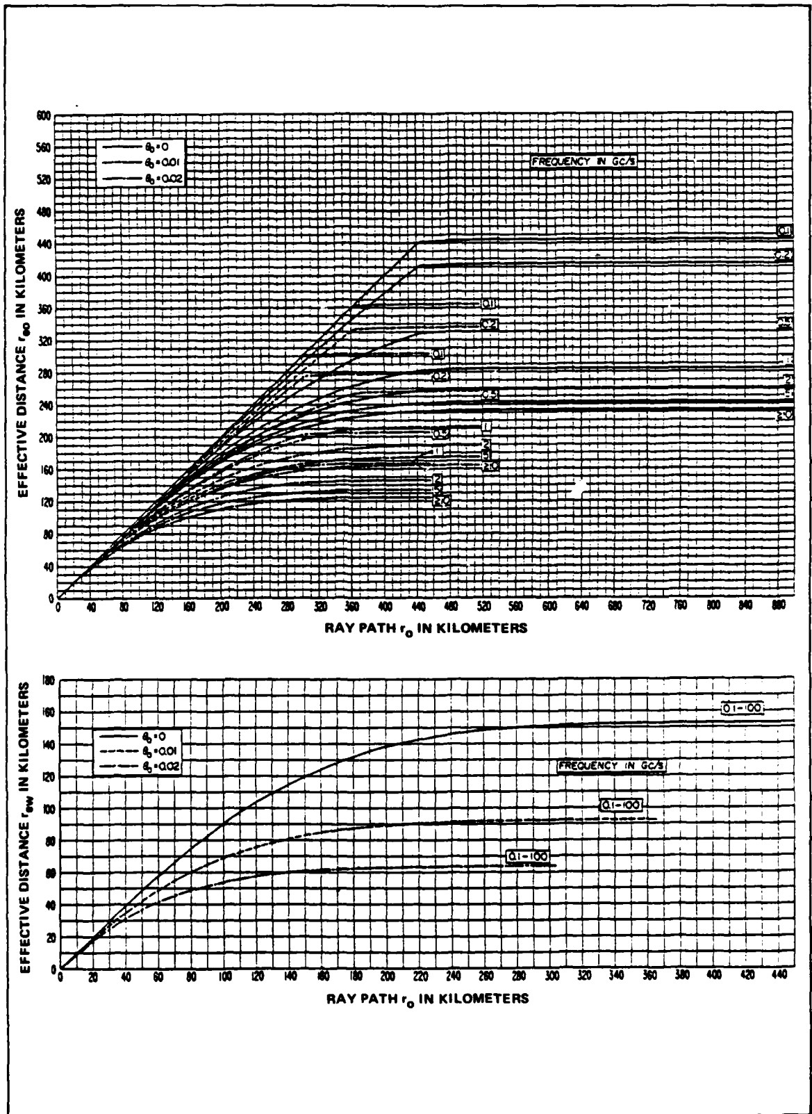
Figure 1-13. Effective distances r_{eo} and r_{ew} for absorption by oxygen and water vapor, \theta_o = 0, 0.01, 0.02 .
