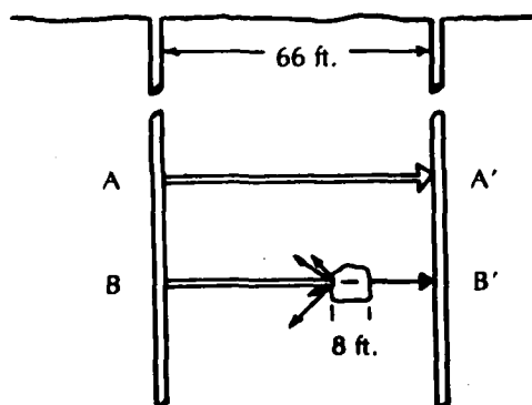
Figure 2. Signal Delay Caused by Tunnel. This example shows the degree of signal delay which can be caused by a typical tunnel. The delay-deviation from normal depends on the ratio of tunnel size to hole spacing, and the ratio of normal rock sonic velocity to the sonic velocity in air (or water if the tunnel is water-filled).
