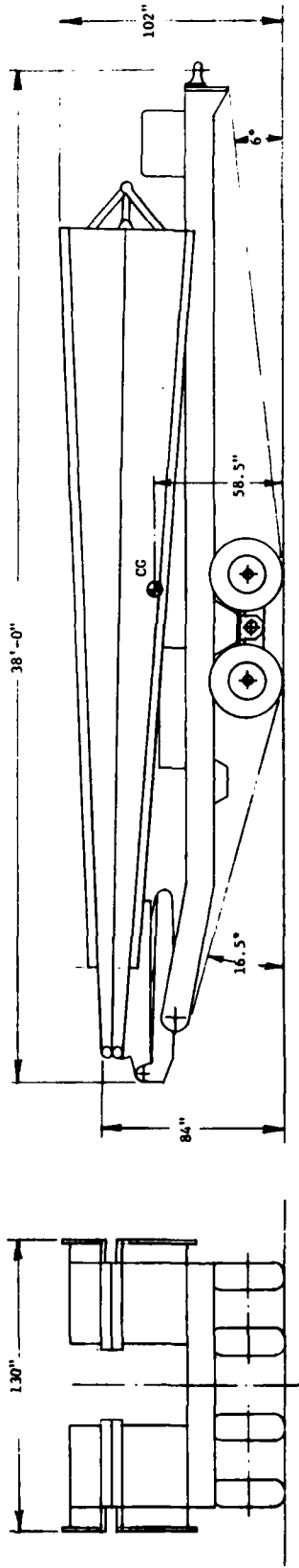
Ground Transport Configuration
