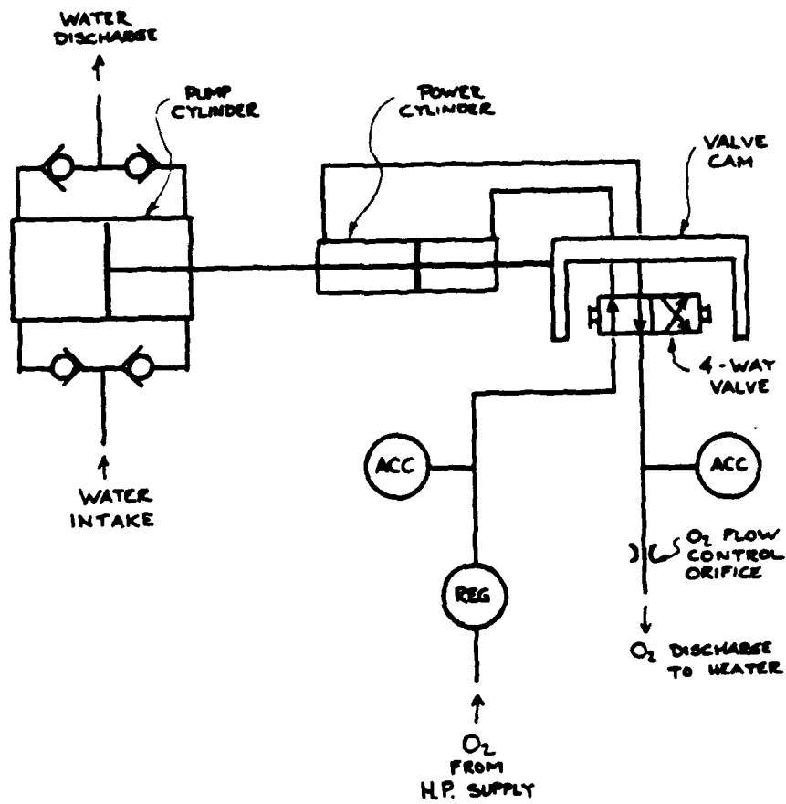
FIGURE 17. WATER PUMP SCHEMATIC
