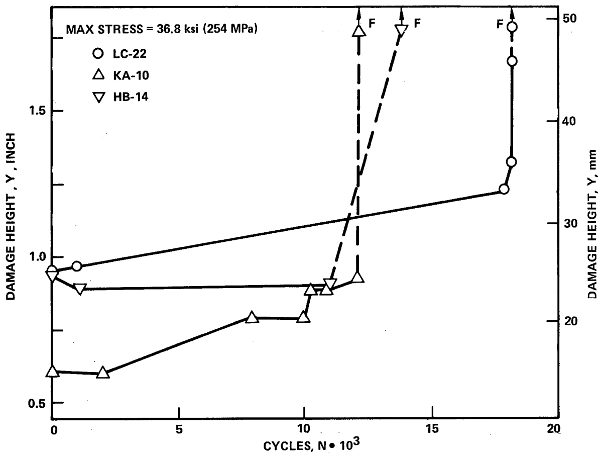
Figure 81a & b. Damage Growth Behavior of Impact Damaged 24-Ply 67% 0° Fiber T300/5208 Laminate Specimen, R = -1 \sigma_{\max} = 36.8 ksi (254 MPa)
