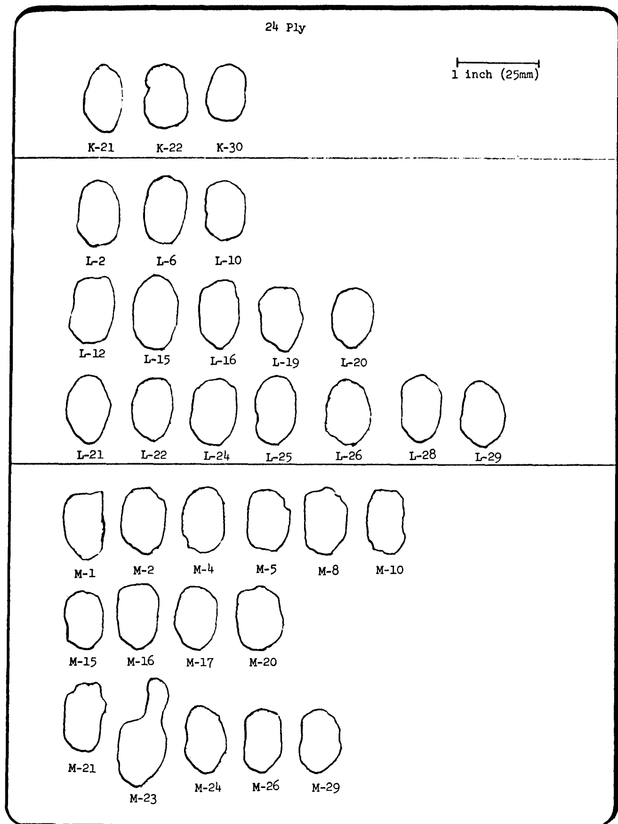
Figure 1b. Initial Impact Damage Dimensions for 67% 0° Fiber 24-Ply Laminate Specimens
