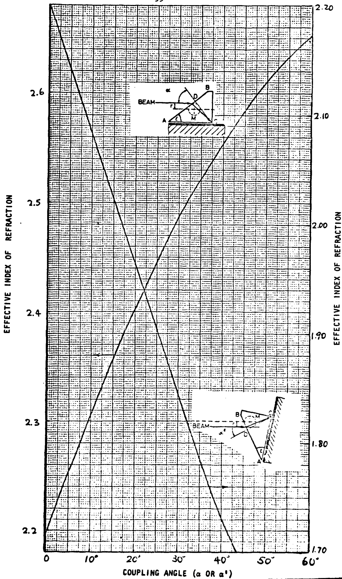
Figure 4 Effective refractive index vs coupling angle for a rutile prism.
