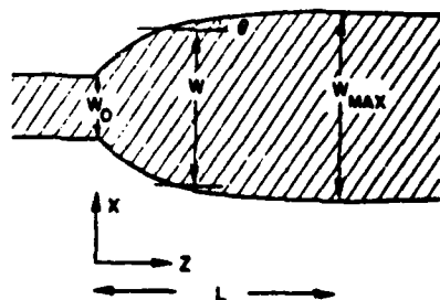
Figure 7 Top view of a parabolic waveguide horn (after Burns, et. al.)
