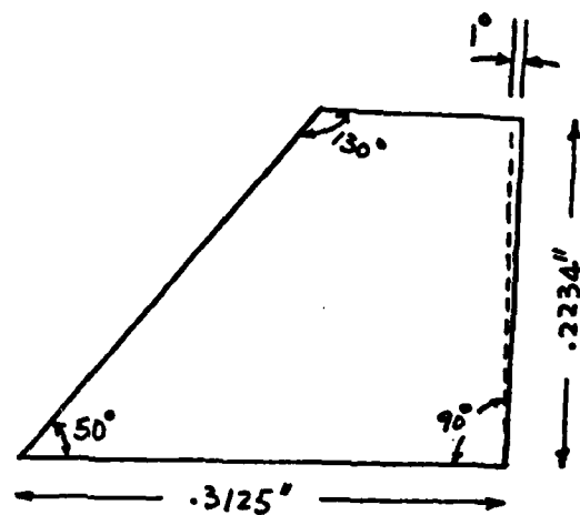
Figure 5 A possible design for a prism.
