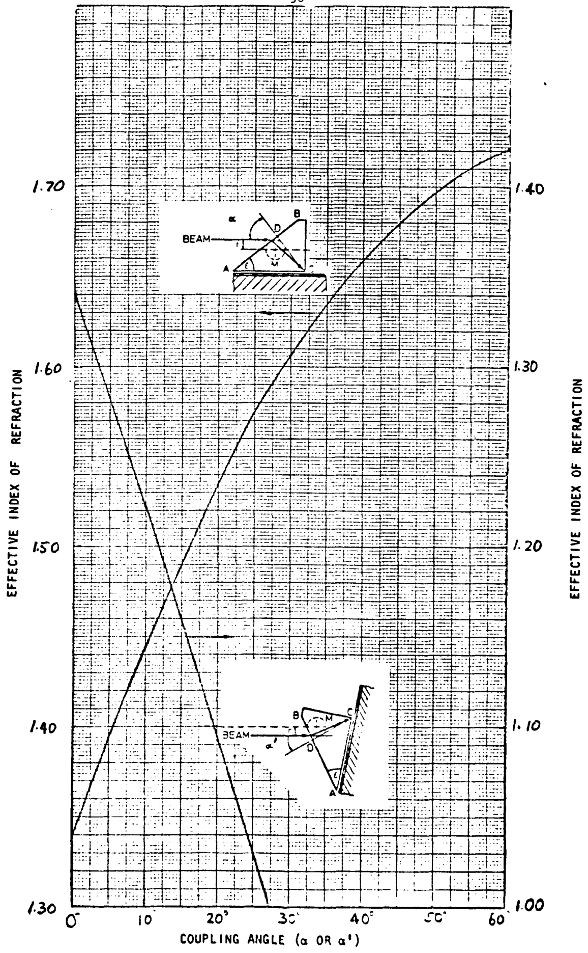
Figure 3 Effective refractive index vs coupling angle for a flint glass prism.
