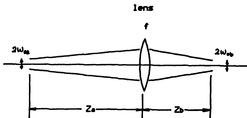
Figure 6 Transformation of Gaussian beam by a lens
