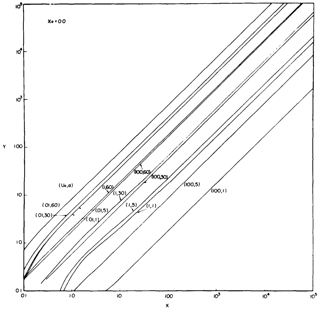
Figure 2. Typical Trajectories for y_0 = 0 , x_0 = 0.0 . The numbers in parenthesis are emission energy, U_0 , and emission angle, \alpha
