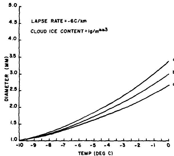
(a) Cloud Ice Content is 1.0 \text{ g/mm}^3
