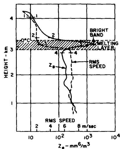
Figure B1. Profile of Radar Reflectivity vs Height. Note that maximum radar reflectivity is found below the 0°C-isotherm (after Lhermitte and Atlas, 1963 B6 )
