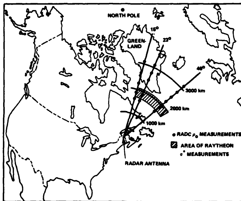
Figure 1. Coverage of the Polar Fox II Radar
