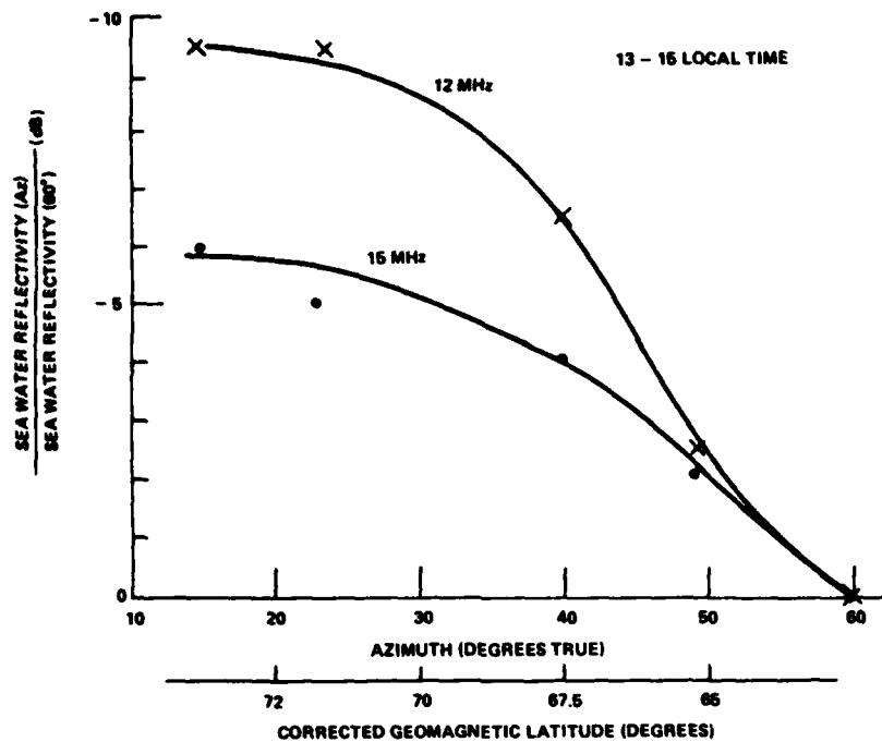
Figure 4. Azimuthal Dependence of Sea Water Reflectivity
