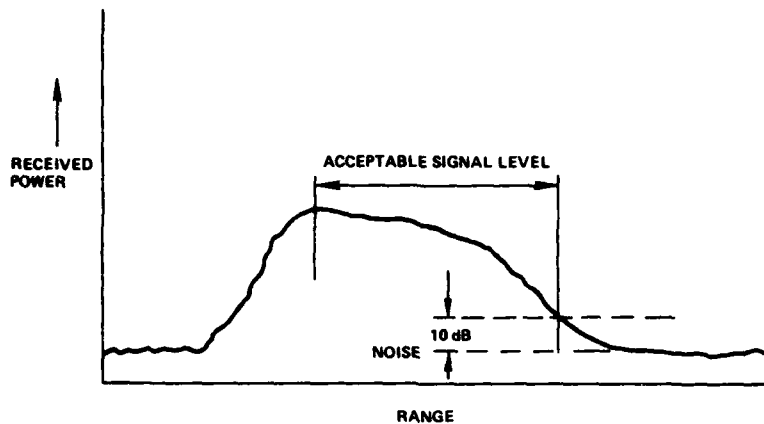
Figure 3. Typical Ground Clutter Signal
