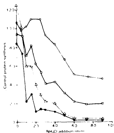
Fig. 7. Effect of time of \text{NH}_4\text{Cl} addition on diphtheria toxin-induced inhibition of protein synthesis. Toxin conc.: \circ , 0.001; \square , 0.01; \triangle , 0.1; \bullet , 0.5 \mu\text{g/ml} .
