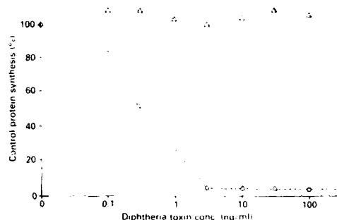
Fig. 1. Effect of NH 4 Cl on diphtheria toxin-induced inhibition of protein synthesis. ○, Control; △, NH 4 Cl, 10 mM.
