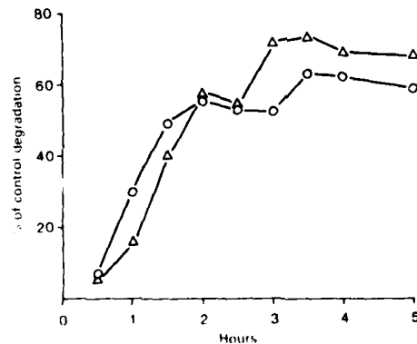
Fig. 5. Effect of \text{NH}_4\text{Cl} on the degradation of diphtheria toxin. \Delta , Control; \circ , \text{NH}_4\text{Cl} , 10 mM.
