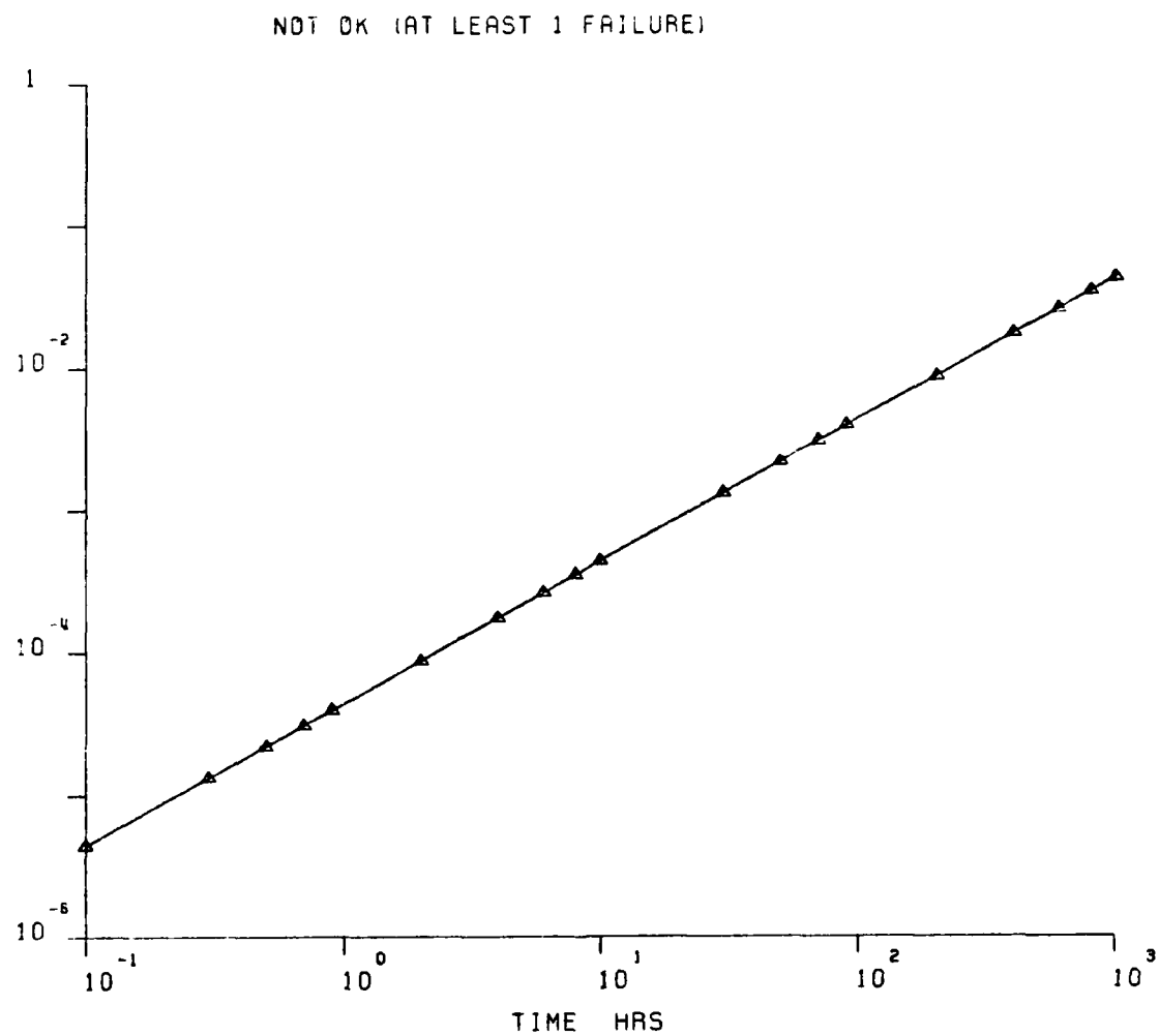
Figure A-17. Markov Model of an Example Engine Controller (2 of 7)
