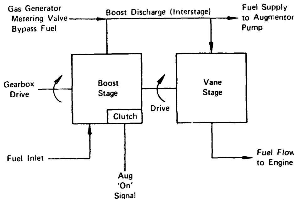
Figure 22. Main Fuel Pump Functional Block Diagram
