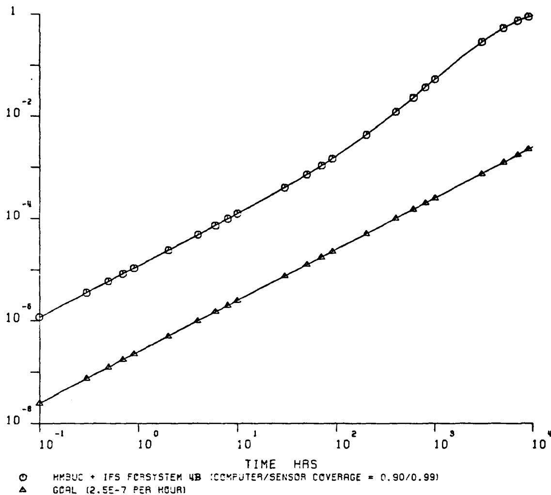
Figure 54. HMBUC and IFS for System 4A (Comp/Sensor Coverage = 0.90/0.99)
