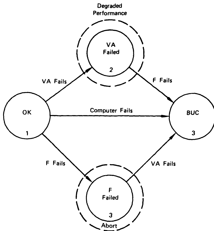
Figure A-15. Computer and Actuator Failure Model
