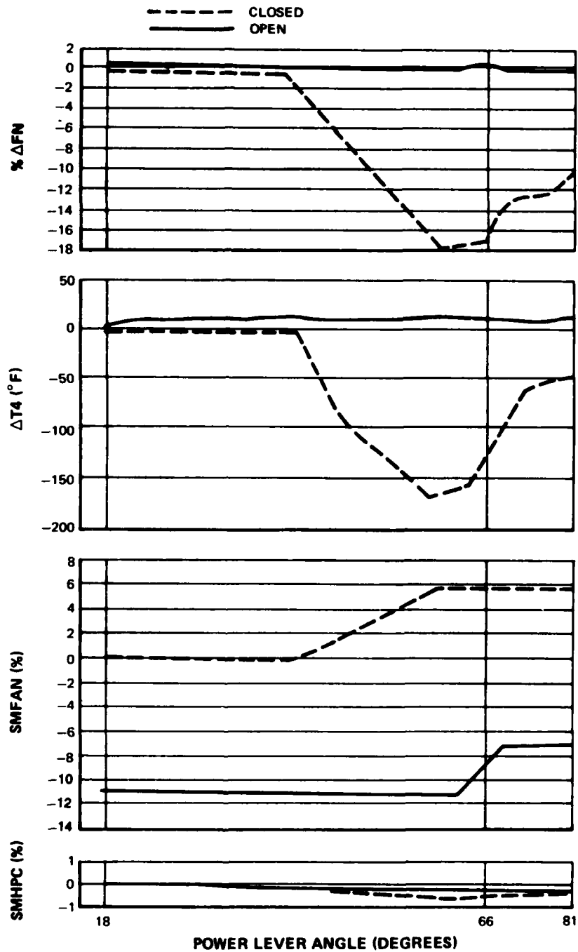
Figure 28. Fan Inlet Guide Vane Angle (FIGV) Failure Effects at Sea Level Static Conditions
