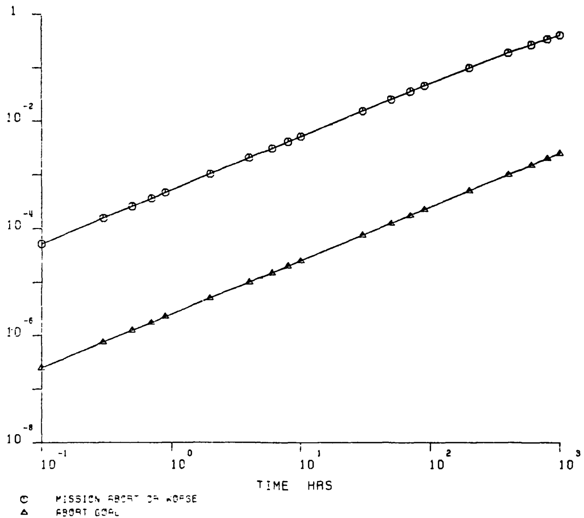
Figure 40. FAFTEEC Baseline Reliability Evaluation: Simplex System (Mission Abort)
