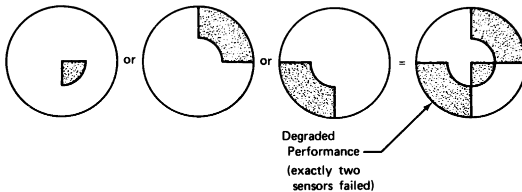
Figure A-12. The Resultant Union of the Three Sets Represented by Venn Diagrams
