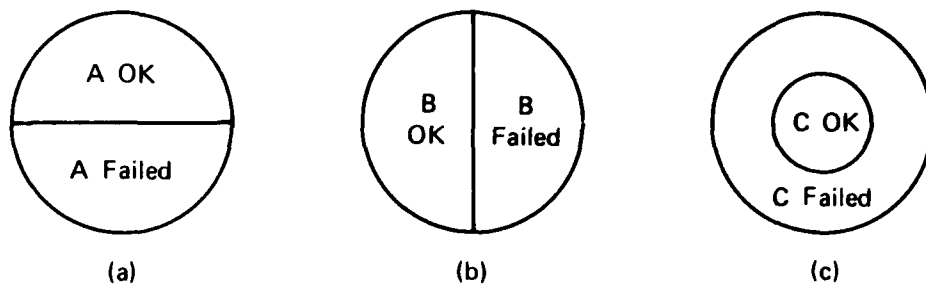
Figure A-8. Venn Diagram Representation of Partitional Example (Figure A-7)
