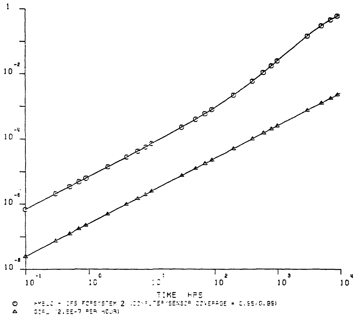
Figure 48. HMBUC and IFS System 2 (Comp/Sensor Coverage = 0.95/0.99)
