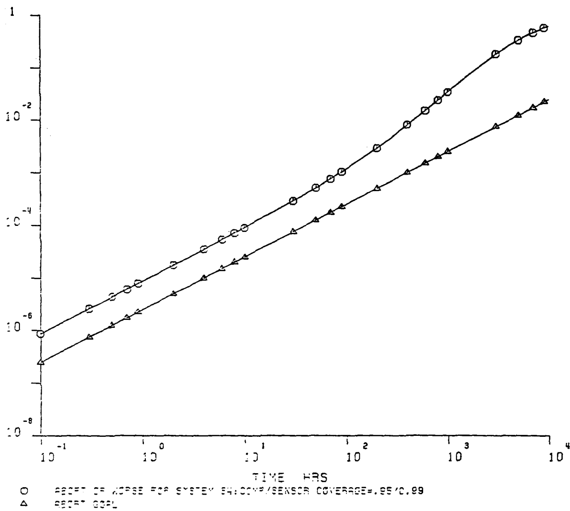
Figure 49. Abort Model for System 3 (Comp/Sensor Coverage = 0.95/0.99)
