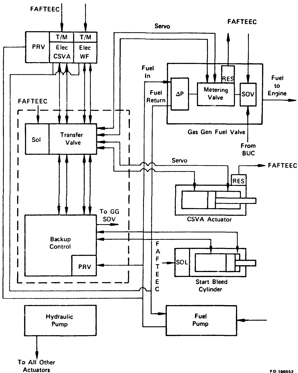
Figure 19. FAFTEEC Backup Control Implementation
