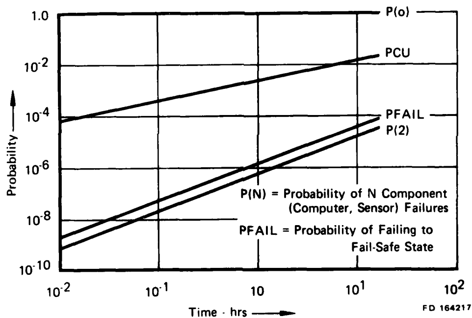
Figure A-4. Reliability Model Results for Sample Case
