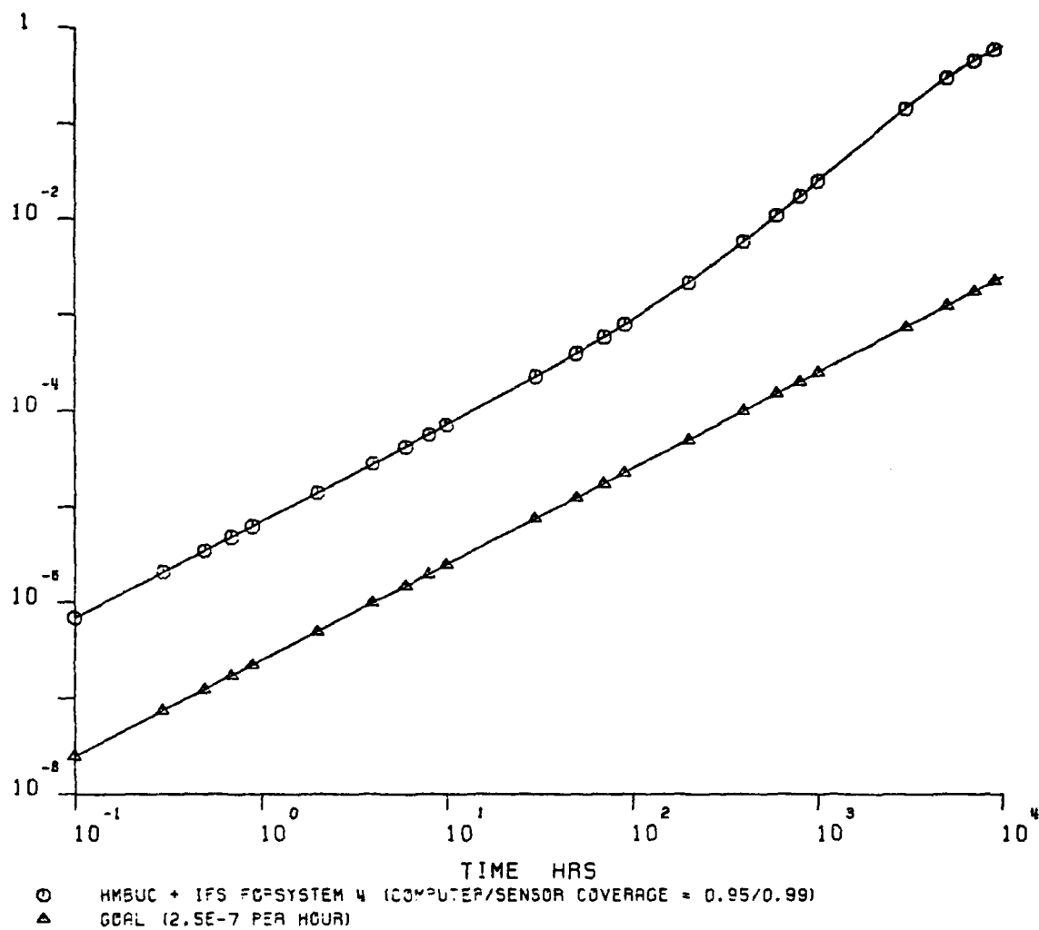
Figure 50. HMBUC and IFS for System 3 (Comp/Sensor Coverage = 0.95/0.99)
