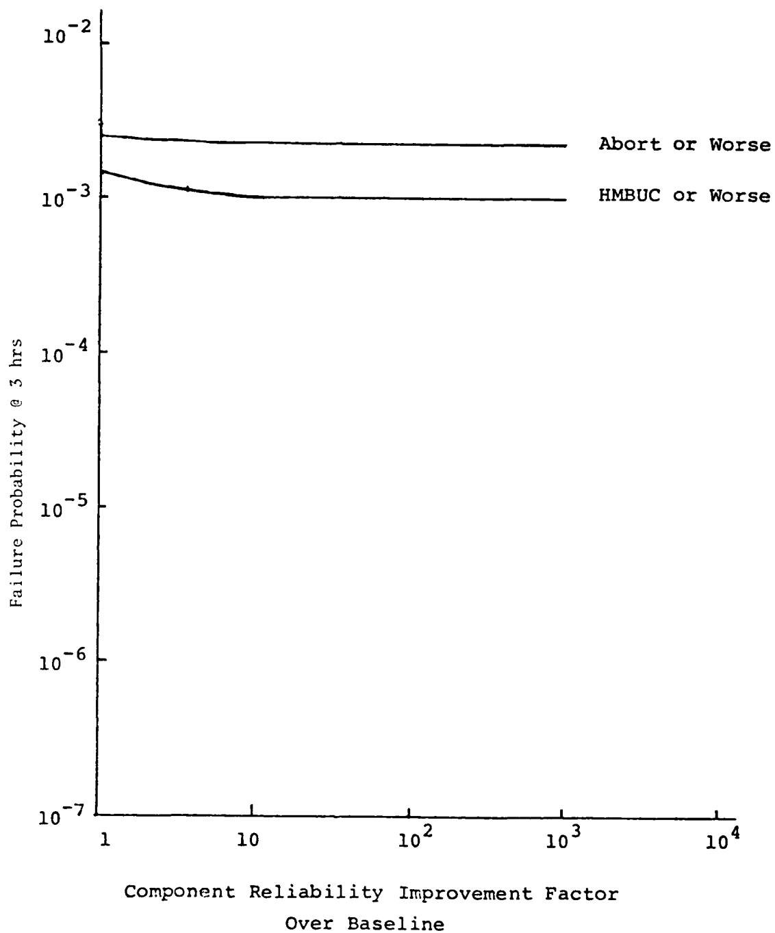
Figure 42. FAFTEEC Reliability Improvement Due to Improvement in Computer Reliability
