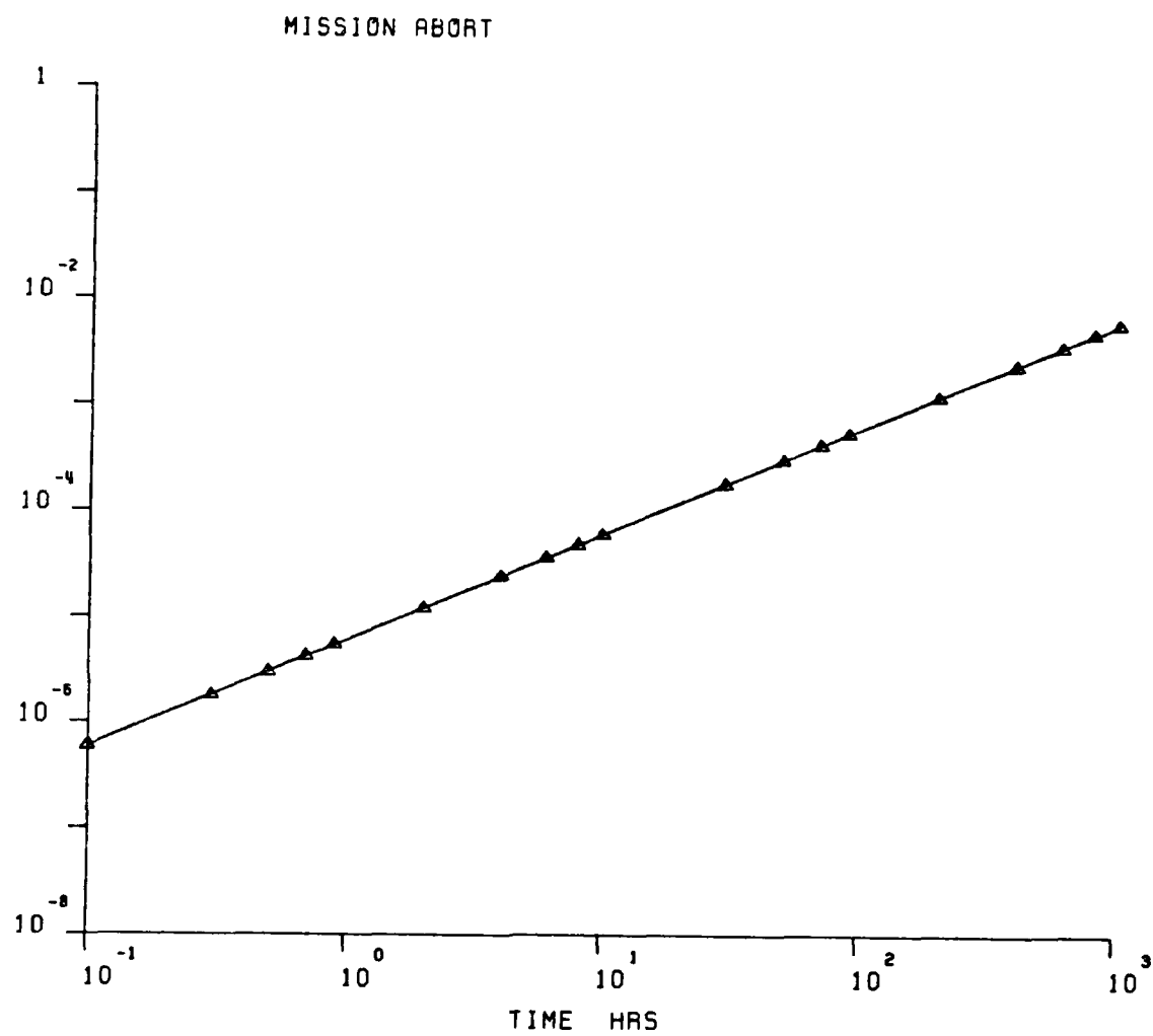
Figure A-17. Markov Model of an Example Engine Controller (5 of 7)
