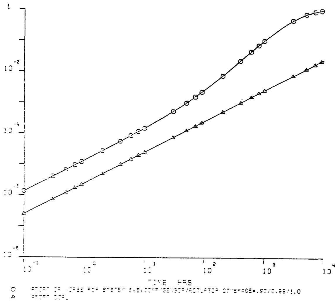
Figure 53. Abort Model for System 4A (Coverage = 0.90/0.99)
