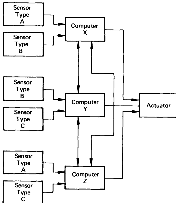
Figure A-1. Control System Example
