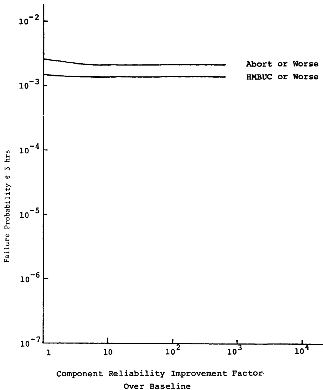
Figure 44. FAFTEEC Reliability Improvement Due to Improvement in Actuator Reliability
