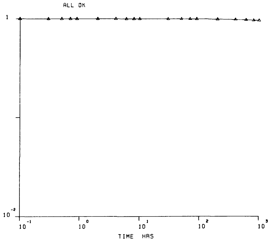
Figure A-17. Markov Model of an Example Engine Controller (1 of 7)
