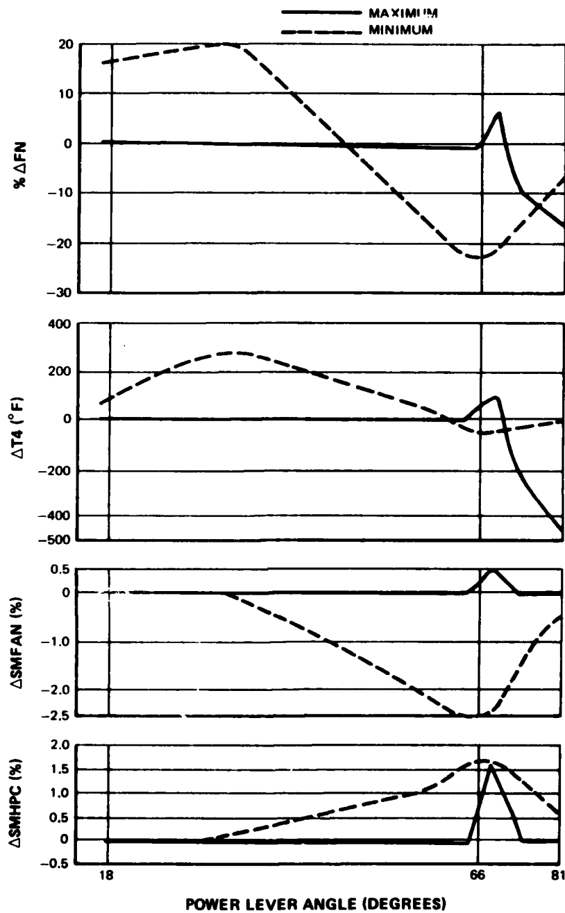
Figure 27. Gas Generator Exhaust Nozzle Area (AJE) Failure Effects at Sea Level Static Conditions
