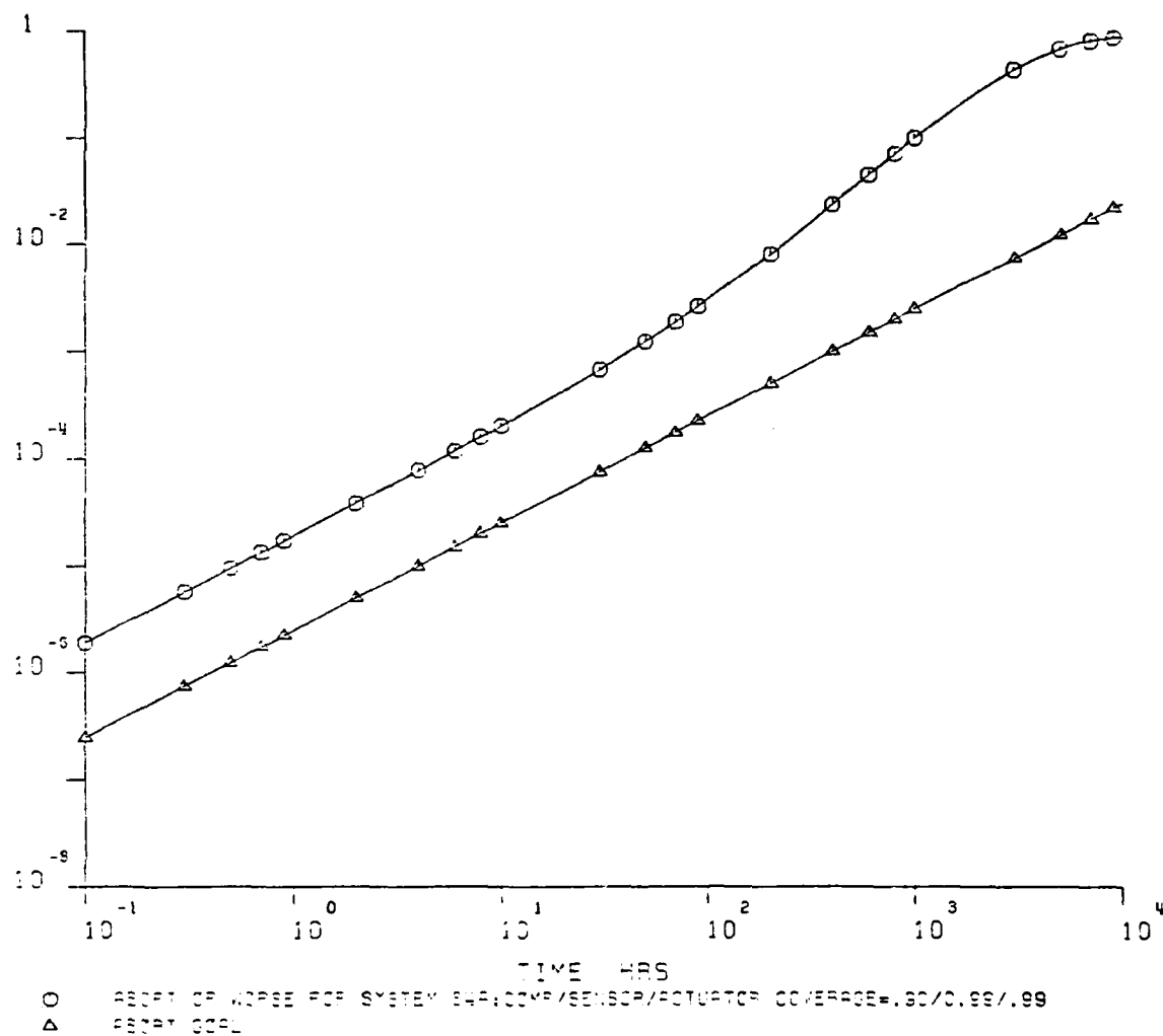
Figure 51. Abort Model for System 4 (Comp/S and A Coverage = 0.90/0.99)
