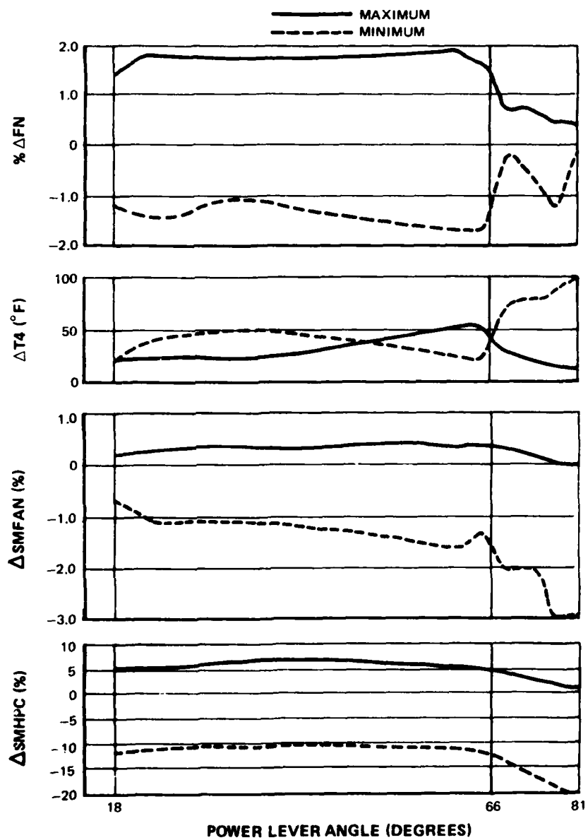
Figure 24. High-Pressure Turbine Area (A4) Failure Effects at Sea Level Static Conditions
