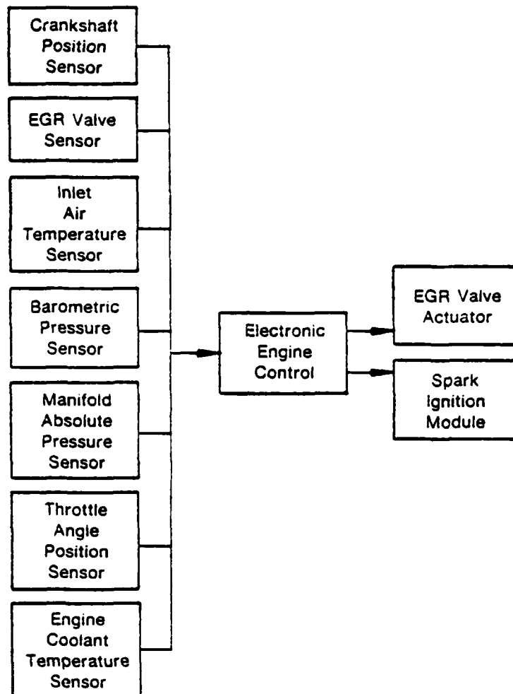
Figure 80. Electronic Engine Control System Ford
