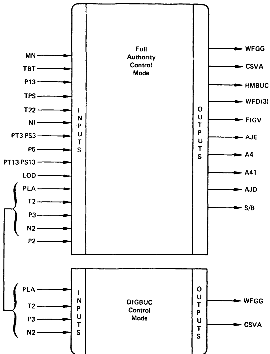
Figure 14. DIGBUC Fail-Soft Mode
