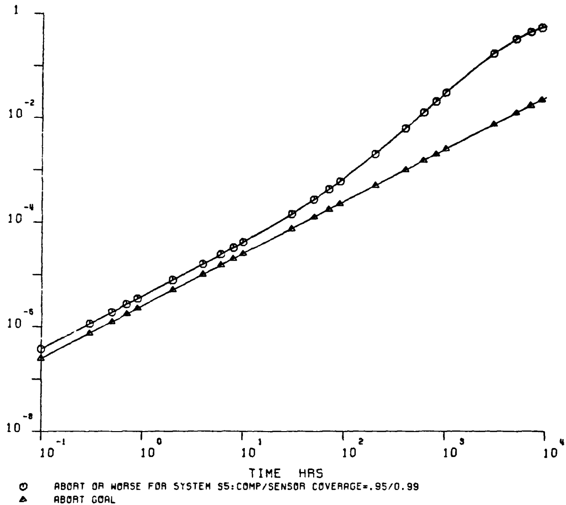
Figure 55. Abort Model for System 5 (Comp/Sensor Coverage = 1/0/0.99)
