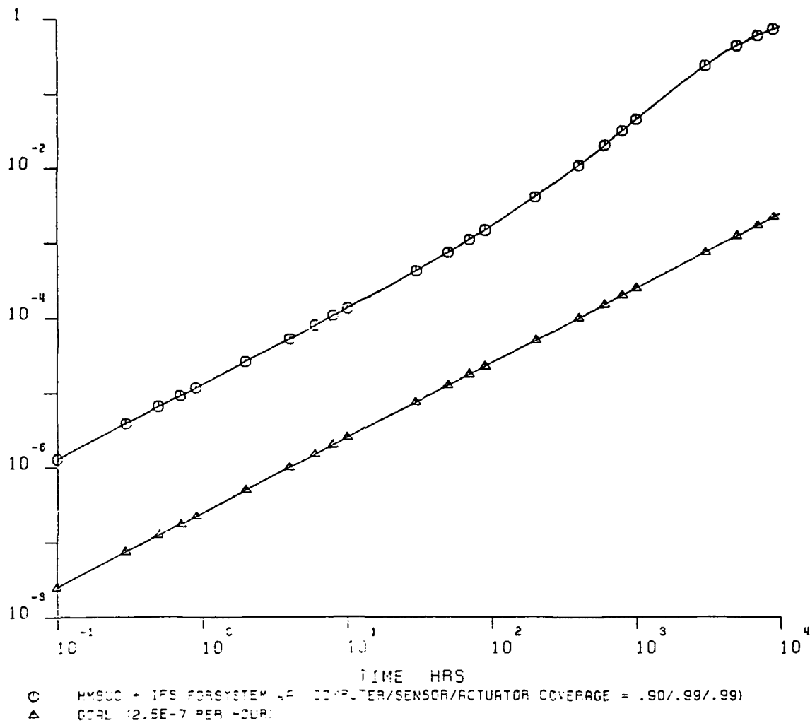
Figure 52. HMBUC and IFS for System 4 (Comp/S and A Coverage = 0.90/0.99)
