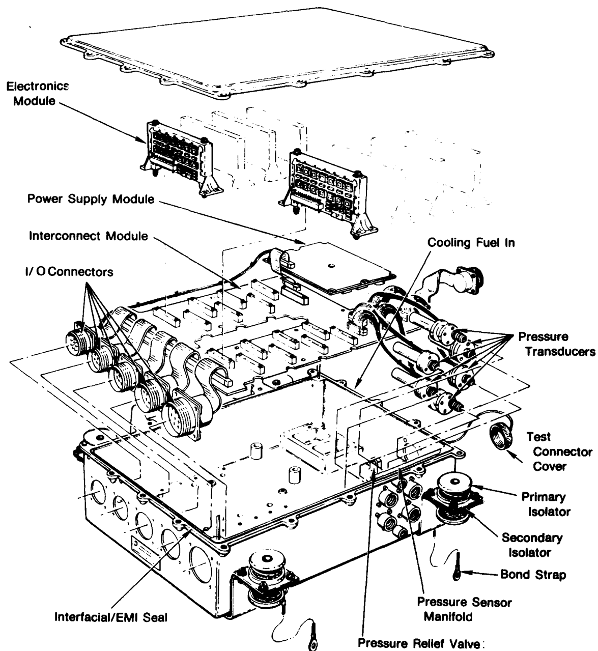
Figure 63. FAFTEEC Exploded View
