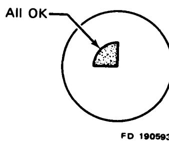
Figure A-10. Resultant Intersection of the Venn Diagrams
