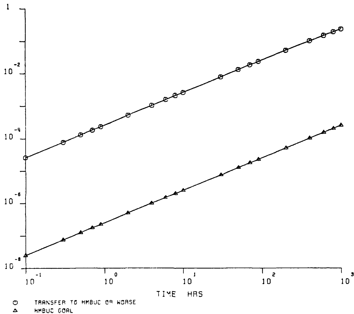
Figure 41. FAFTEEC Baseline Reliability Evaluation: Simplex System (Transfer to HMBUC)
