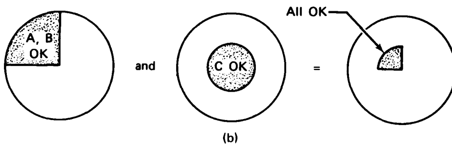
Figure A-9. Intersection of the Venn Diagrams
