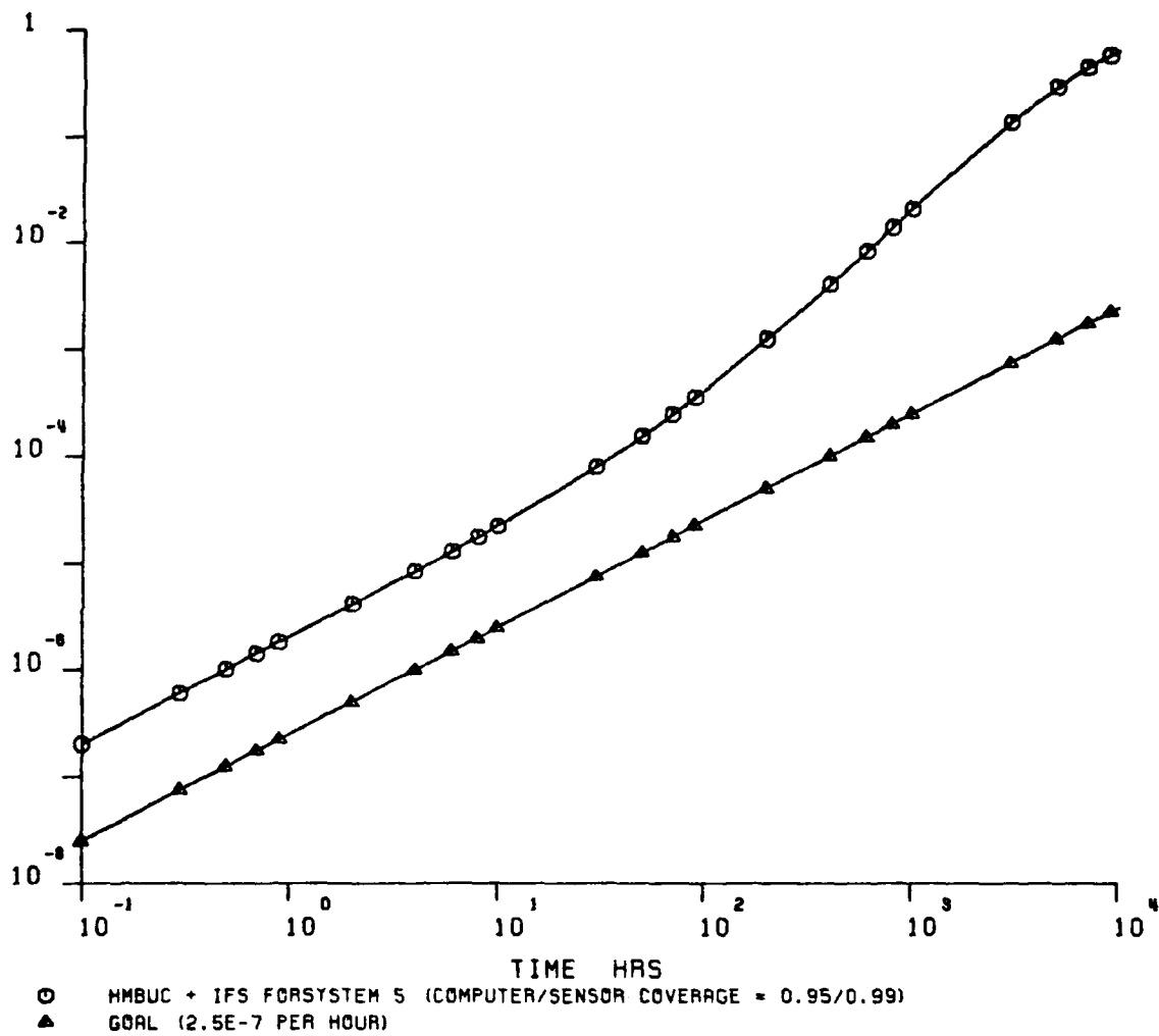
Figure 56. HMBUC and IFS for System 5 (Comp/Sensor Coverage = 1/0/0.99)
