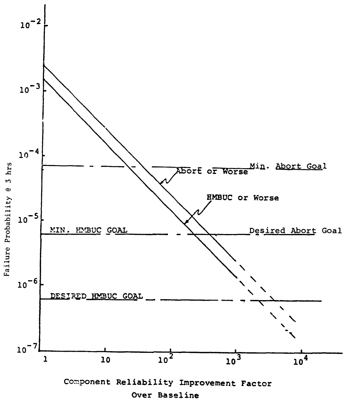
Figure 46. FAFTEEC Reliability Improvements Due to Improvement in All Components
