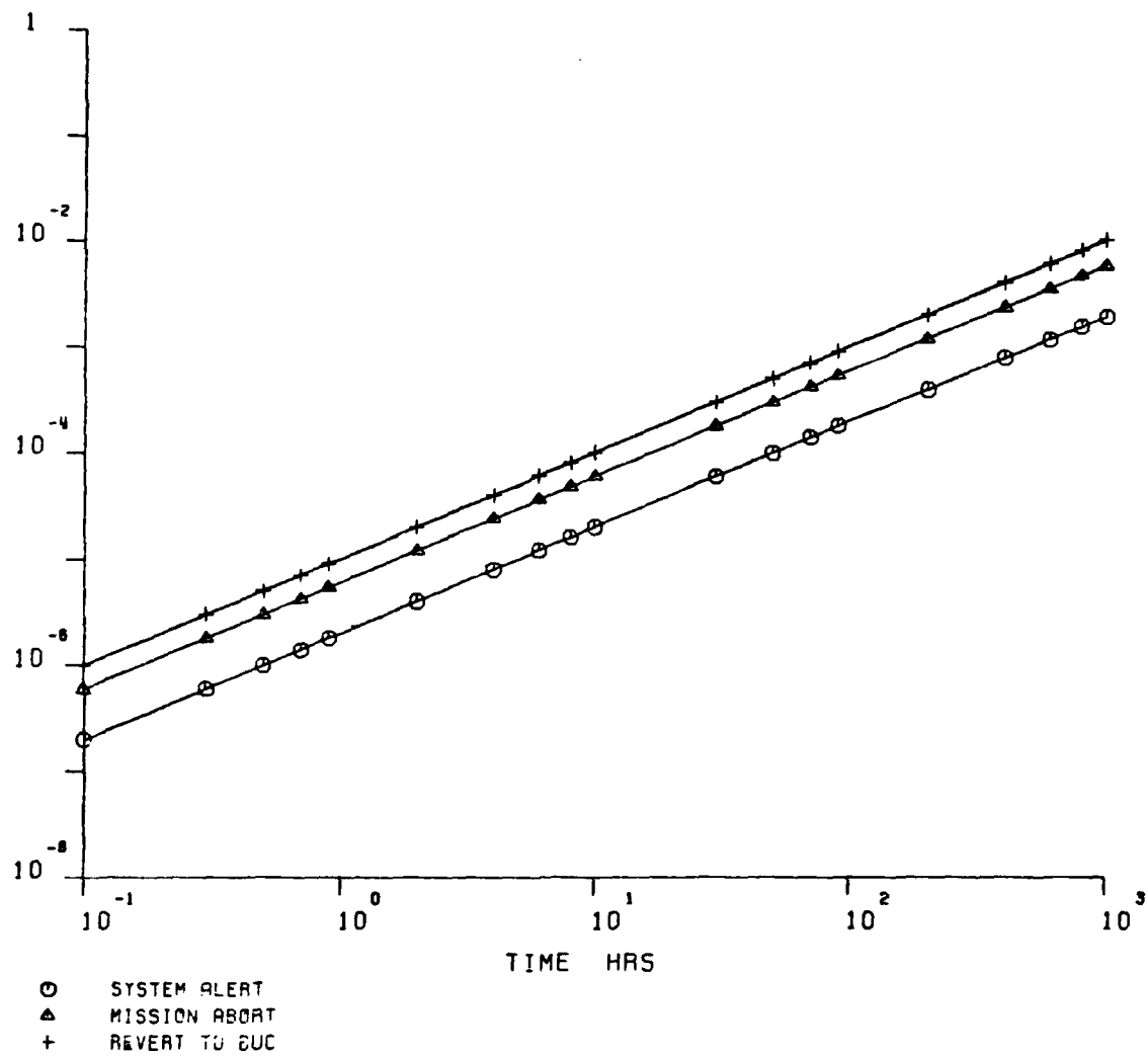
Figure A-17. Markov Model of an Example Engine Controller (7 of 7)
