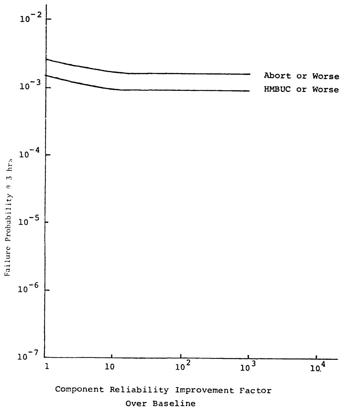
Figure 43. FAFTEEC Reliability Improvement Due to Improvement in Sensor Reliability
