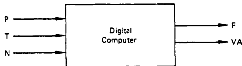
Figure A-13. An Example Engine Controller
