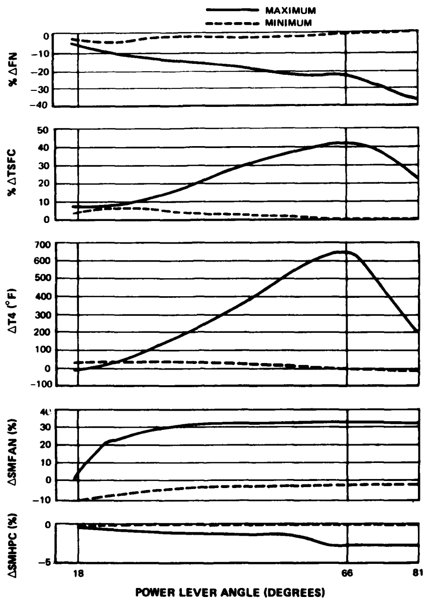
Figure 26. Fan Duct Exhaust Nozzle Area (AJD) Failure Effects at Sea Level Static Conditions
