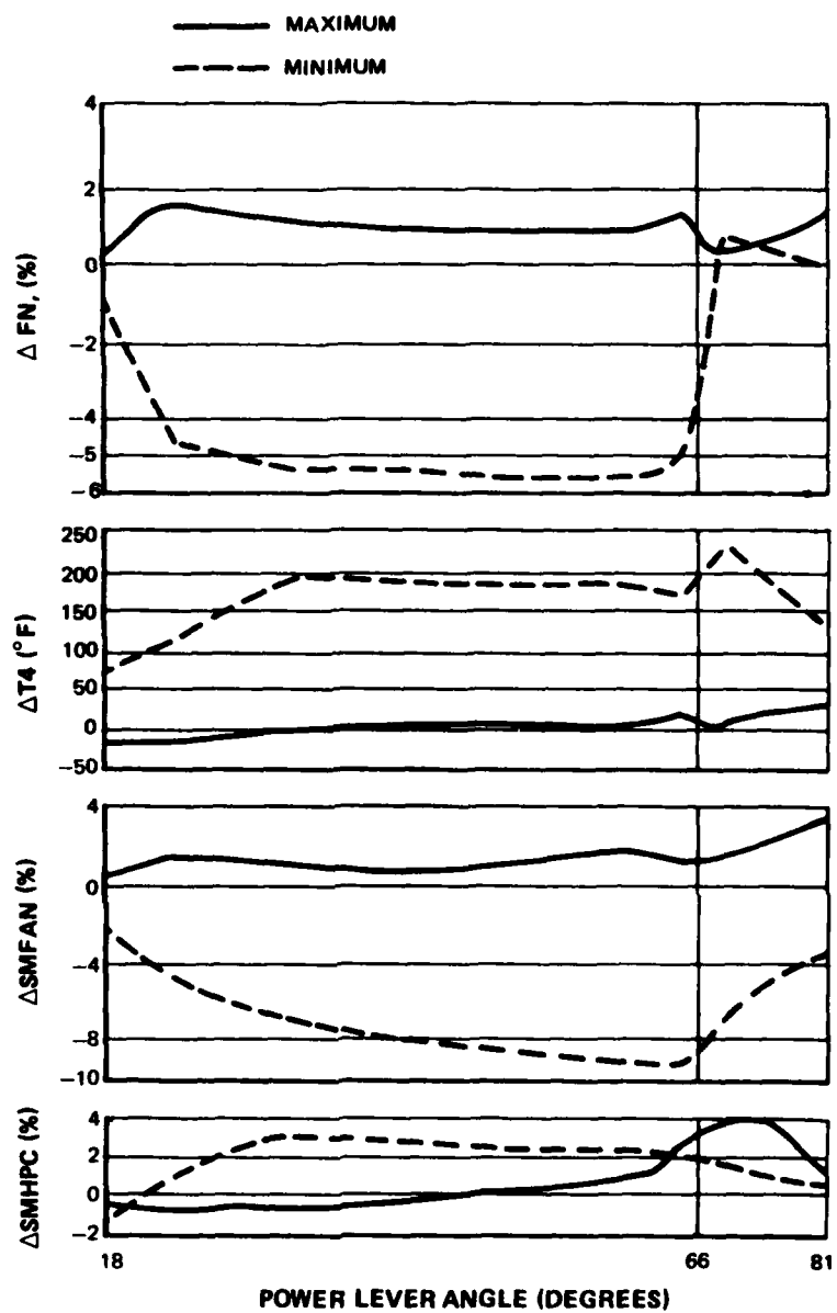
Figure 25. Low-Pressure Turbine Area (A41) Failure Effects at Sea Level Static Conditions
