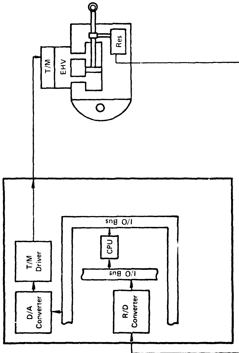
Figure 18. FAFTEEC CSVA Loop Implementation
