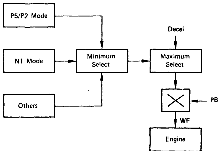
Figure 4. WF Control Logic (Sheet 1 of 3)
