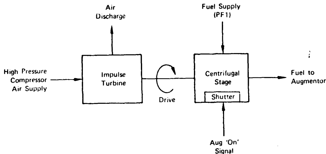
Figure 23. Augmentor Fuel Pump Functional Block Diagram
