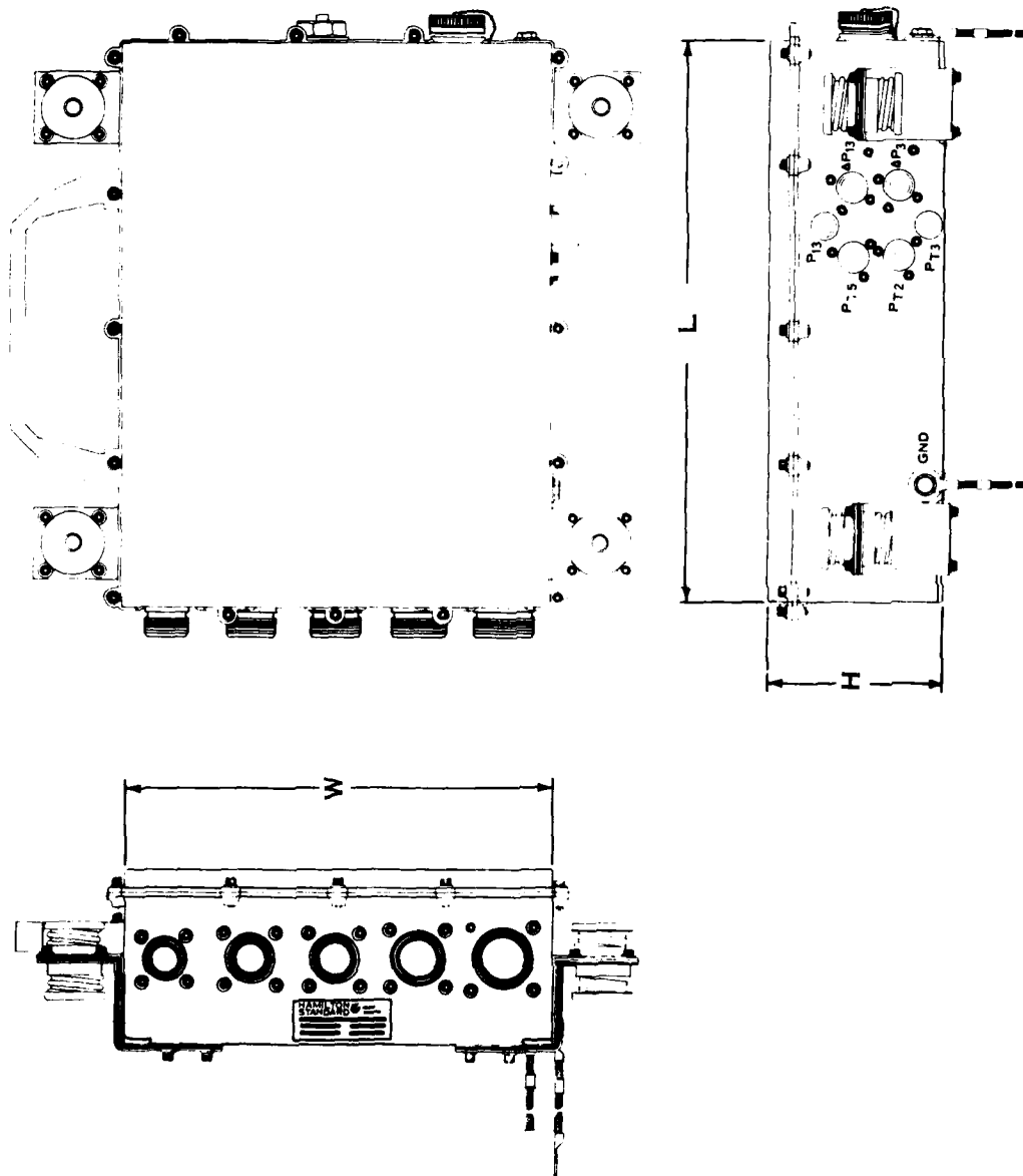
Figure 62. FAFTEEC Package Outline
