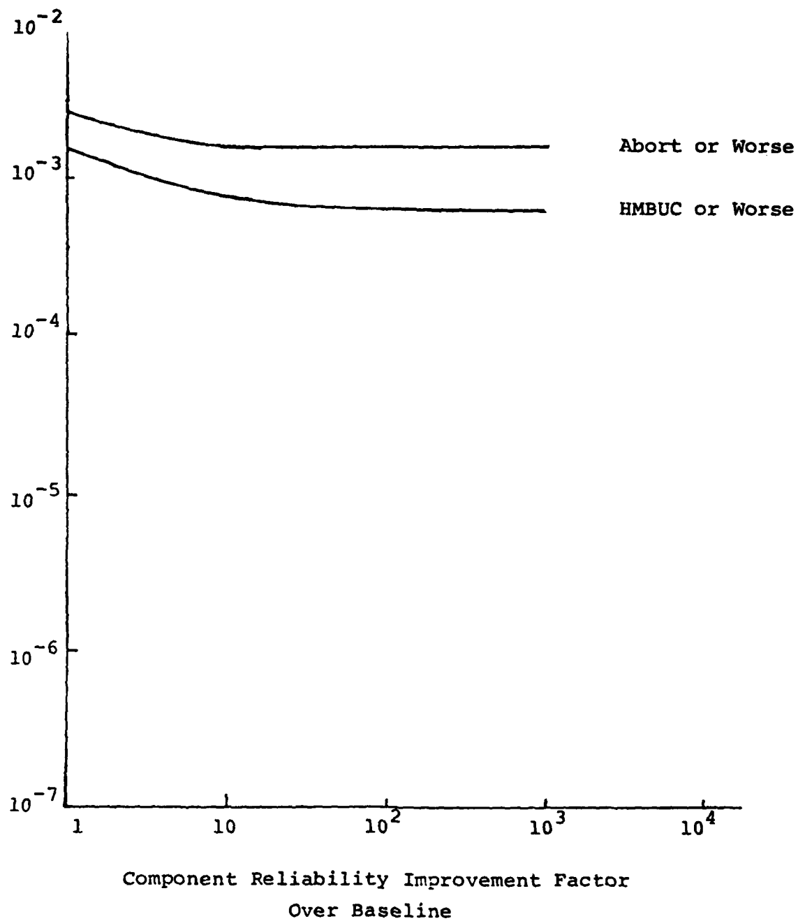
Figure 45. FAFTEEC Reliability Improvement Due to Improvement in Miscellaneous Components
