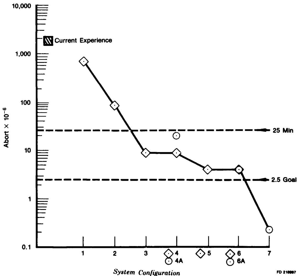
Figure 75. Mission Abort Reliability
