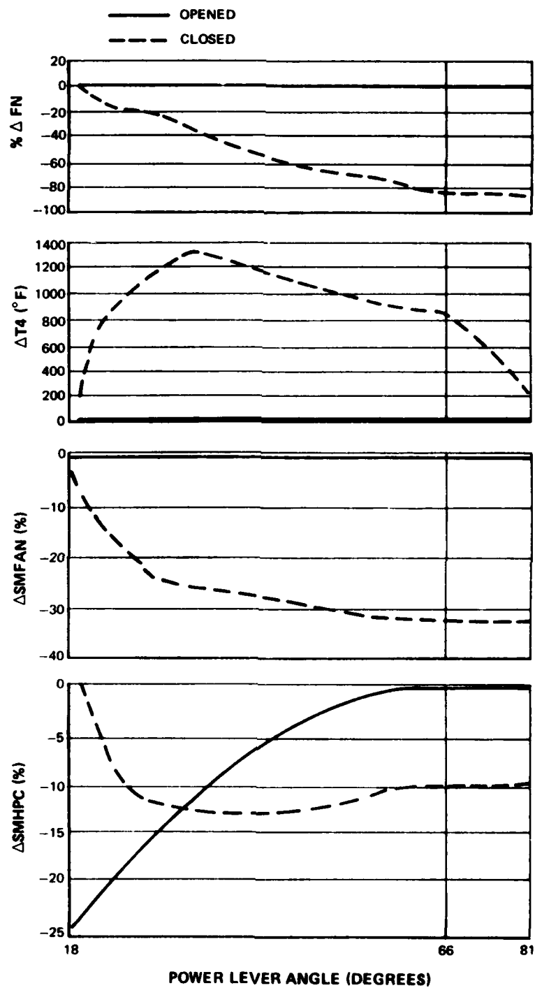
Figure 29. Compressor Stator Vane Angle (CSVA) Failure Effects at Sea Level Static Conditions
