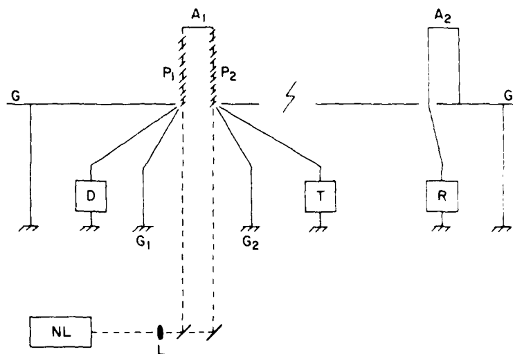
Fig. 1 — A schematic diagram of the RF propagation experiment. A_1 represents the plasma antenna rising above the local ground plane, G ; A_2 represents a second antenna rising above its local ground plane, G' . NL represents the Nd:glass laser whose beams --- define the plasma antenna. L represents the long focal length lens. D represents a high voltage system that drives the electric discharge and goes to ground at G_2 . T represents the RF transmitter and G_1 the RF ground. R represents the receiver.
