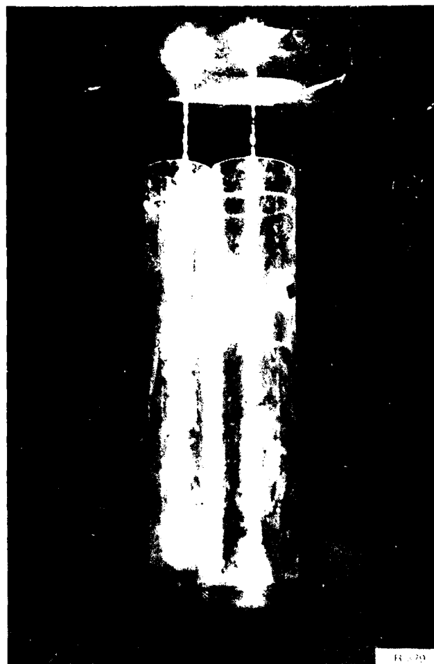
Fig. 4 — An open shutter photograph of the plasma beads produced by laser-induced, aerosol-initiated air breakdown. Note that when this photograph was taken, two plastic insulating tubes were being used, one around each plasma column.
