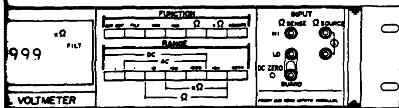
Voltmeter, Controls, Indicators, and Connectors
