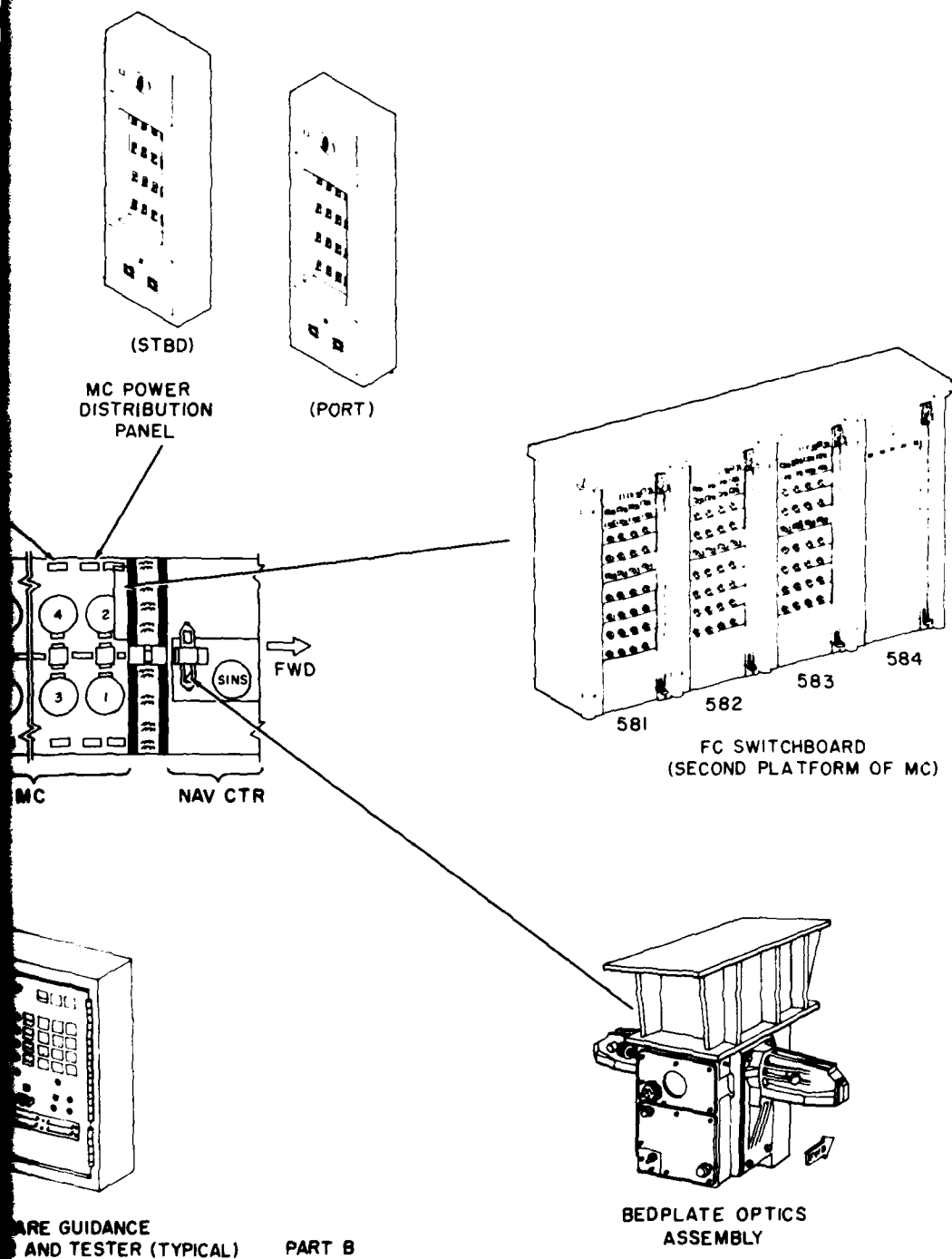
Figure 14. TRIDENT I (C-4) Fire Control Subsystem - Equipments.
