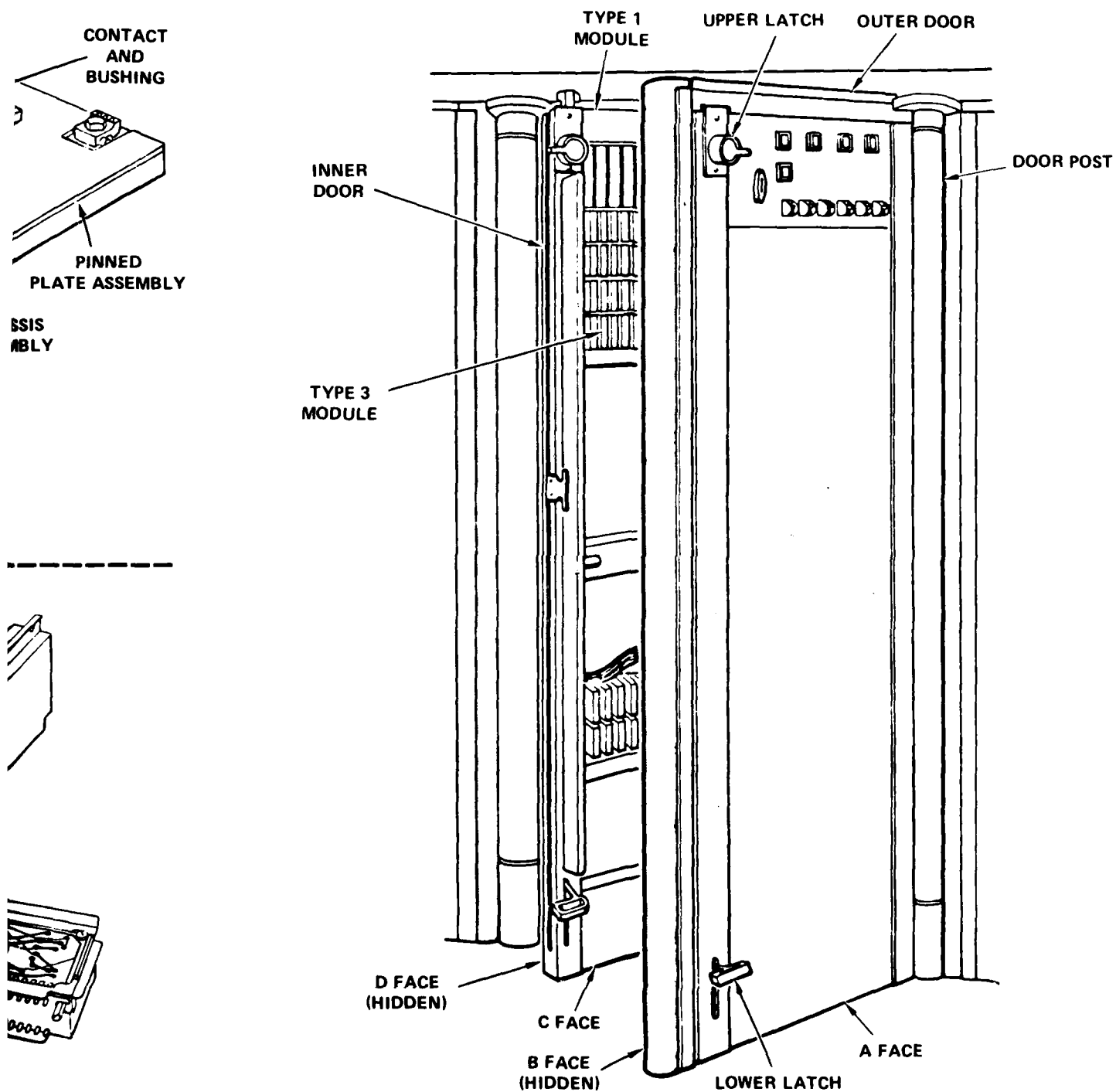
Figure 13. Fire Control Subsystem - Typical Door Assembly.
