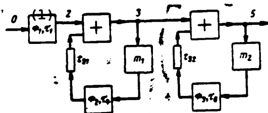
Fig. 8.1.1. Block diagram of double storage device.
