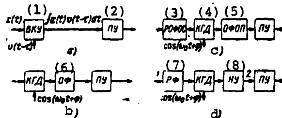
Fig. 6.2.1. Block diagrams of receivers for coherent storage of completely known signals. Key: (1) Cross-correlation device; (2) Threshold device; (3) Radio-frequency optimum filter for single pulsed signal; (4) Coherent detector; (5) Video frequency optimum filter for envelope of sequence of pulsed signals; (6) Optimum filter; (7) Radio-frequency filter; (8) Video frequency storage device.
