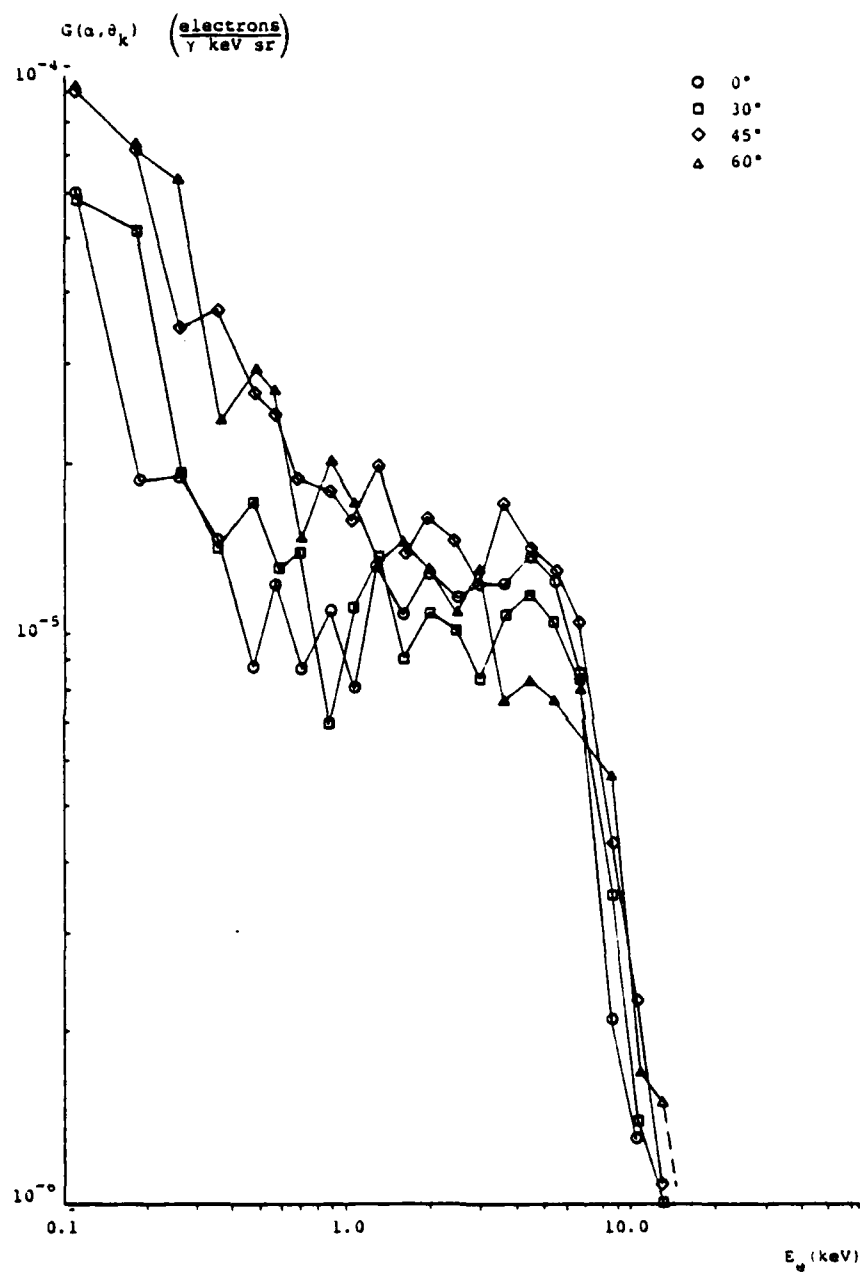
FIGURE 33. Differential Yield vs. Energy; Mylar, Unfiltered
