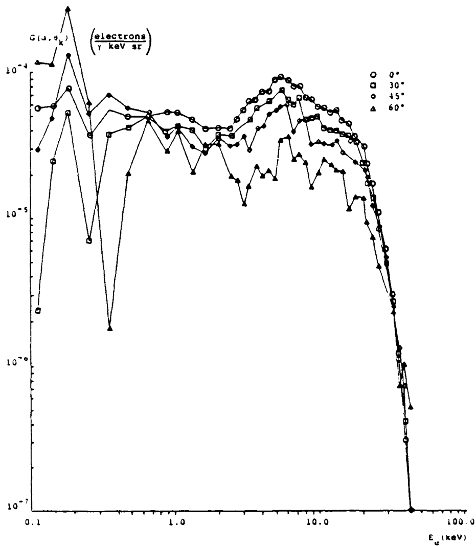
FIGURE 23. Differential Yield vs. Energy; Ta with Filter
