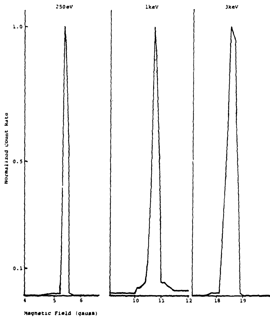
FIGURE 21. Channel 4 (60°) Resolution
