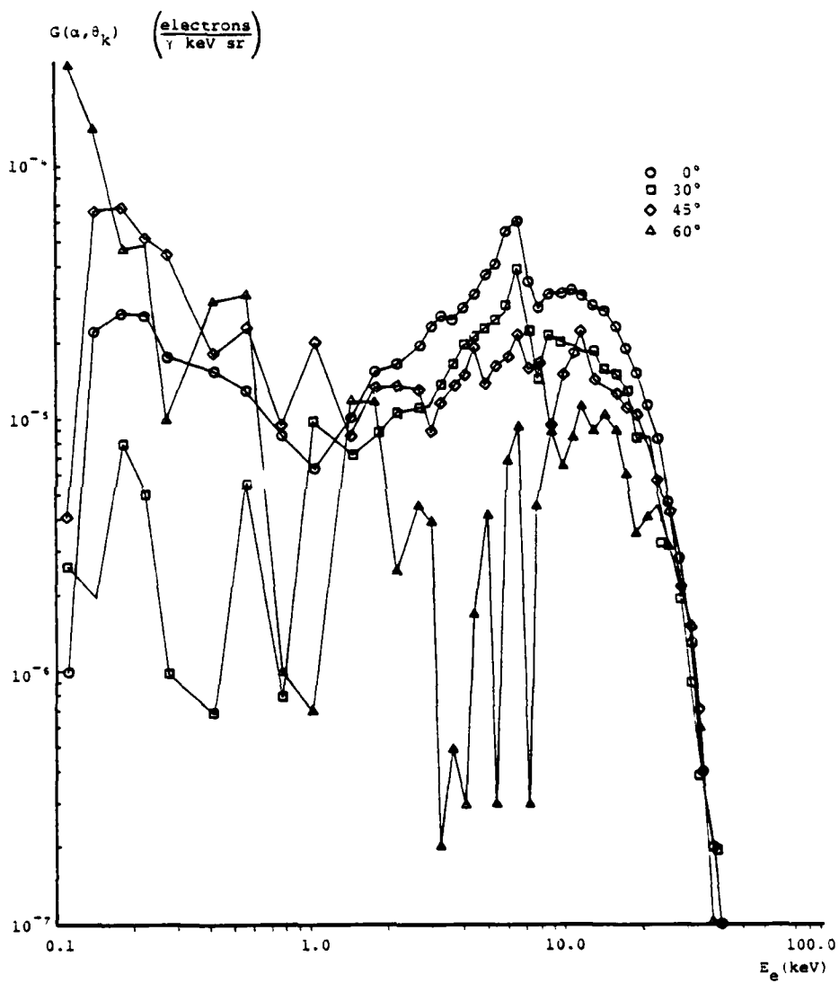
FIGURE 22. Differential Yield vs. Energy; Cu with Filter
