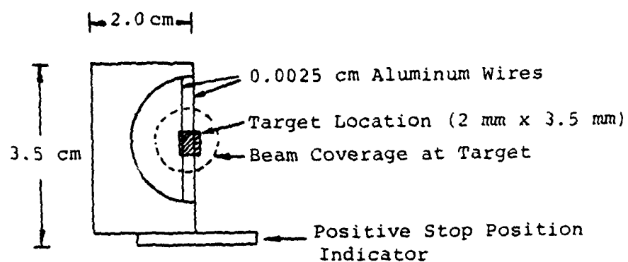
FIGURE 15. Target Mount
