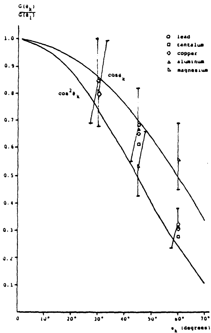
FIGURE 37. Normalized Yield vs. \theta_k ; Metal Targets
