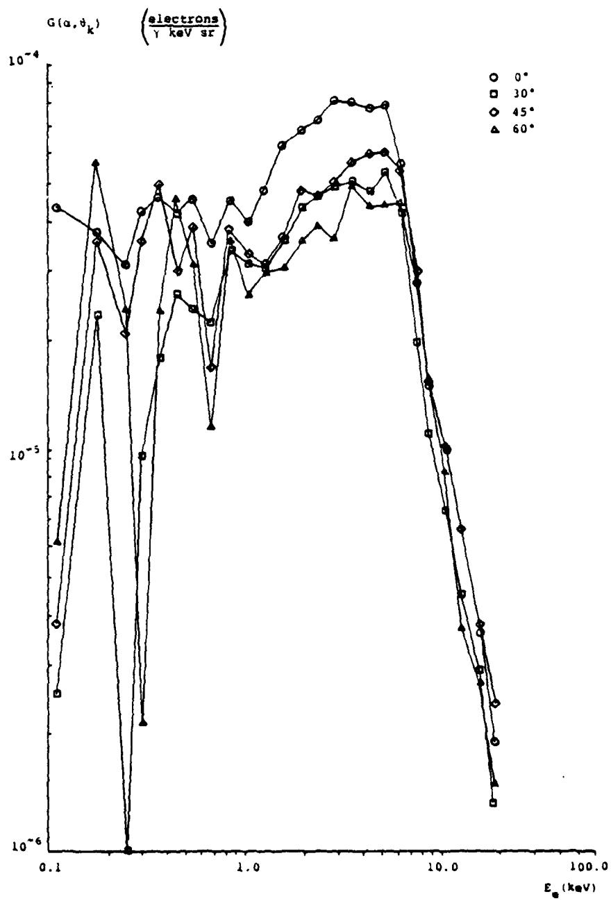
FIGURE 29. Differential Yield vs. Energy; Cover Glass, Unfiltered
