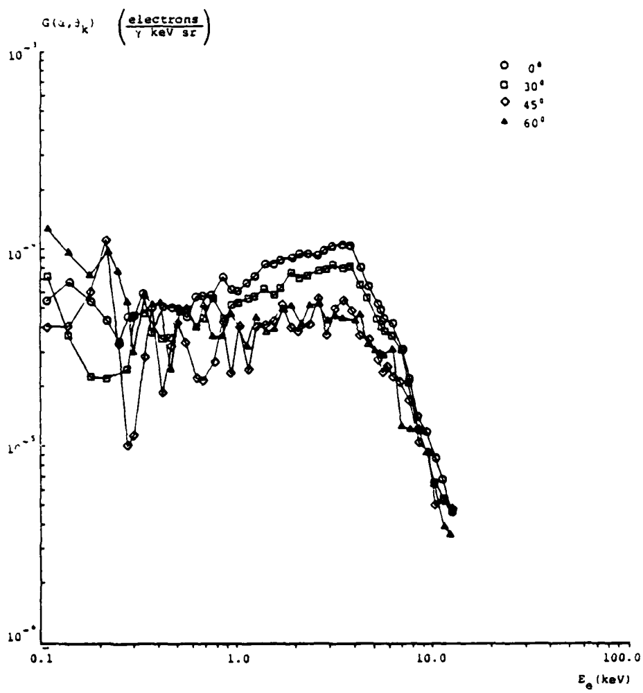
FIGURE 24. Differential Yield vs. Energy; Mg, Unfiltered
