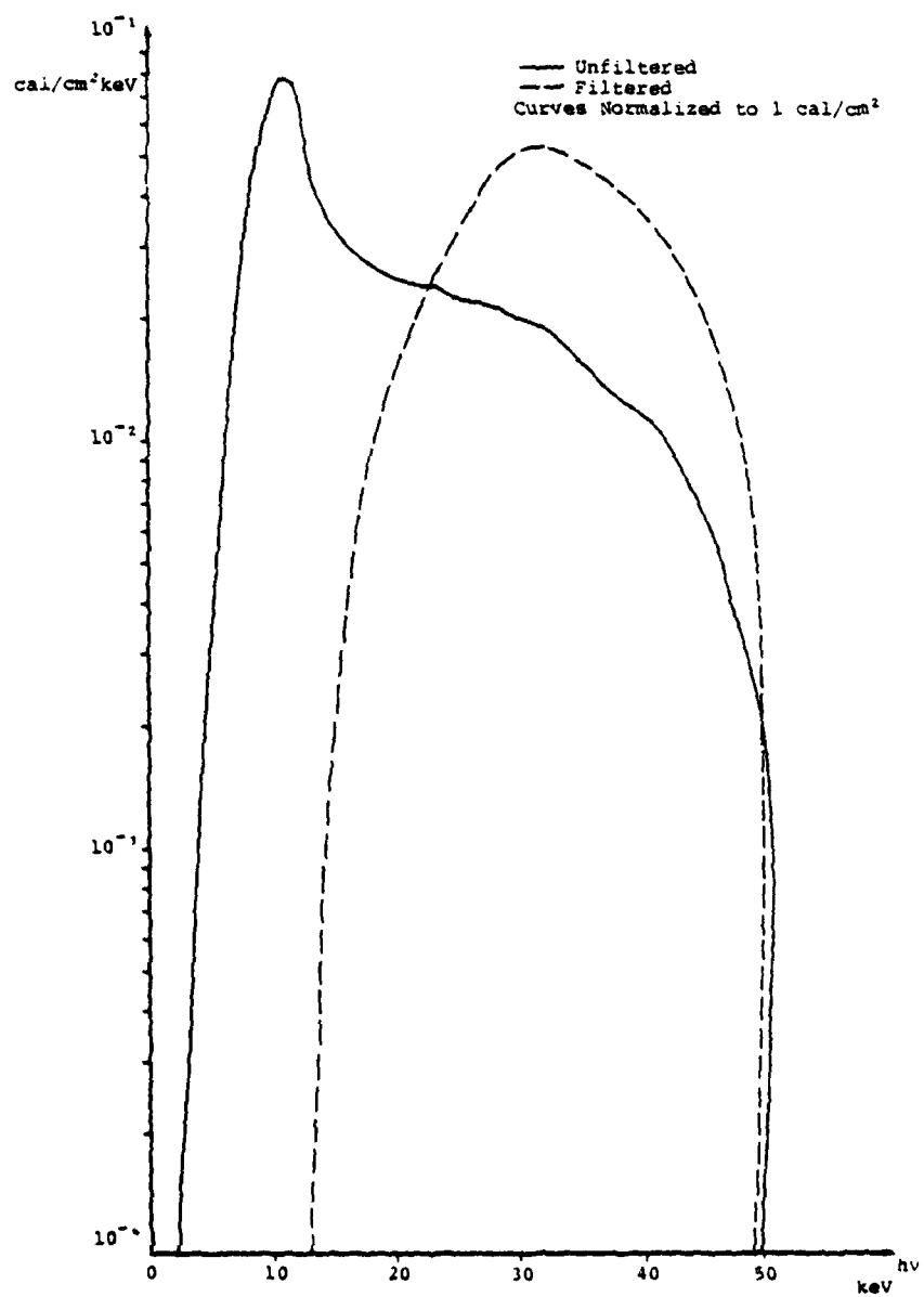
FIGURE 11. X-Ray Energy Distribution.
