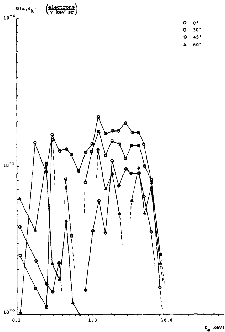
FIGURE 32. Differential Yield vs. Energy; Kevlar, Unfiltered
