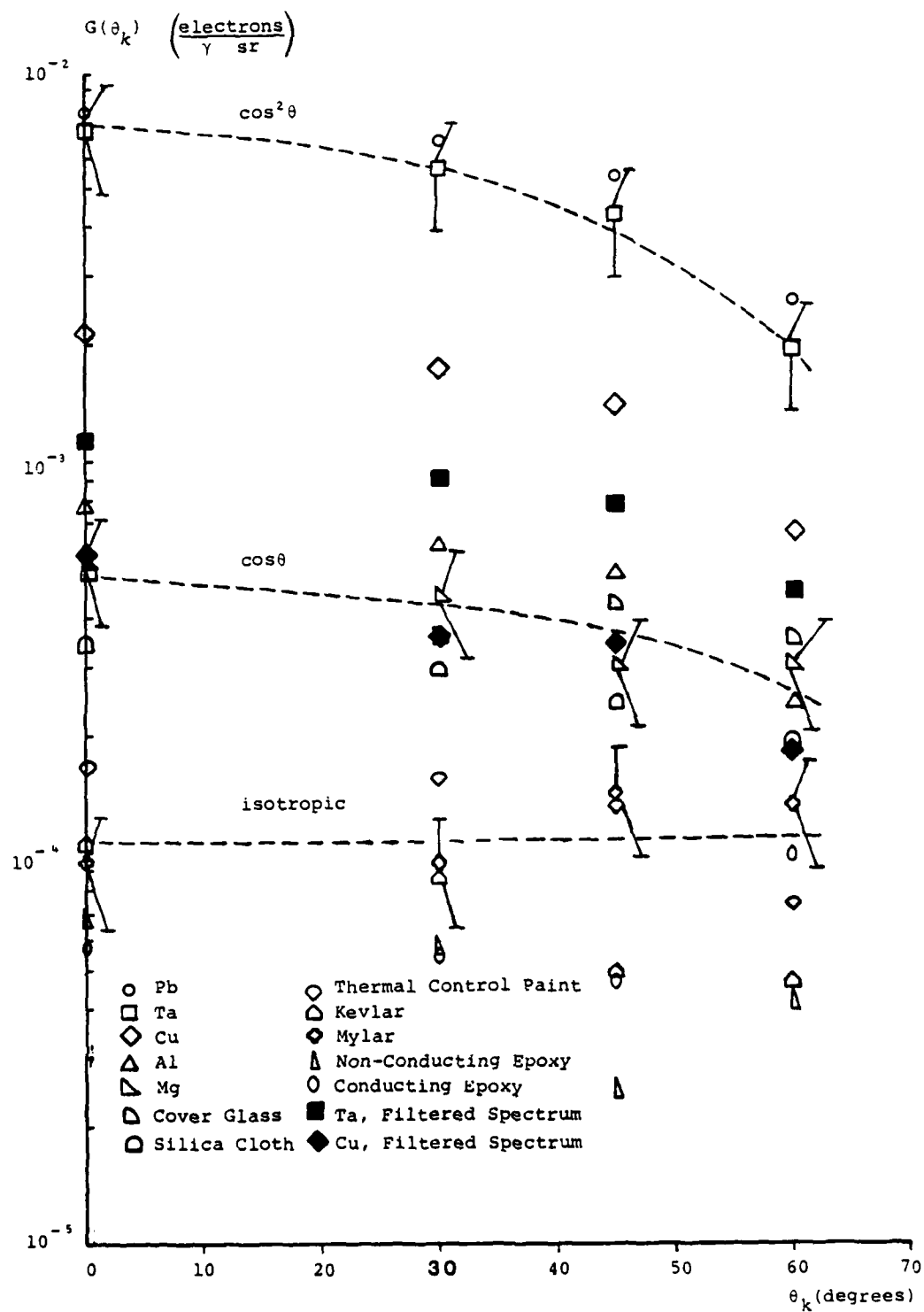
FIGURE 36. Energy Integrated Yield
