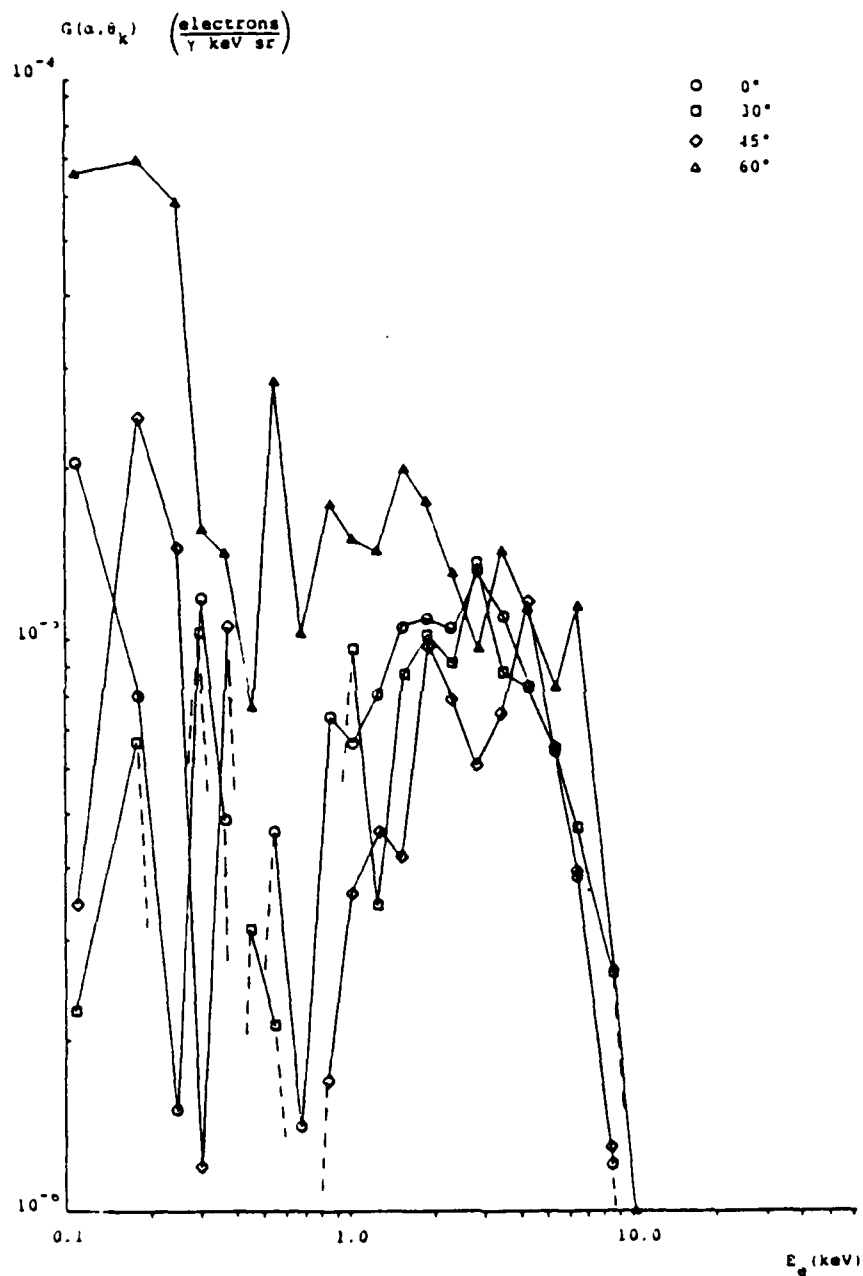
FIGURE 34. Differential Yield vs. Energy; Nonconducting Epoxy, Unfiltered
