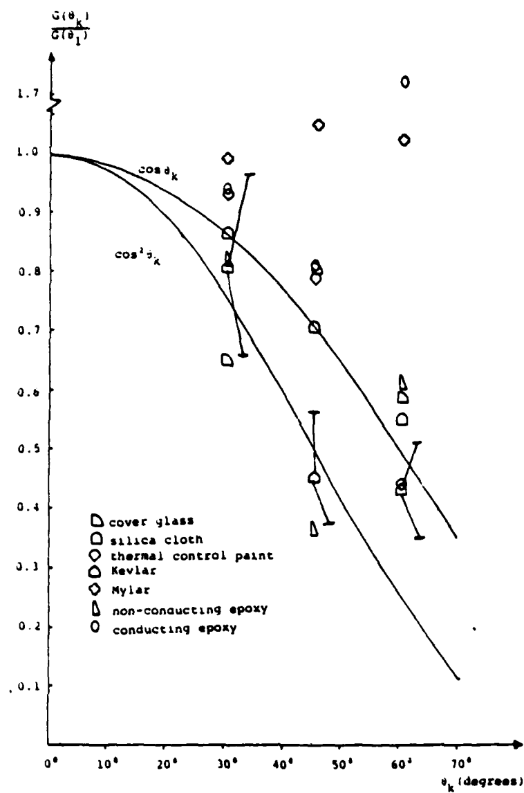
FIGURE 38. Normalized Yield Versus \theta_k ; Nonmetallic Targets
