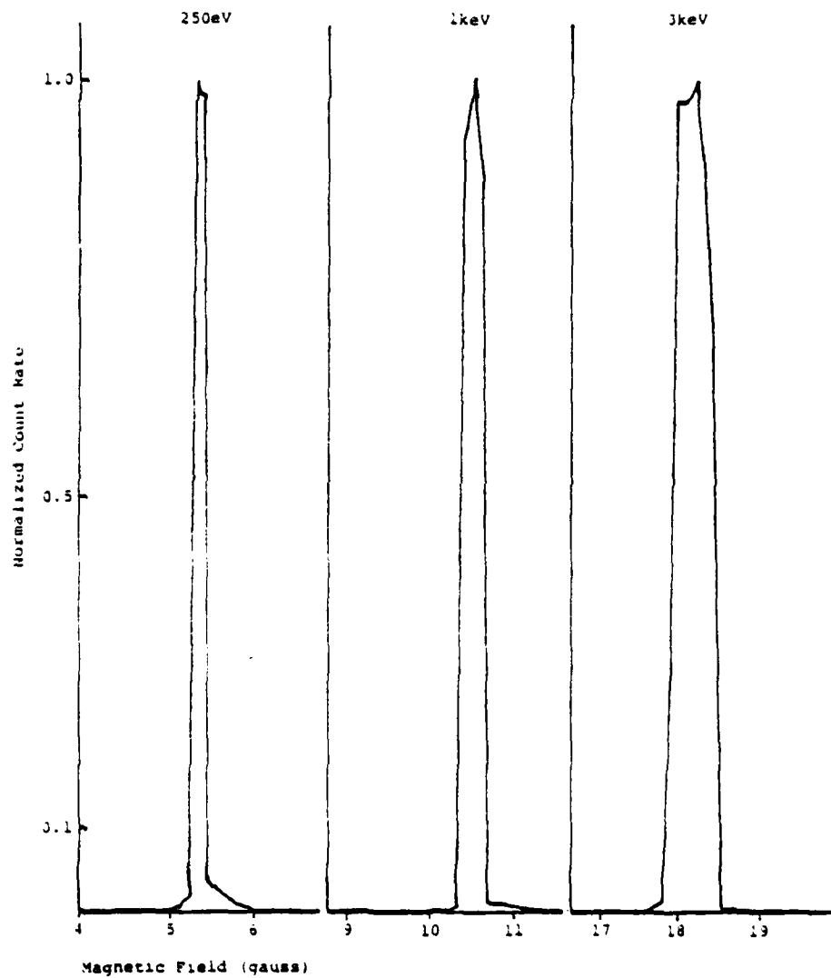
FIGURE 18. Channel 1 ( 0^\circ ) Resolution
