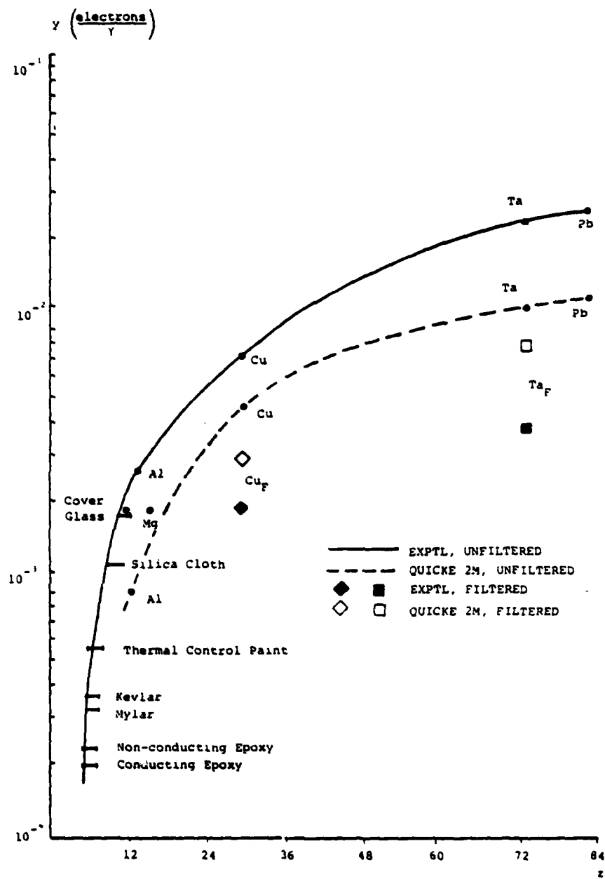
FIGURE 39. Yield Versus Atomic Number
