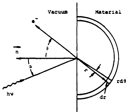
FIGURE 2. Photoelectric Yield Model Geometry
