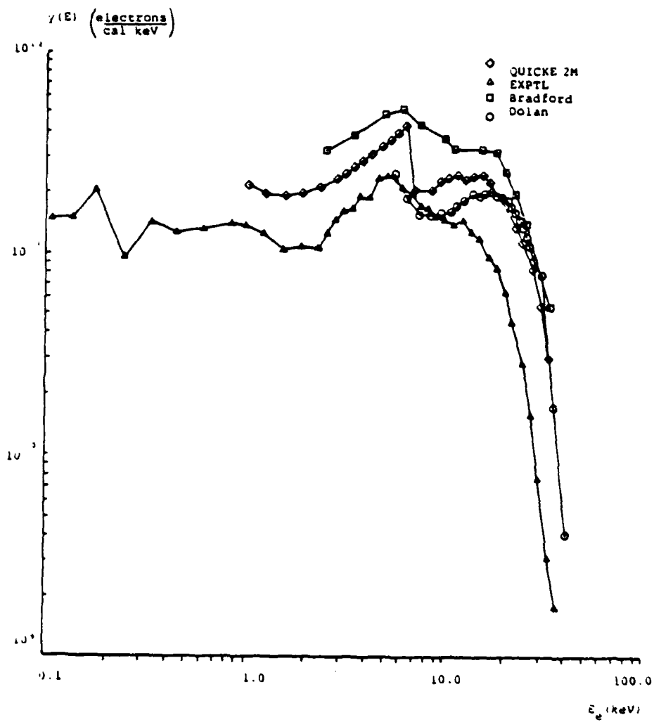
FIGURE 41 . Experiment and Code Comparison; Ta Filtered Spectrum
