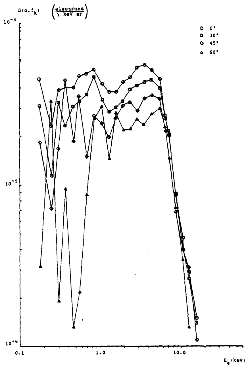
FIGURE 30. Differential Yield vs. Energy; Silica Cloth, Unfiltered
