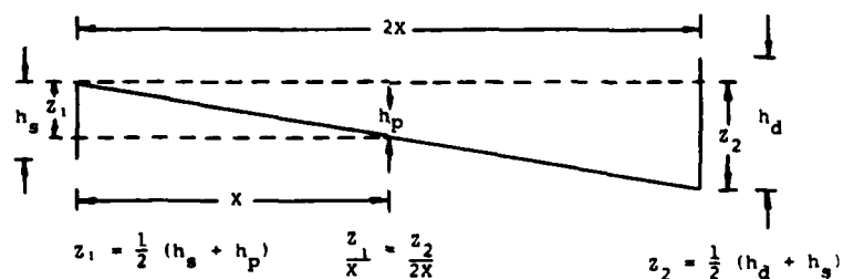
FIGURE 8. Vertical Collimation Geometry
