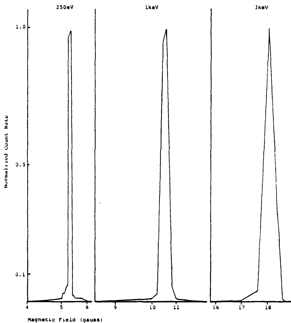
FIGURE 19. Channel 2 (30°) Resolution
