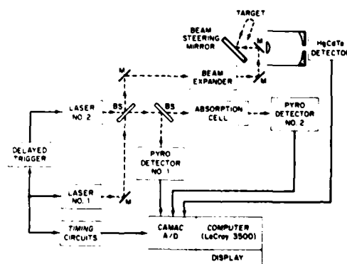
Fig. 1. Schematic of dual-laser DIAL system used for temporal correlation measurements.
