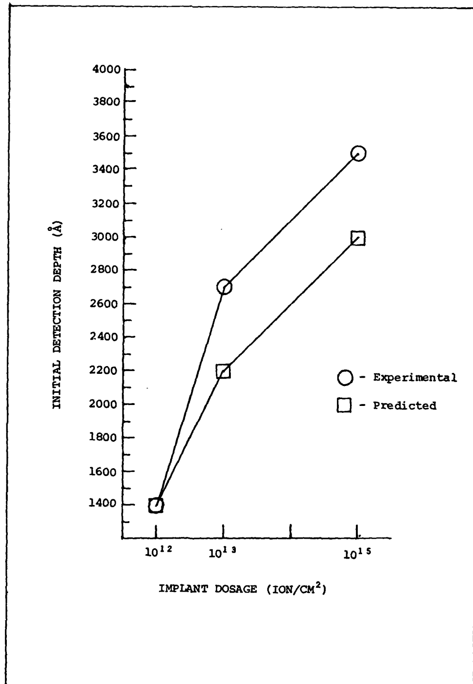
Fig. 12. Comparison of Initial Cathodoluminescence Detection Depths with LSS Profiles
