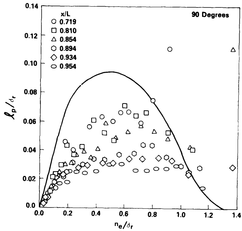
Figure 16d - Angular Location, \theta = 90 Degrees
