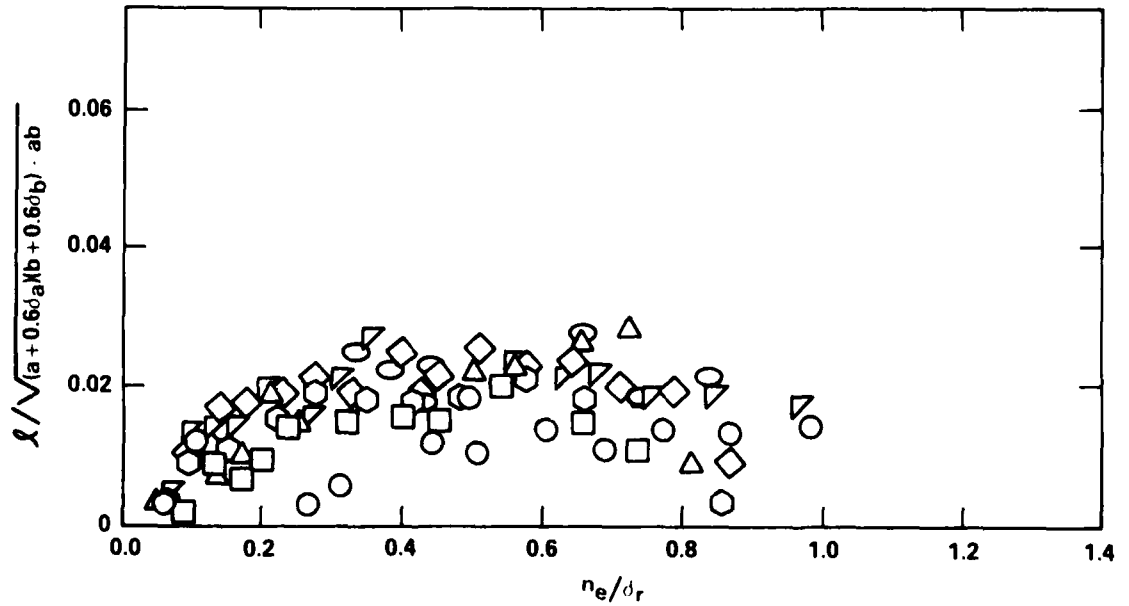
Figure 18f - Present Model, 80 Degree Plane
