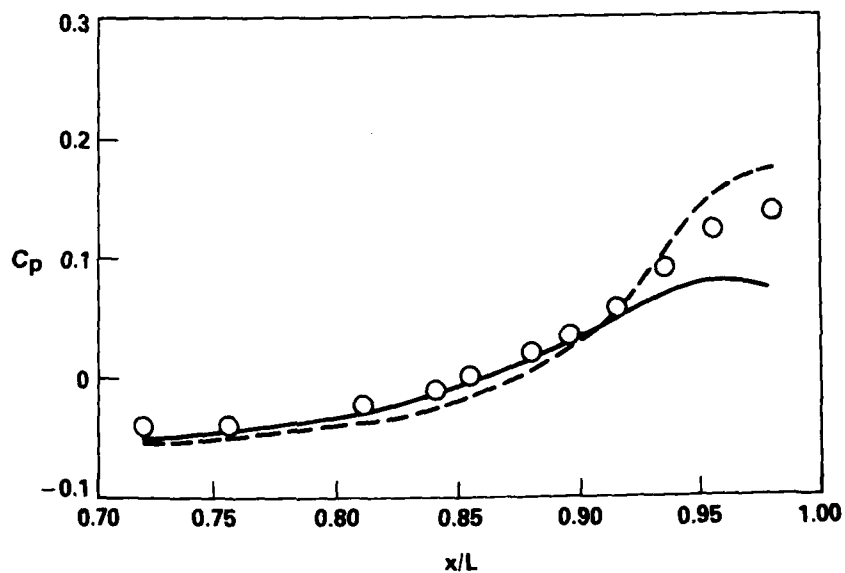
Figure 6d - \theta = 80 Degrees
