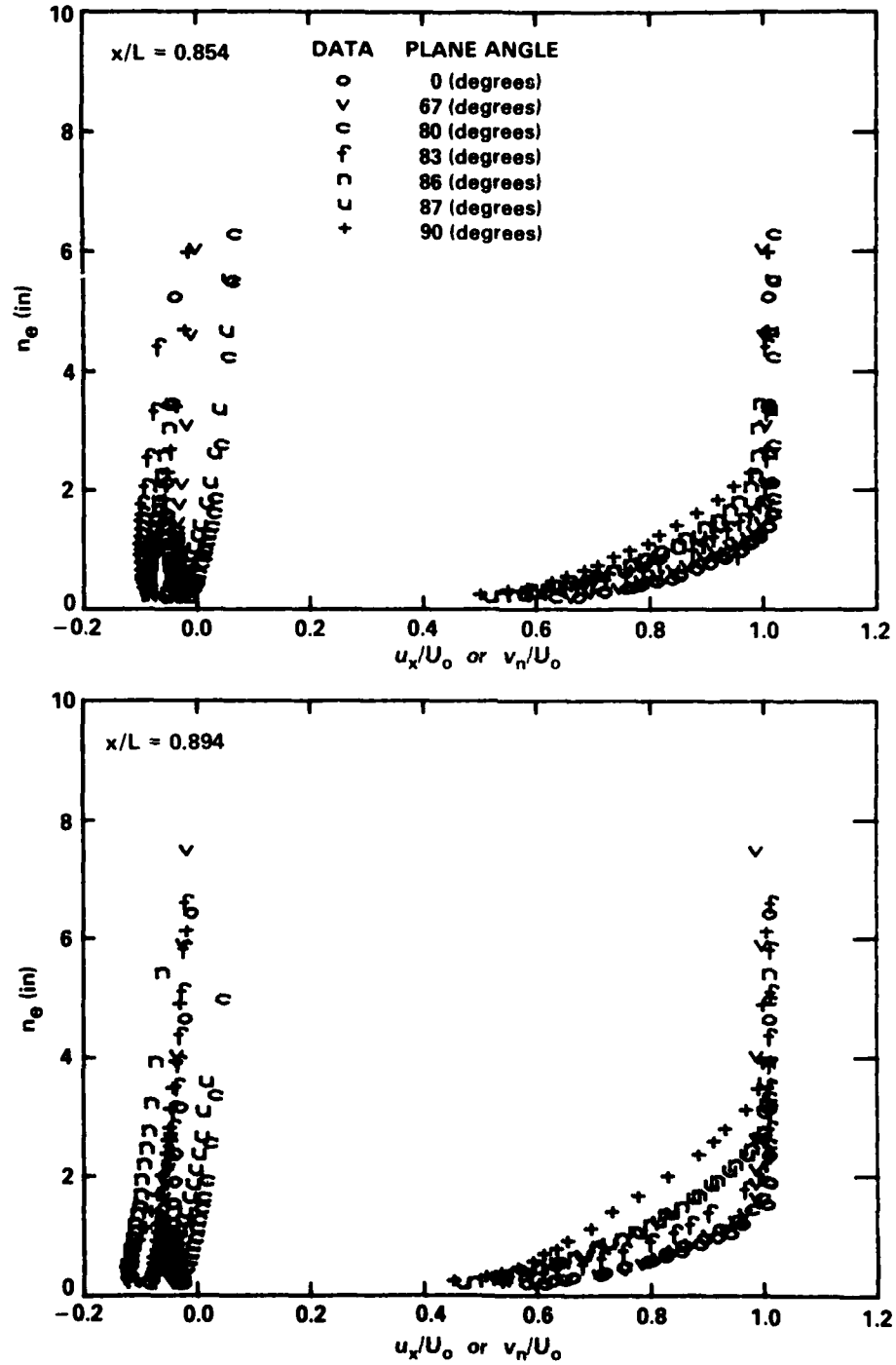
Figure 7b - Nondimensional Axial Lengths, x/L = 0.854 and 0.894
