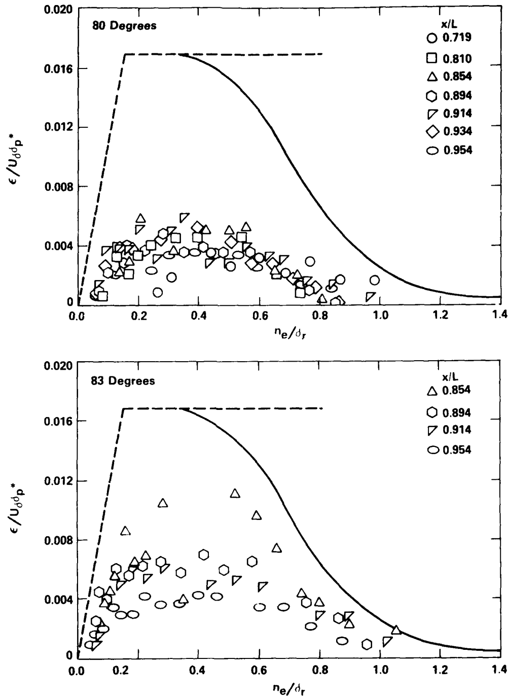
Figure 15b - Angular Locations, \theta = 80 and 83 Degrees
