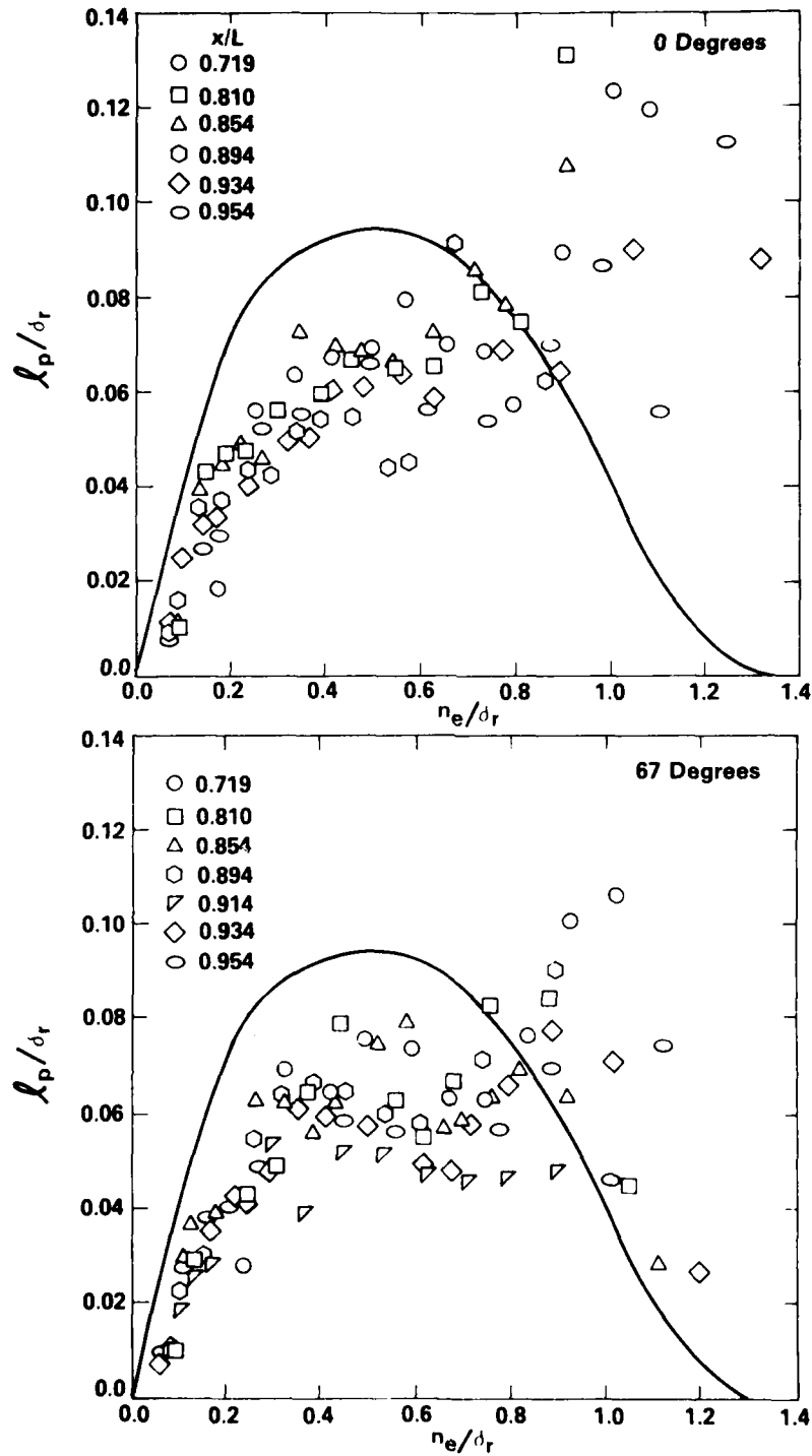
Figure 16a - Angular Locations, \theta = 0 and 67 Degrees
