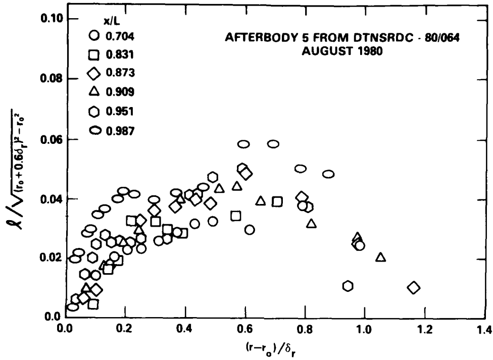
Figure 18c - Afterbody 5
