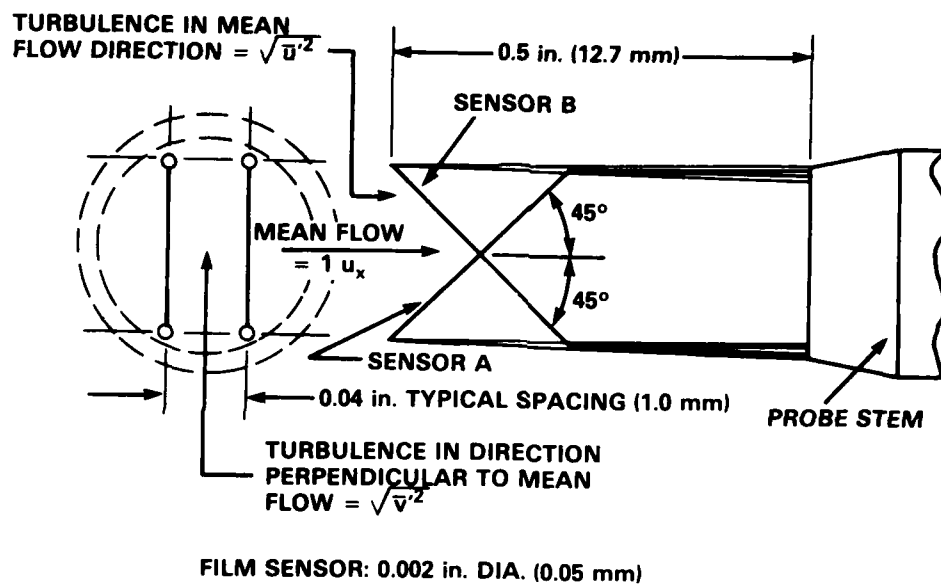
Figure 5 - Schematic of a Two-Element Sensor Alined 90 Degrees to Each Other and 45 Degrees to the Probe Axis
