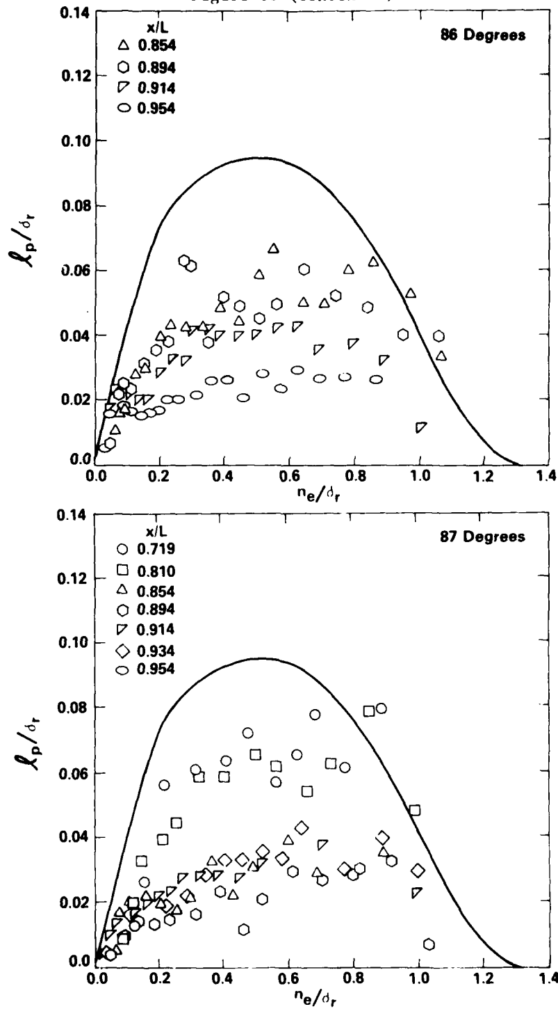
Figure 16c - Angular Locations, \theta = 86 and 87 Degrees
