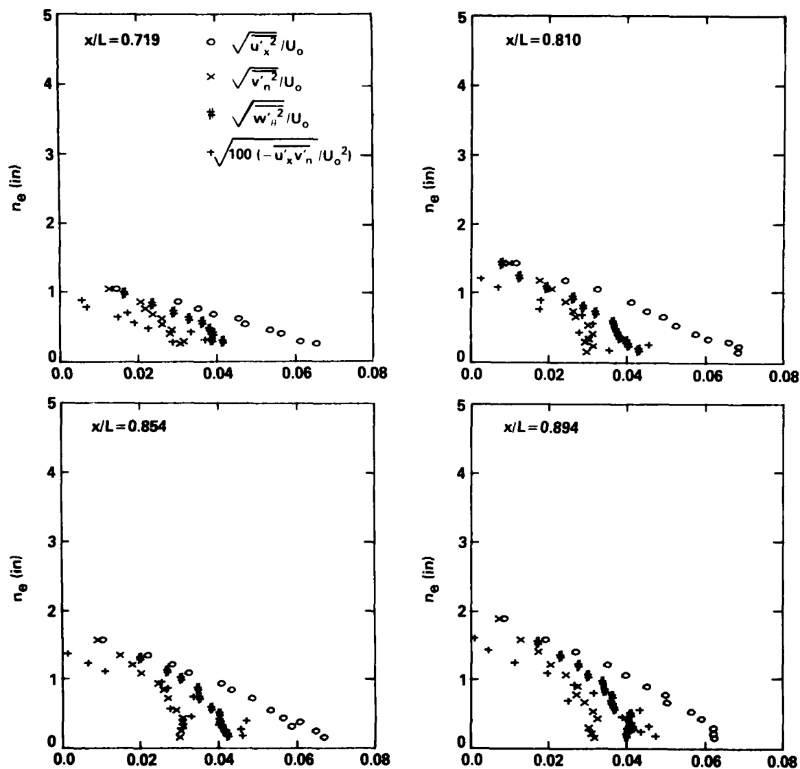
Figure 10a - Nondimensional Axial Lengths, x/L = 0.719, 0.810, 0.854, and 0.894
