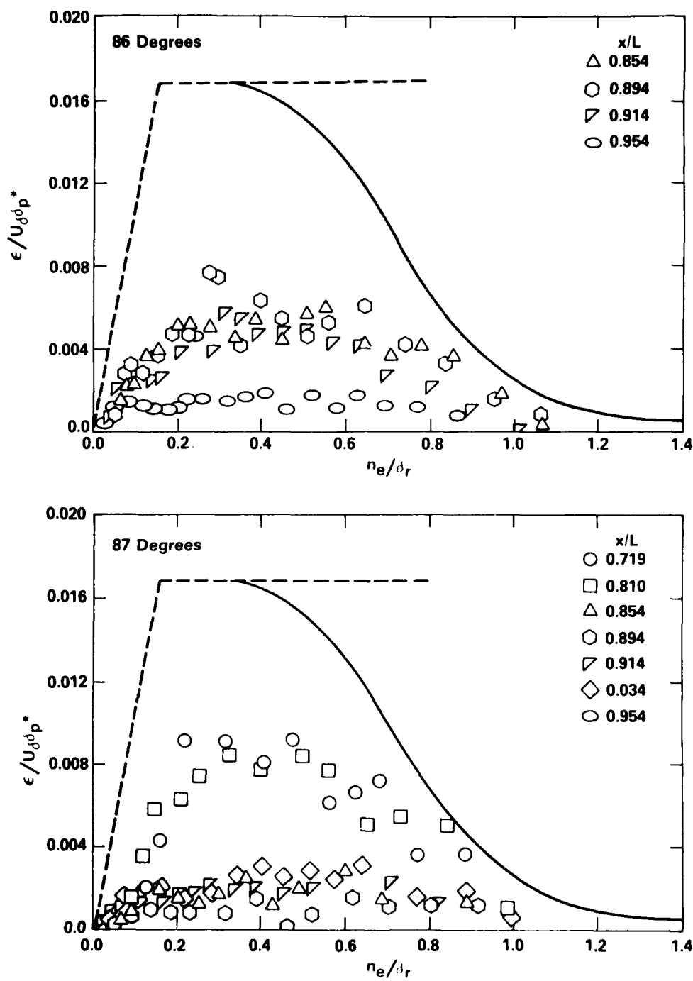
Figure 15c - Angular Locations, \theta = 86 and 87 Degrees
