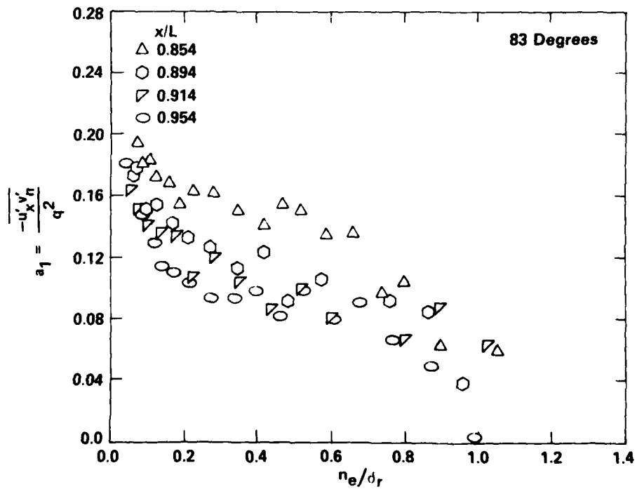
Figure 14b - Angular Locations \theta = 80 and 83 Degrees
