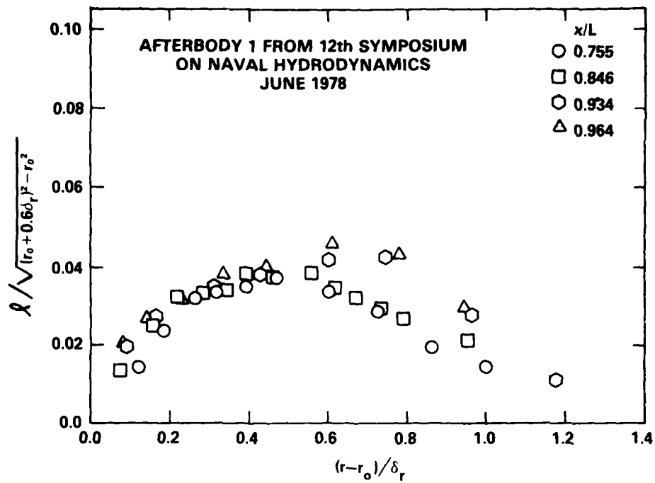
Figure 18a - Afterbody 1
