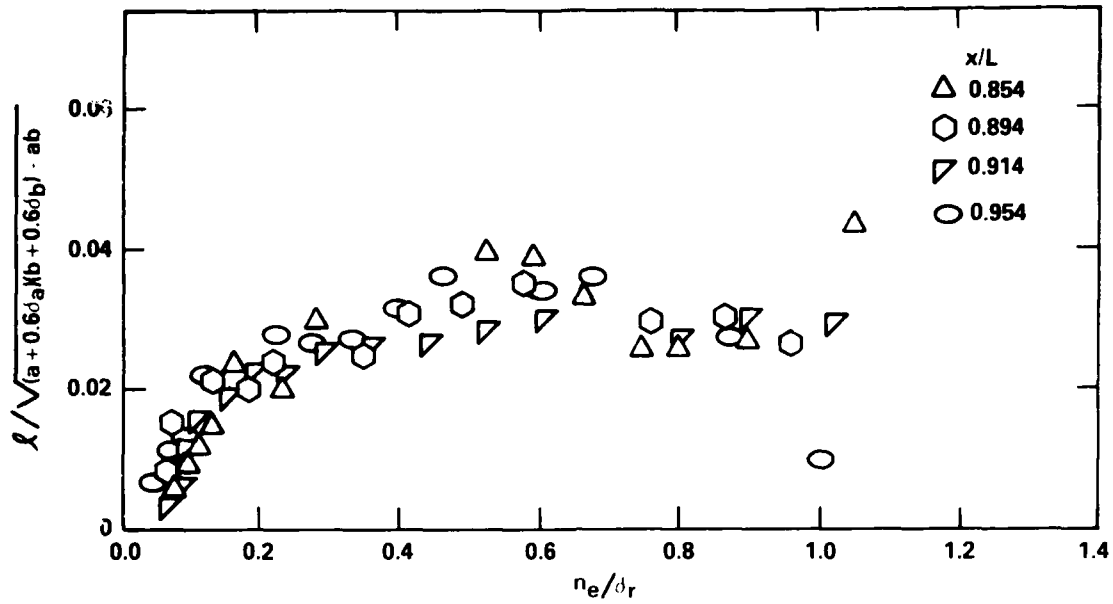
Figure 18g - Present Model, 83 Degree Plane
