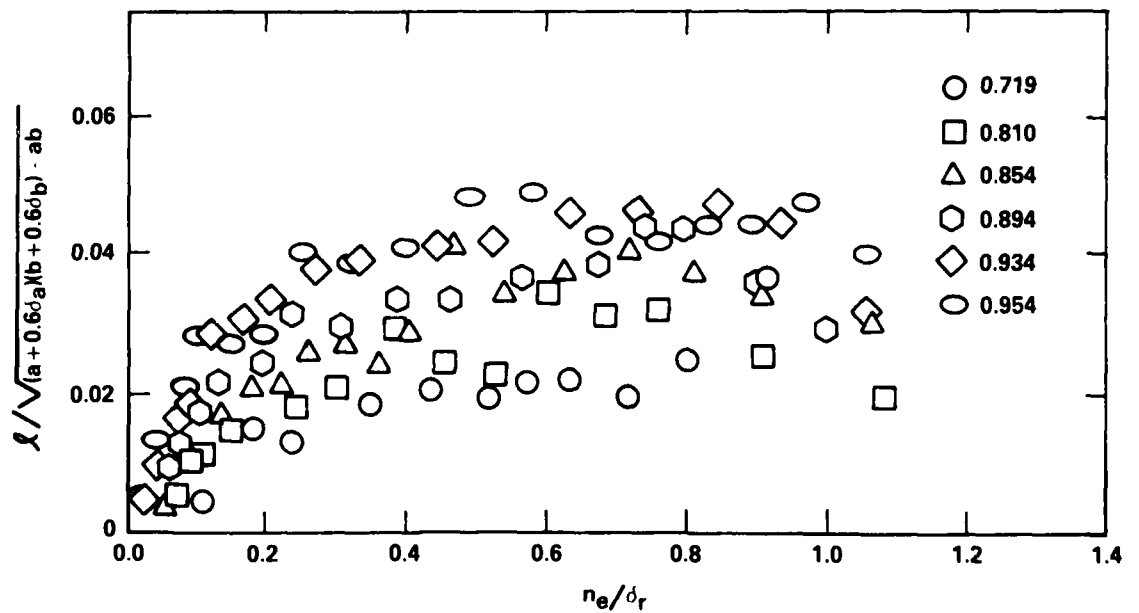
Figure 18j - Present Model, 90 Degree Plane
