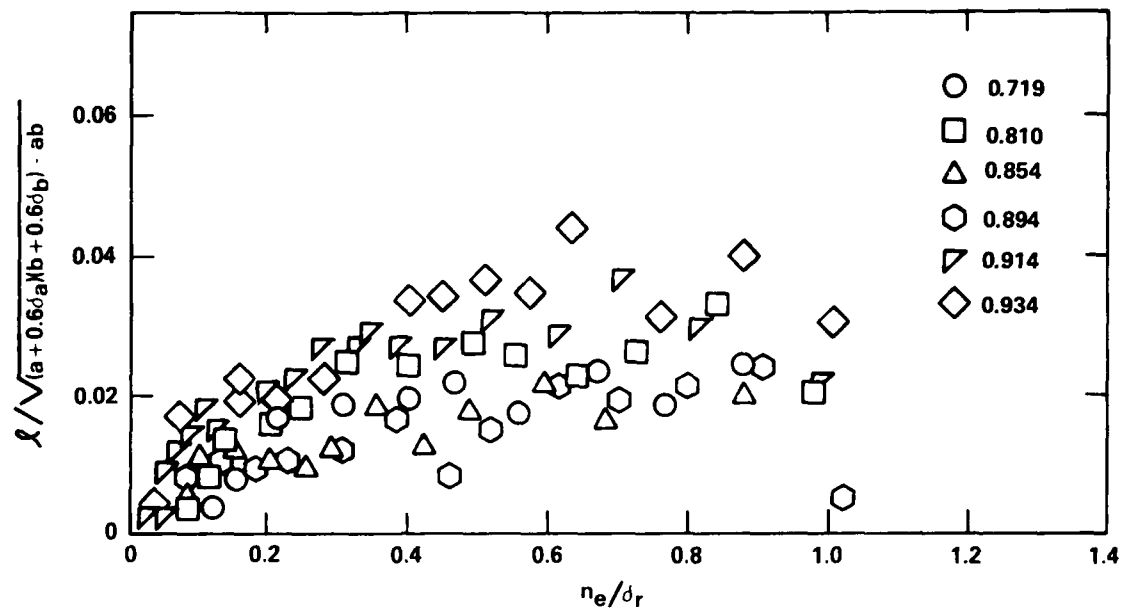
Figure 18i - Present Model, 87 Degree Plane
