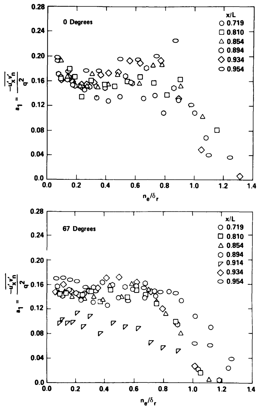
Figure 14a - Angular Locations, \theta = 0 and 67 Degrees
