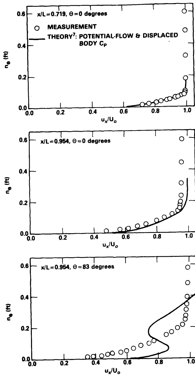
Figure 8 - Computed and Measured Mean Axial Velocity Distributions
