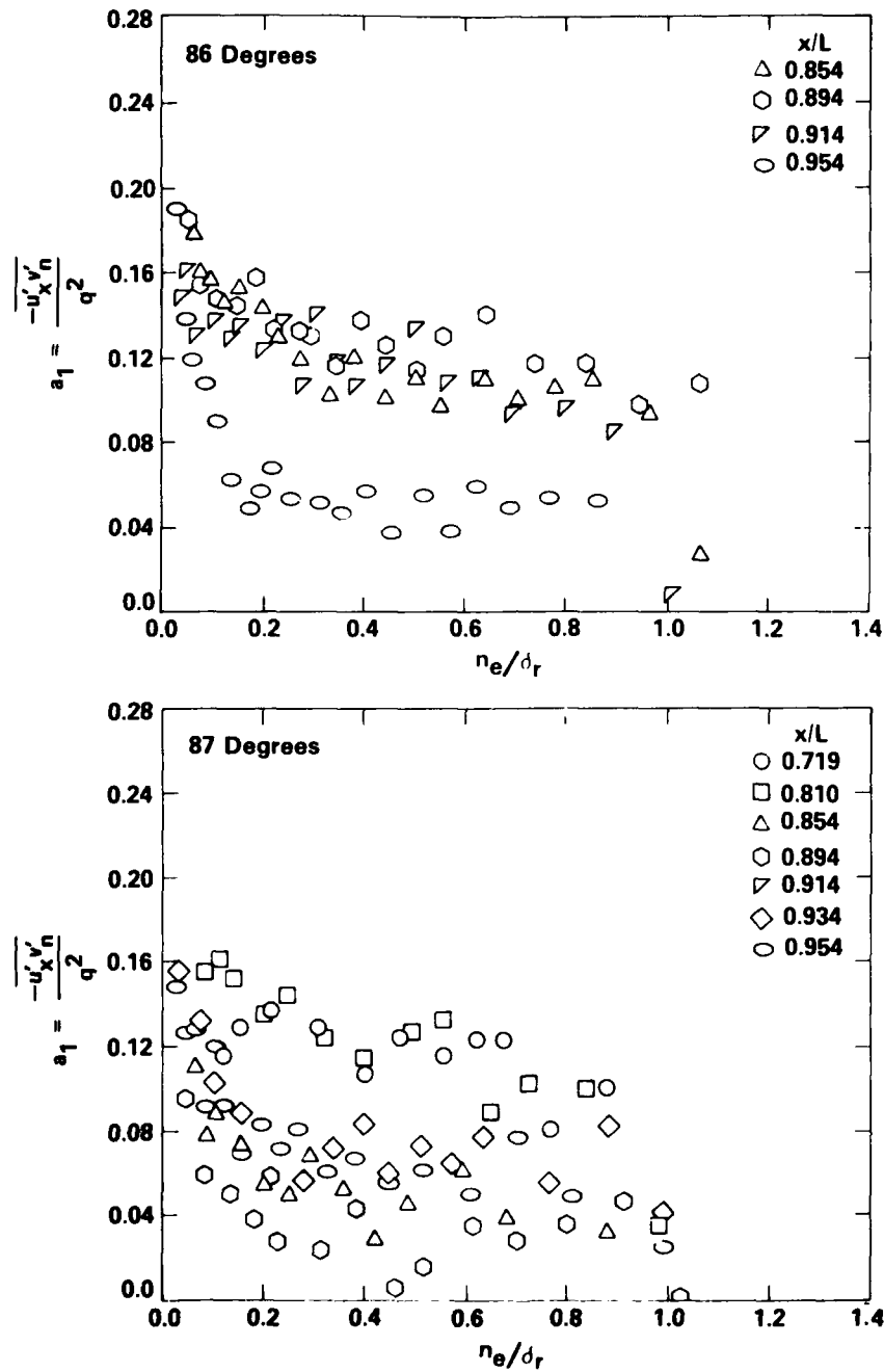
Figure 14c - Angular Locations, \theta = 86 and 87 Degrees
