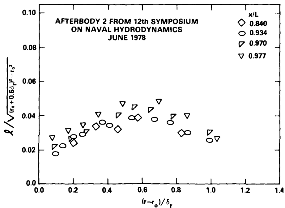
Figure 18b - Afterbody 2
