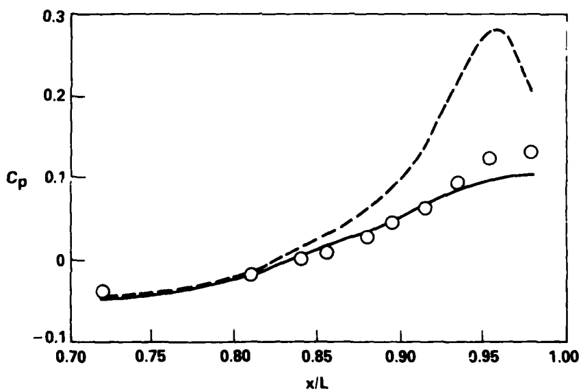
Figure 6e - \theta = 90 Degrees
