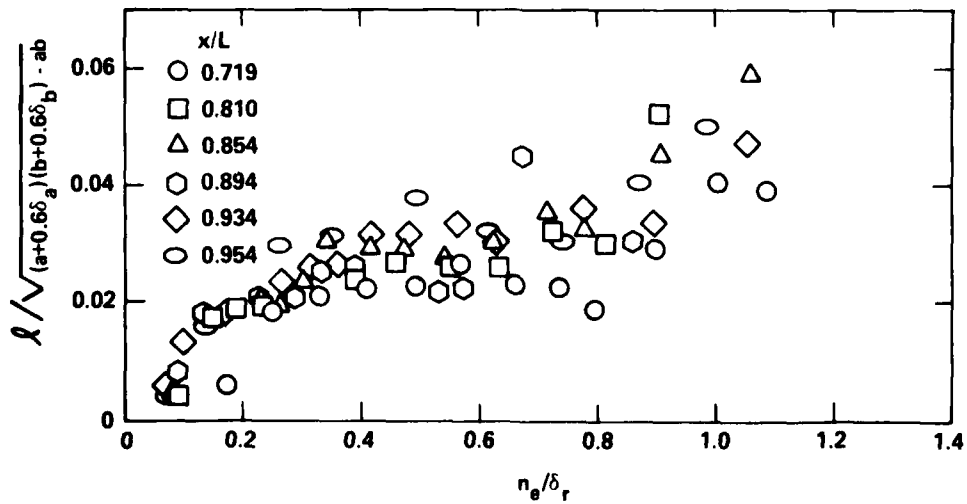
Figure 18d - Present Model, 0 Degree Plane
