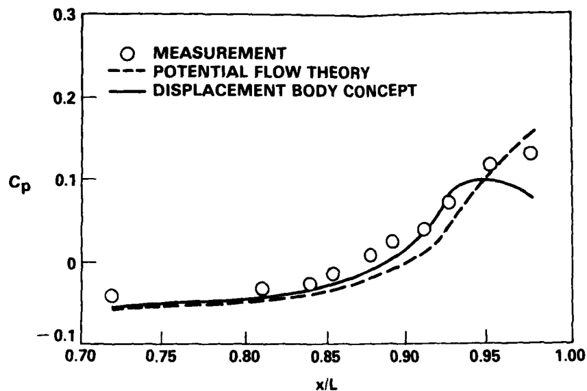
Figure 6a - \theta = 0 Degrees
