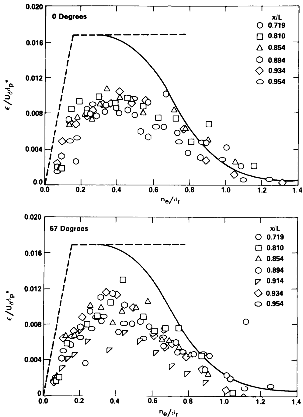
Figure 15a - Angular Locations, \theta = 0 and 67 Degrees
