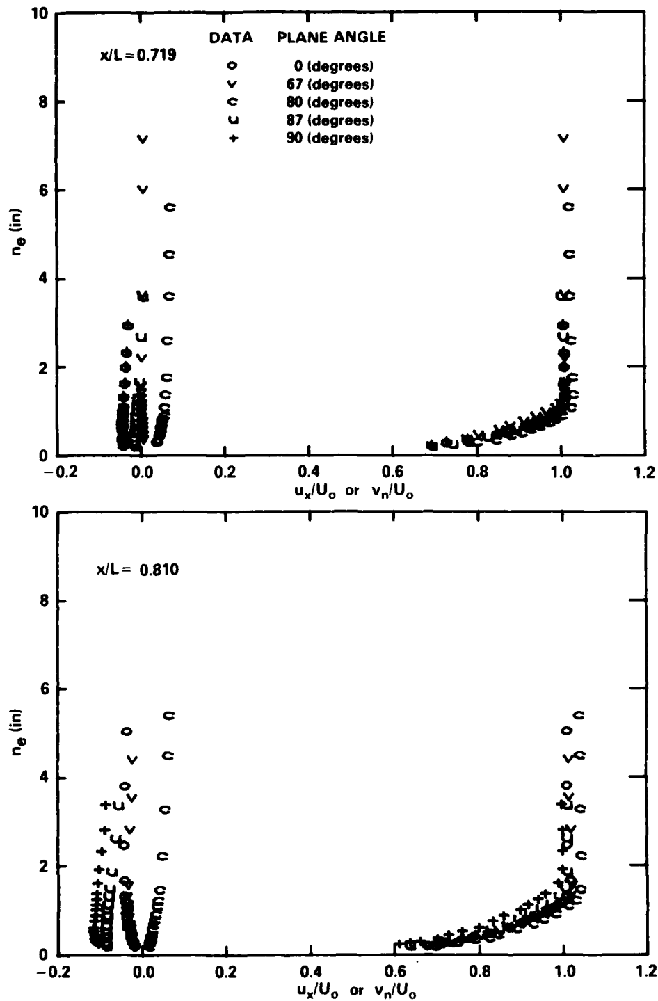
Figure 7a - Nondimensional Axial Lengths, x/L = 0.719 and 0.810
