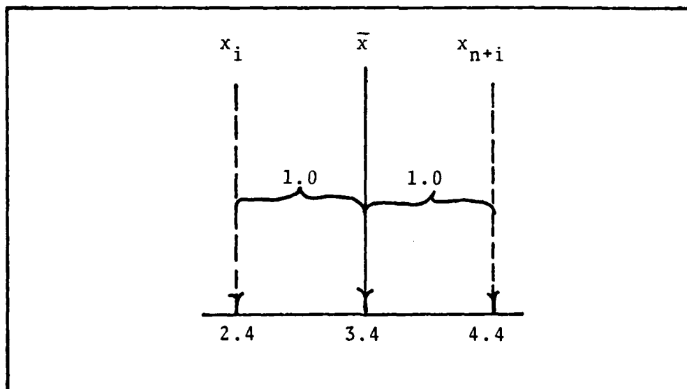
Fig 4. Doubling Samples About the Mean
