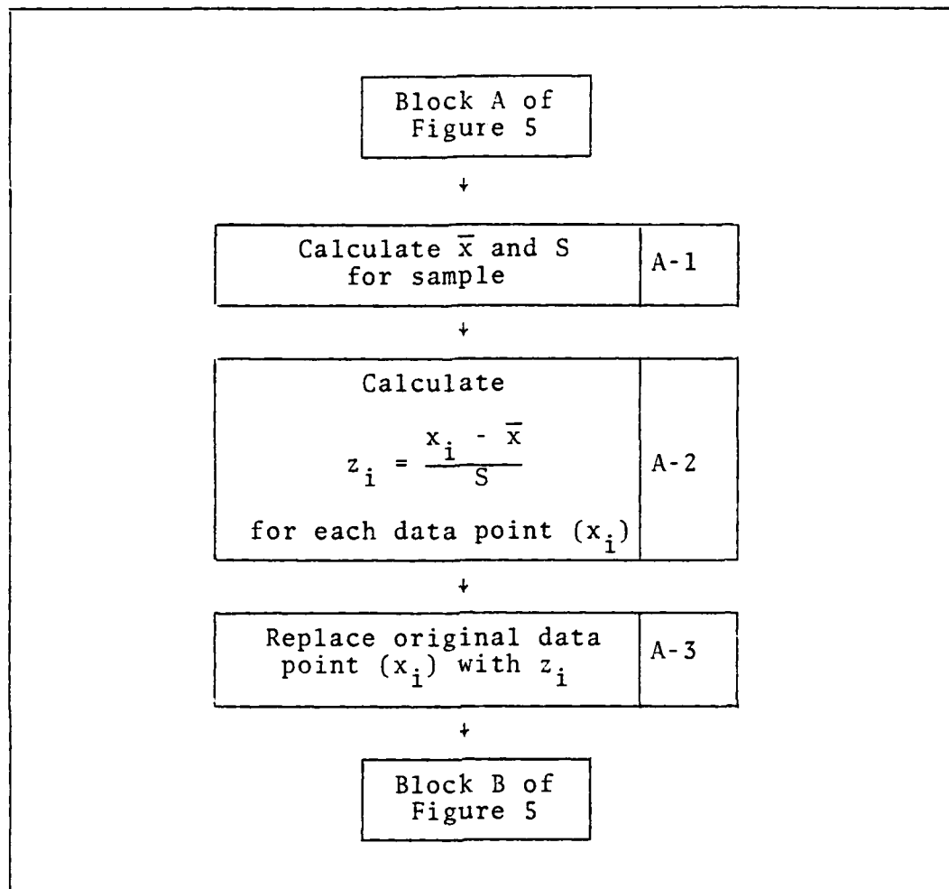
Fig 7. Program Logic for Standardizing the Data
