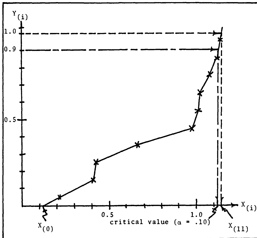
Fig 3. Example of Bootstrap Technique
