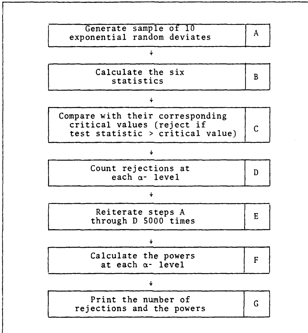
Fig 8. Flow for Typical Power Study Program
