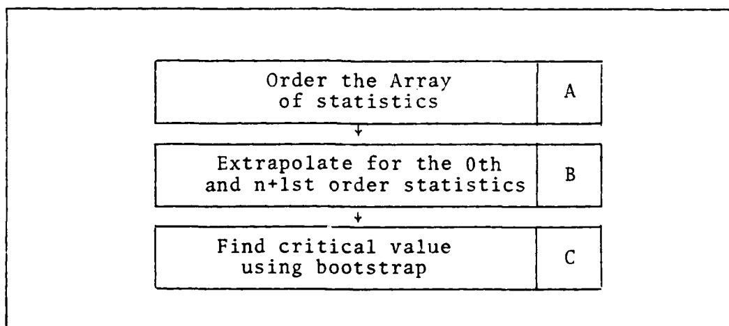
Fig 6. Subprogram for Finding Critical Values
