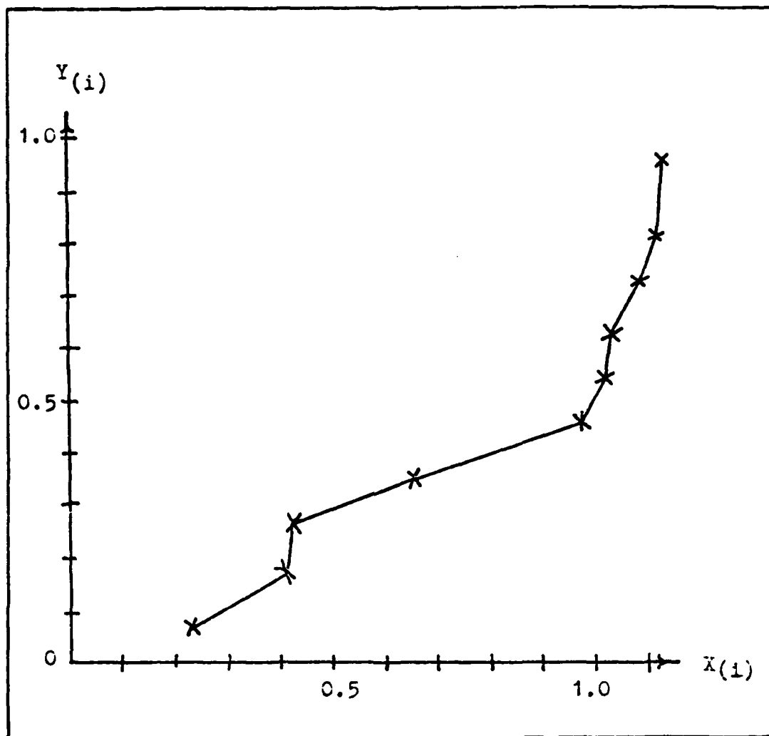
Fig. 1. Example (Order Statistics vs Median Ranks)
