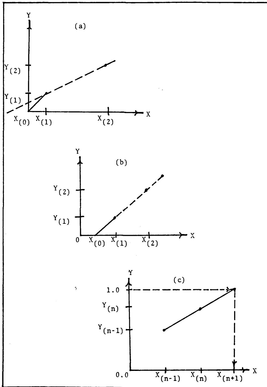
Fig 2. Three Examples of Extrapolation
