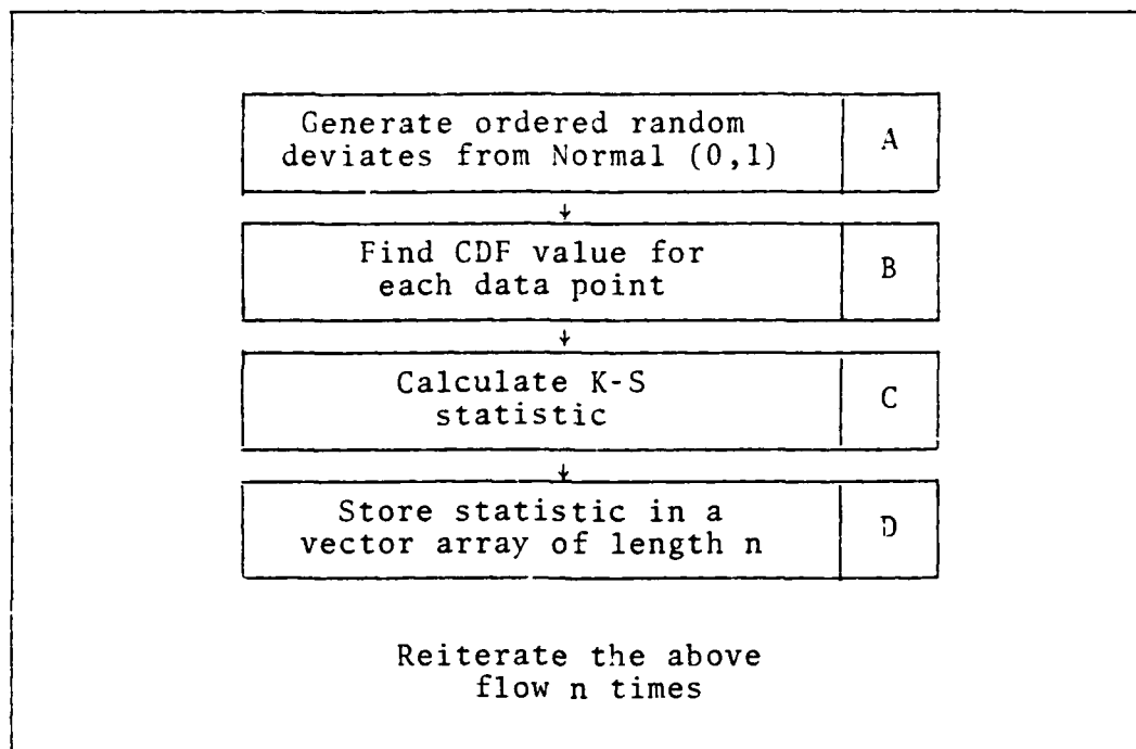
Fig 5. Subprogram for Calculating Statistics
