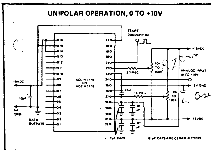
Figure 8. Twelve-Bit A/D Converter Circuit
