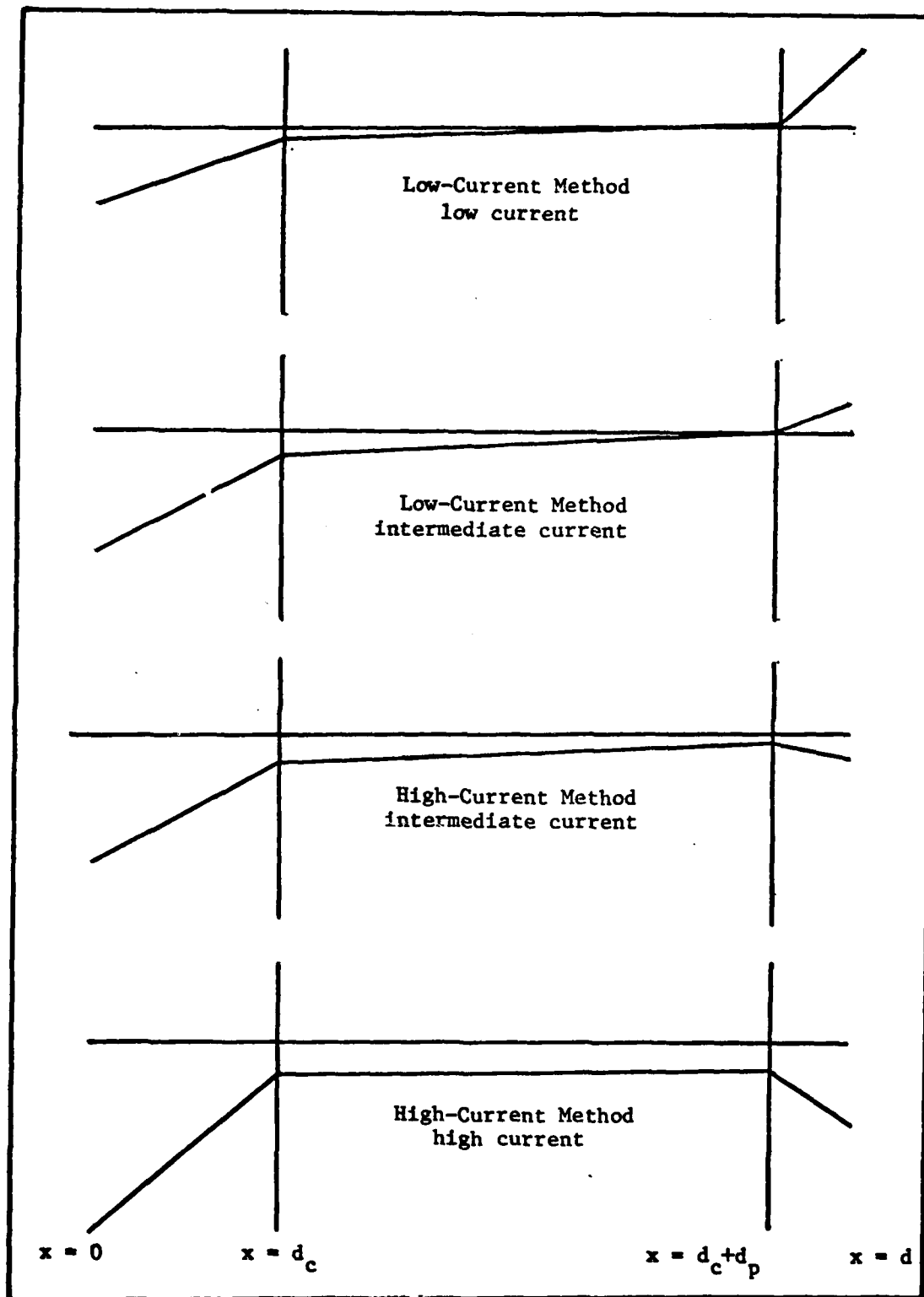
Figure 10. Discharge Electric Field for Variations of Case III Method
