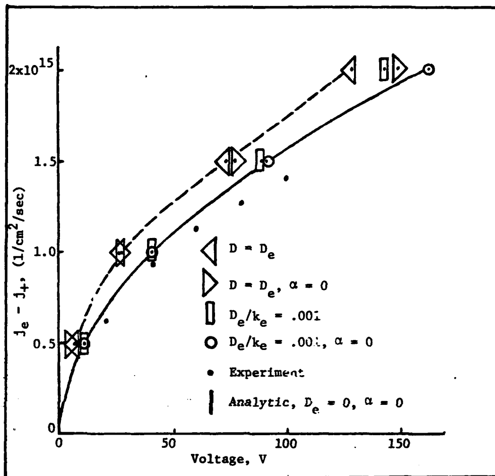
Fig. 13. Calculated and Analytic I-V Characteristics (Argon, 240 Torr, S = 3.6 \times 10^{16} \text{ 1/cm}^3/\text{sec} , with and without \alpha and D_e )
