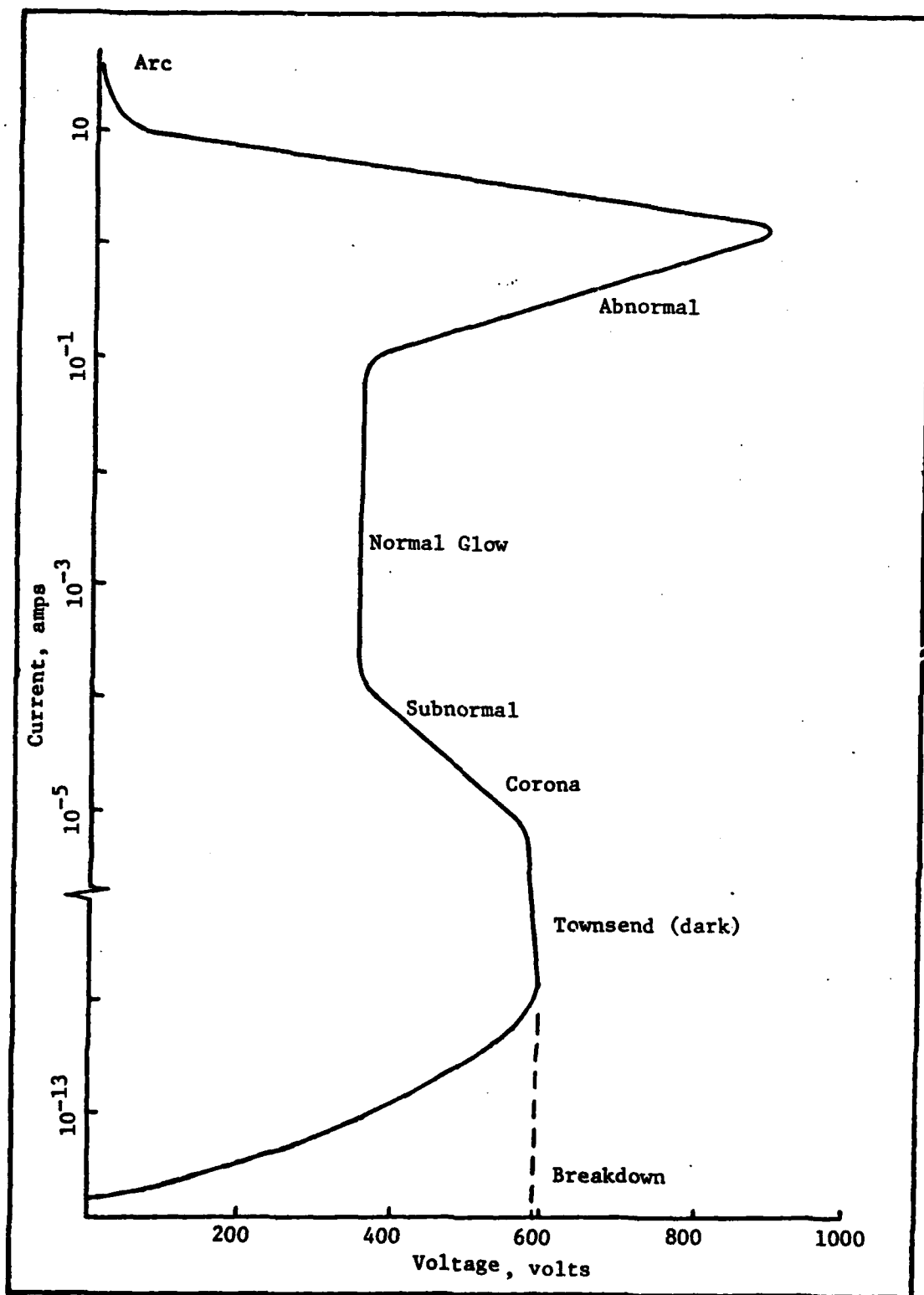
Figure 1. General Current-Voltage Characteristic (Ref. 49:211)
