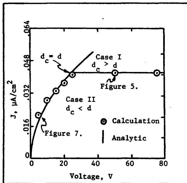
Fig. 6. I-V Characteristic for Case I and Case II ( S = 8 \times 10^{11} ) (Ref. 11:4995)
