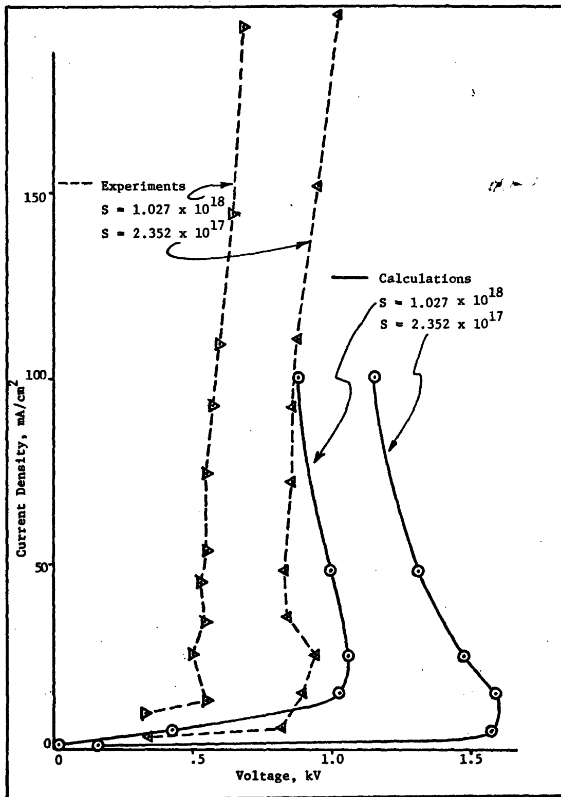
Figure 25. I-V Characteristics-Experimental and Calculated for a Methane Discharge (760 Torr, \gamma = .02 , d = 2.2 cm)
