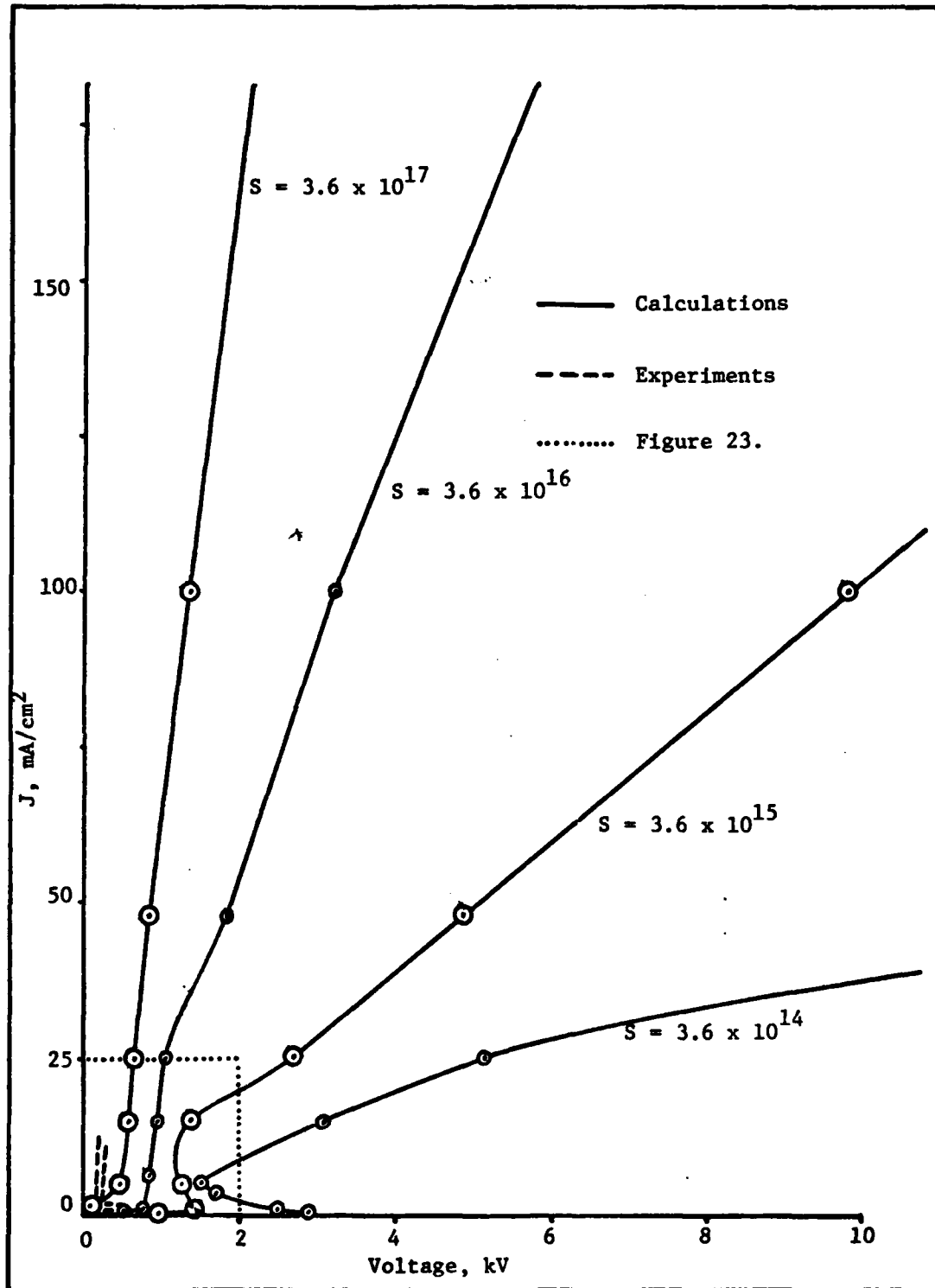
Figure 22. I-V Characteristics-Calculated for an Argon Discharge (760 Torr, \gamma = .02 , d = .3 \text{ cm} , no metastable ionization)
