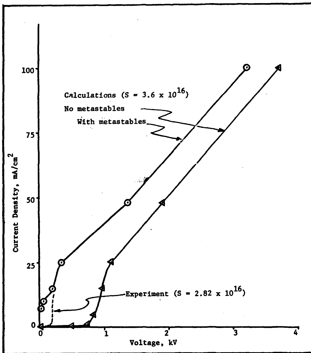
Figure 24. I-V Characteristics-Experimental and Calculated for an Argon Discharge (same parameters as Fig. 22, but with metastable ionization)
