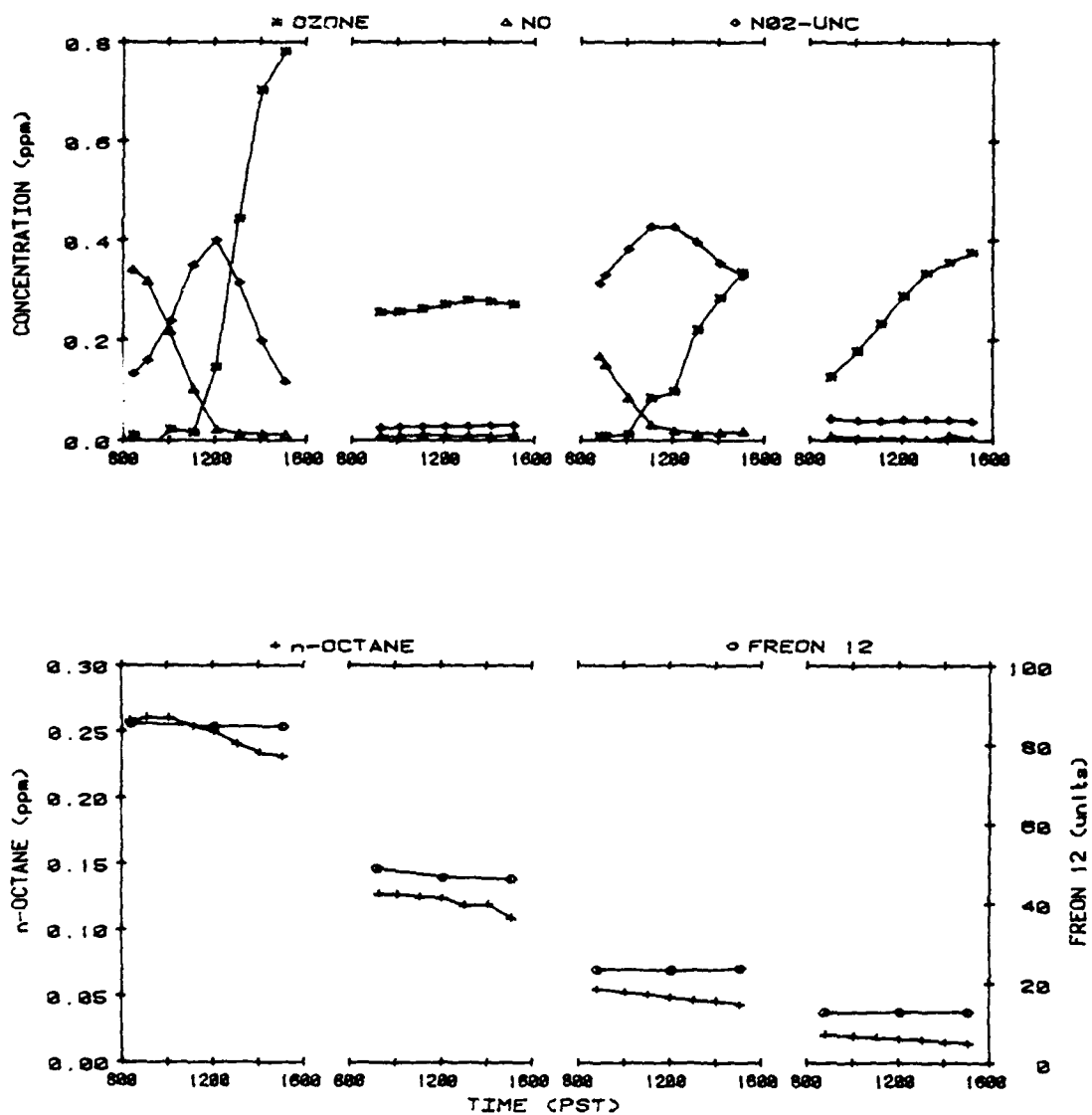
Figure 20. Concentration-Time Profiles for Selected Species, and Physical and Aerosol Measurements for the Four-Day, JP-4(Shale)-NO x Outdoor Chamber Run AFF-18.
