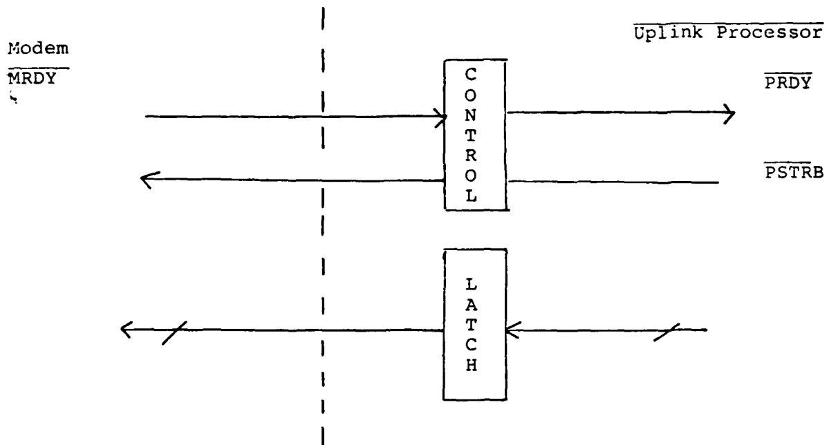
Figure 4. Current Modem - ICCU Interface PIA is ready for a new byte from the processor.
