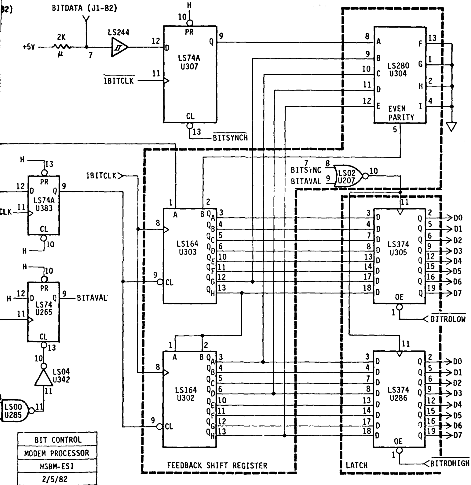
Figure 6. BIT Control
