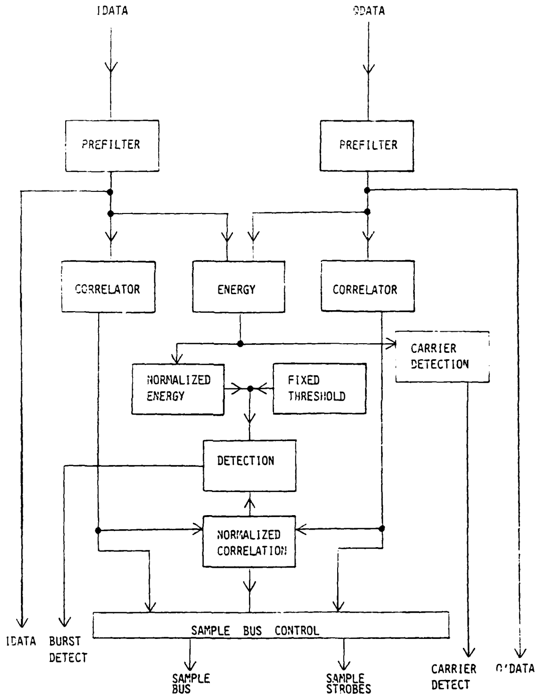
Figure 2. Data Processing Structure
