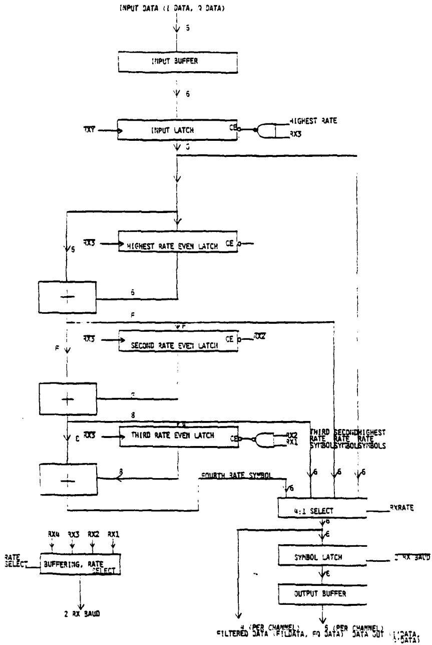
Figure 9. Prefilter Implementation
