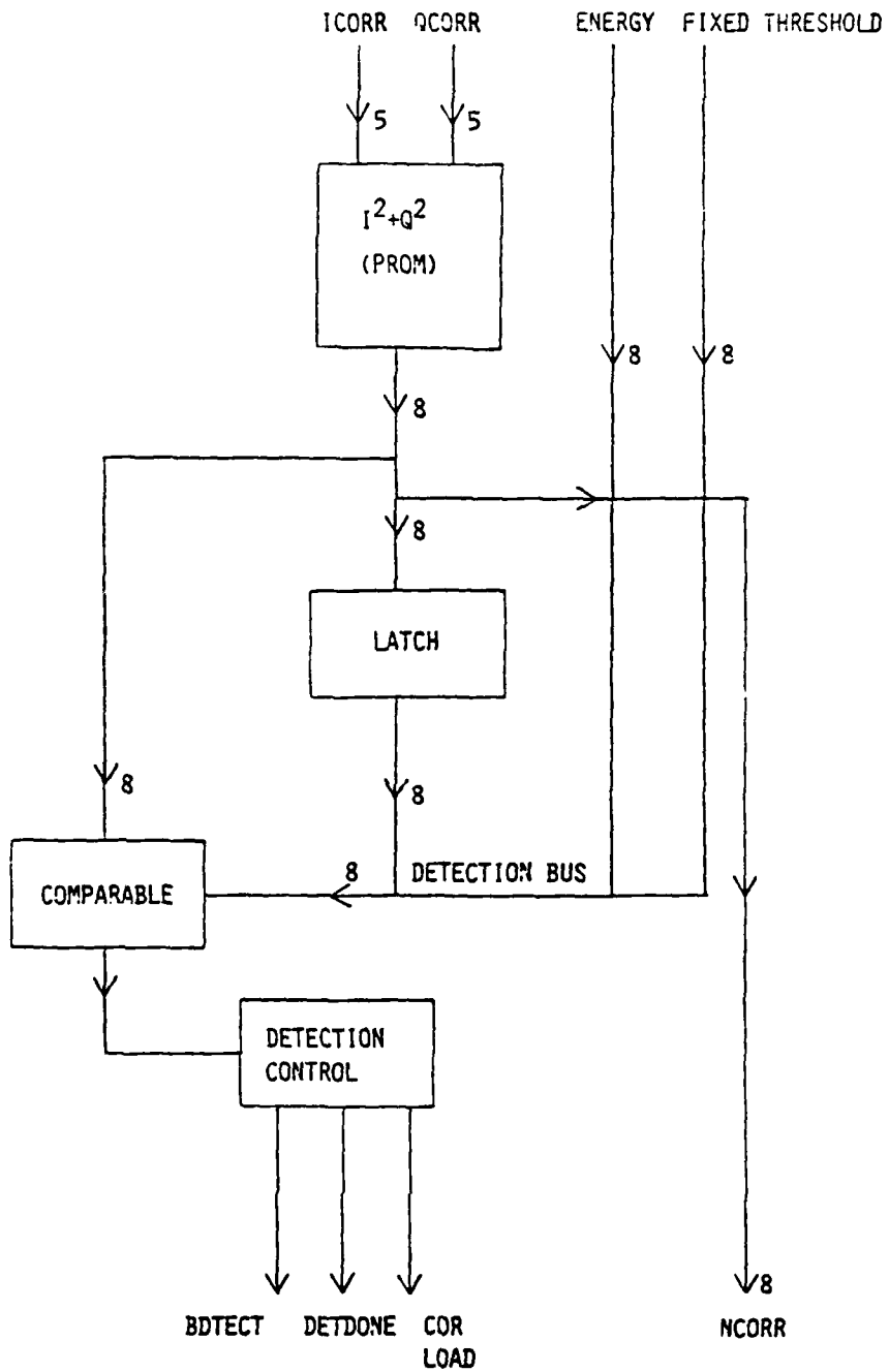
Figure 16. Detection Implementation
