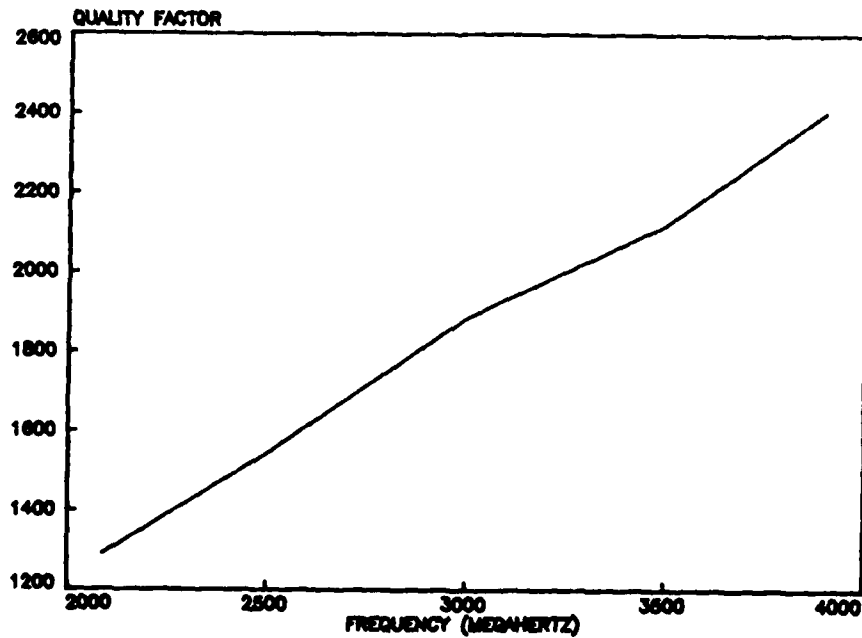
Figure 15. Quality Factor versus Frequency.
