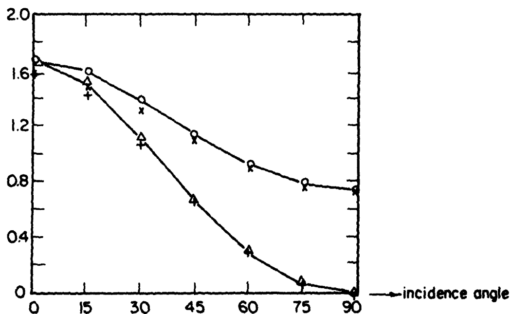
Fig. 15. Transmission coefficient for a circular aperture. R = 0.02\lambda, 0.25\lambda in (a), (b). + : computed result for E_{\perp} -polarization. \times : computed result for E_{\parallel} -polarization \Delta, 0 : corresponding data from [3].
