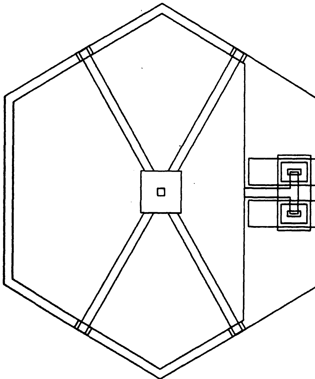
Figure 40. CALMA Layout of Capacitor Cell
