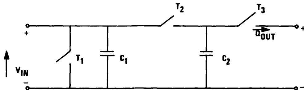
Figure 37. Current Splitter
