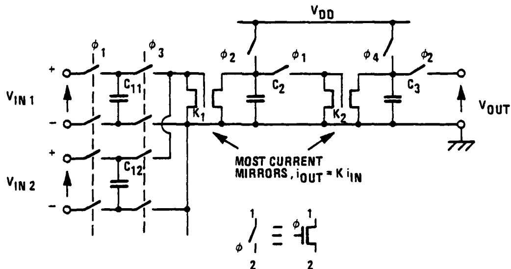
b. Circuit diagram of SC section. Clock phases are mutually exclusive and follow index sequence
