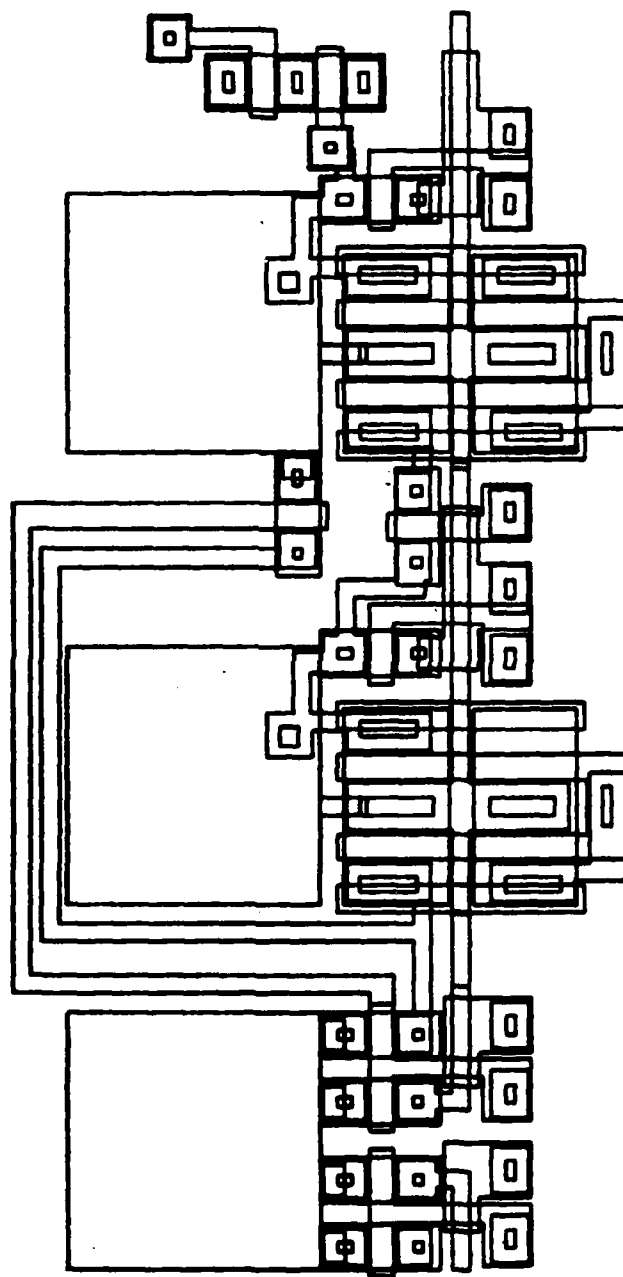
Figure 33. CALMA Layout of First-Order Low-Pass Recursive SC Filter
