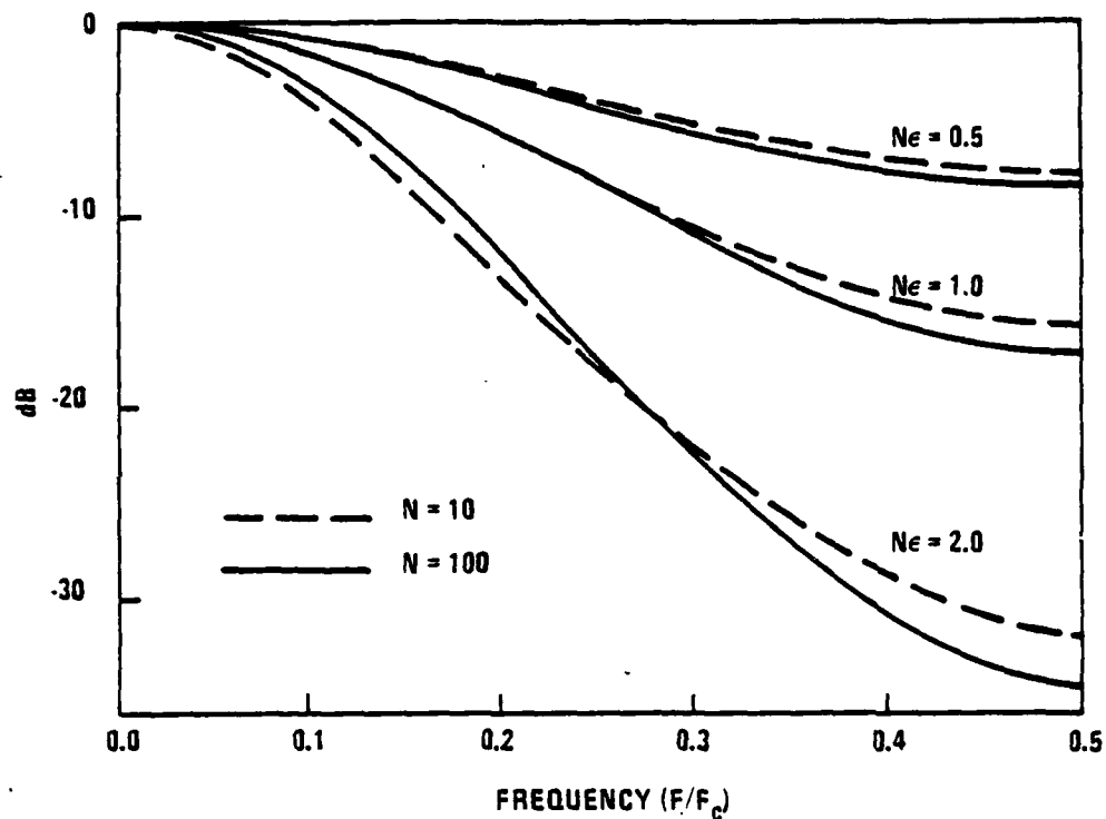
Figure 7. Frequency Response of CCD Delay Lines for Various Transfer Inefficiencies and for 10 or 100 stages
