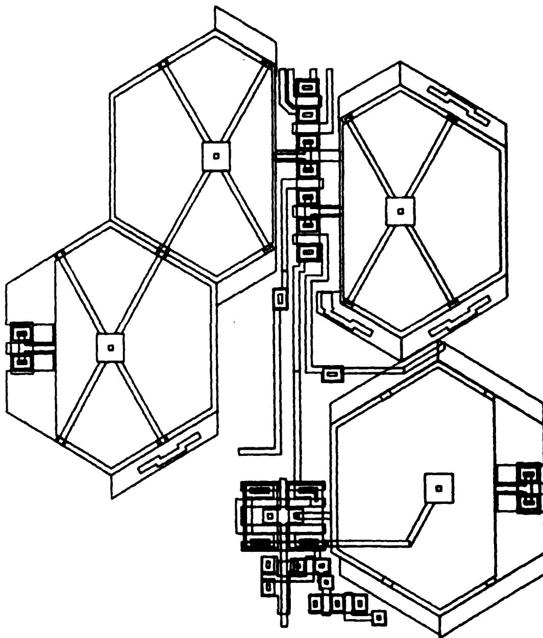
Figure 39. CALMA Layout of Switching Portion of Charge Divider
