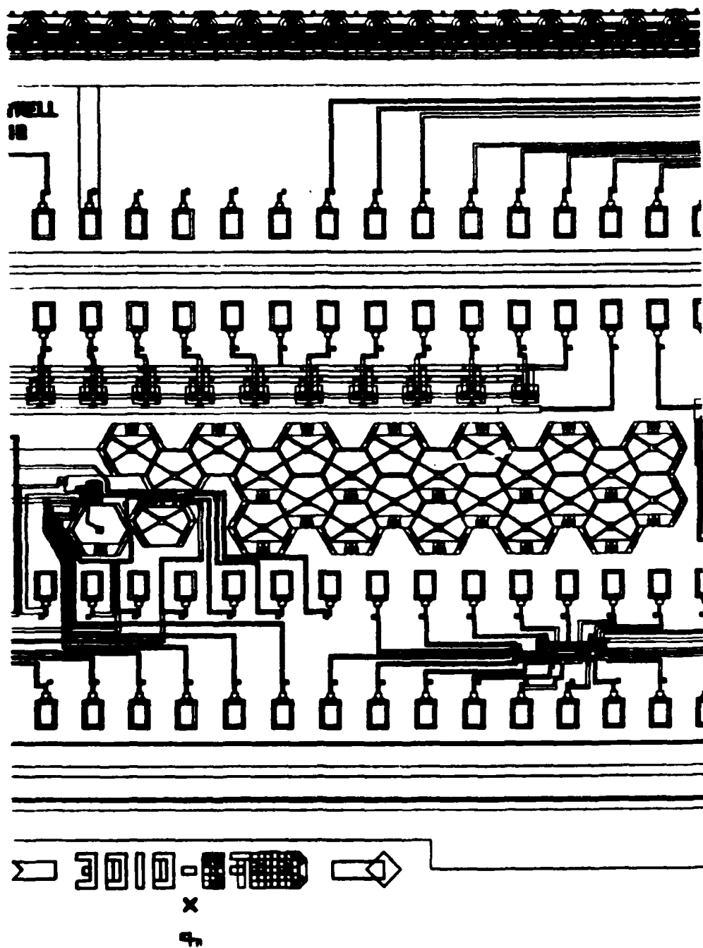
Figure 38. CALMA Layout of Charge Divider
