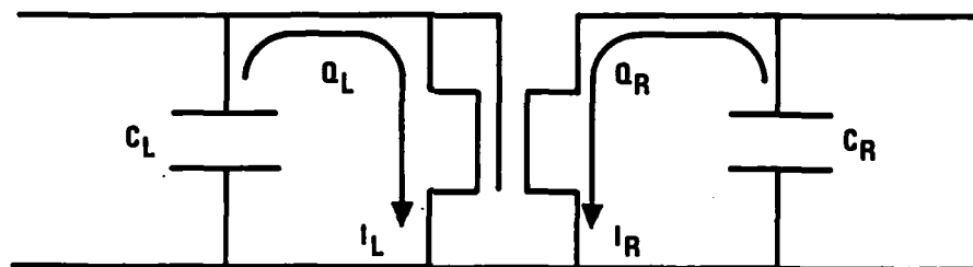
Figure 30. Current Mirror Portion of SC-UDM
