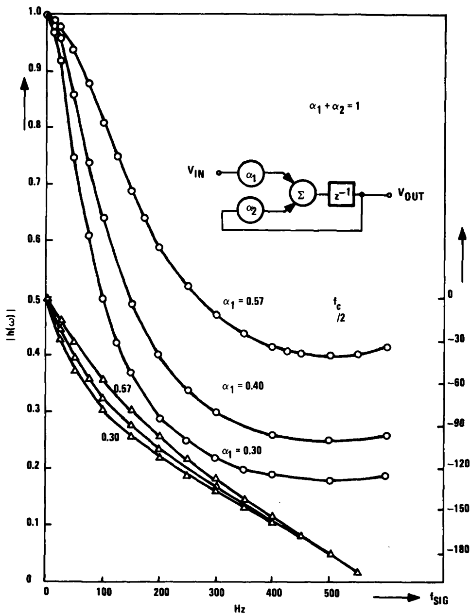
Figure 25. First-Order Recursive Low-Pass Filter
