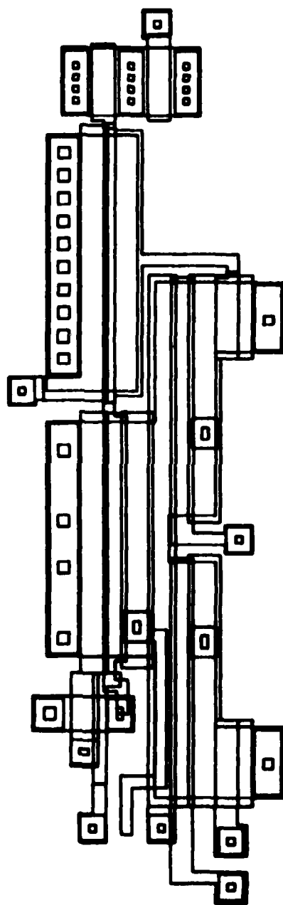
Figure 19. CALMA Layout of Improved SCCD-UDM
