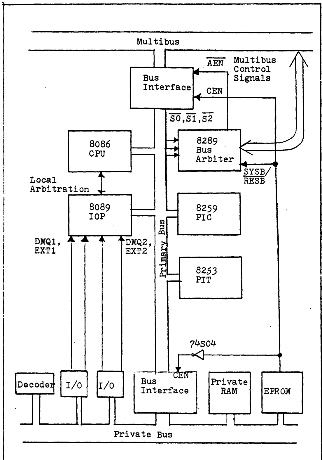
Figure 3-5 Network Subsystem
