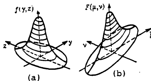
Fig. 1.14. Calculation of the spectrum and shape of the output signal of a multidimensional filter.
