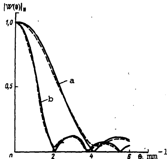
Fig. 3.11. One-dimensional cuts of the spatial frequency transfer functions of diaphragms with circular apertures: (a) d=0.3 \text{ mm} ; (b) d=0.6 \text{ mm} .
