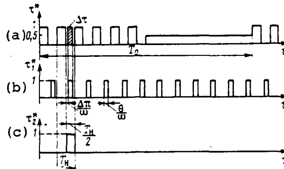
Fig. 2.3. Waveform at the output of a radiant-energy detector when a modulating disk having a nonideal raster pattern is used (a), and the form of auxiliary functions that produce \Delta\tau(t) .
