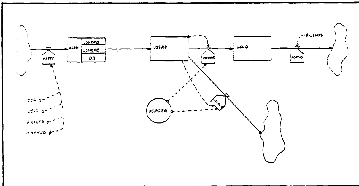
Figure 30. US Force Requests Sector---Flow Diagram
