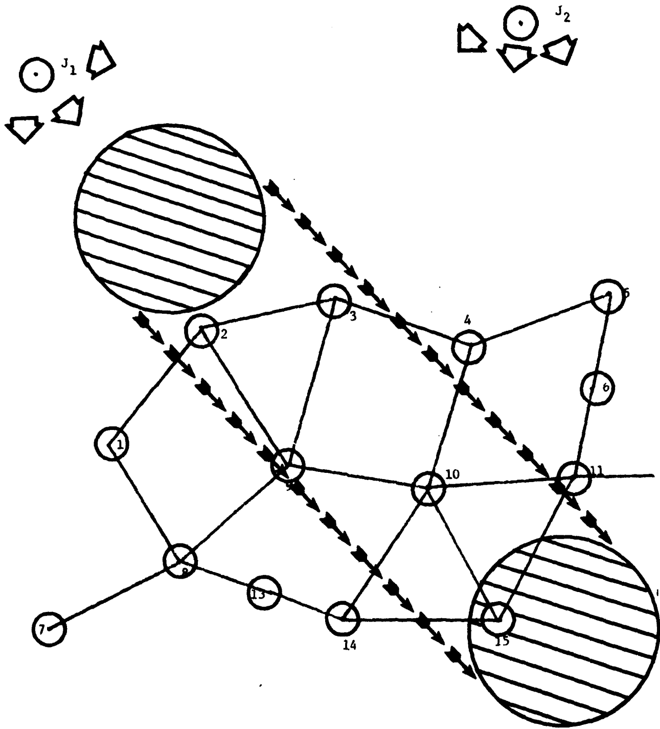
Figure 11. 60 km Diameter Rain Storm
