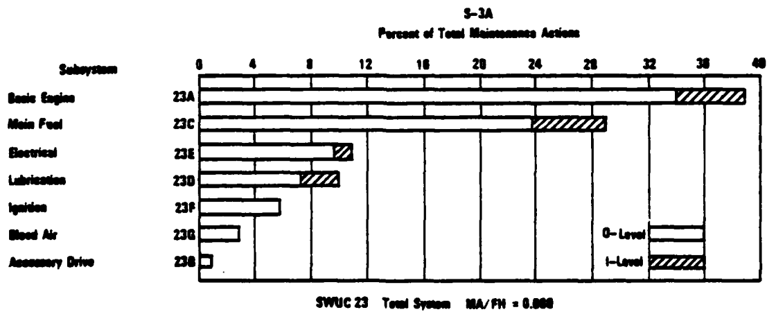
Figure 18. Distribution of S-3A Engine System Maintenance (SWUC 23)
