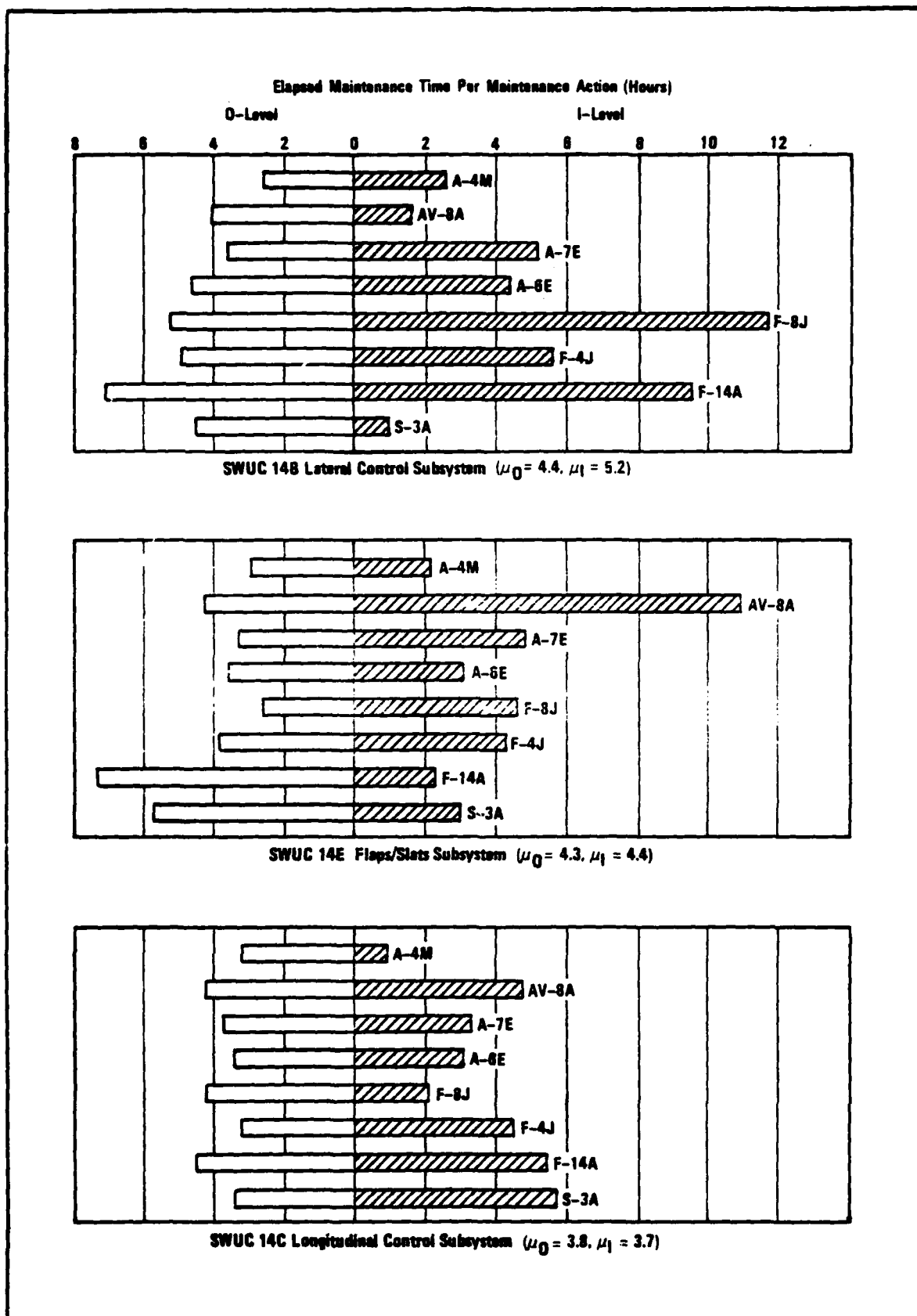
Figure 9. Average Repair Time for Major Flight Controls Subsystems (SWUC 14)
