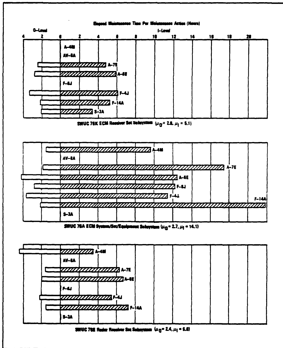
Figure 37. Average Repair Time for Major ECM Subsystems (SWUC 76)
