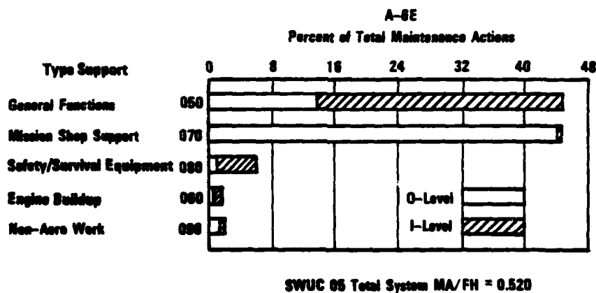
Figure 42. Distribution of A-6E Shop Support Maintenance (SWUC 05)
