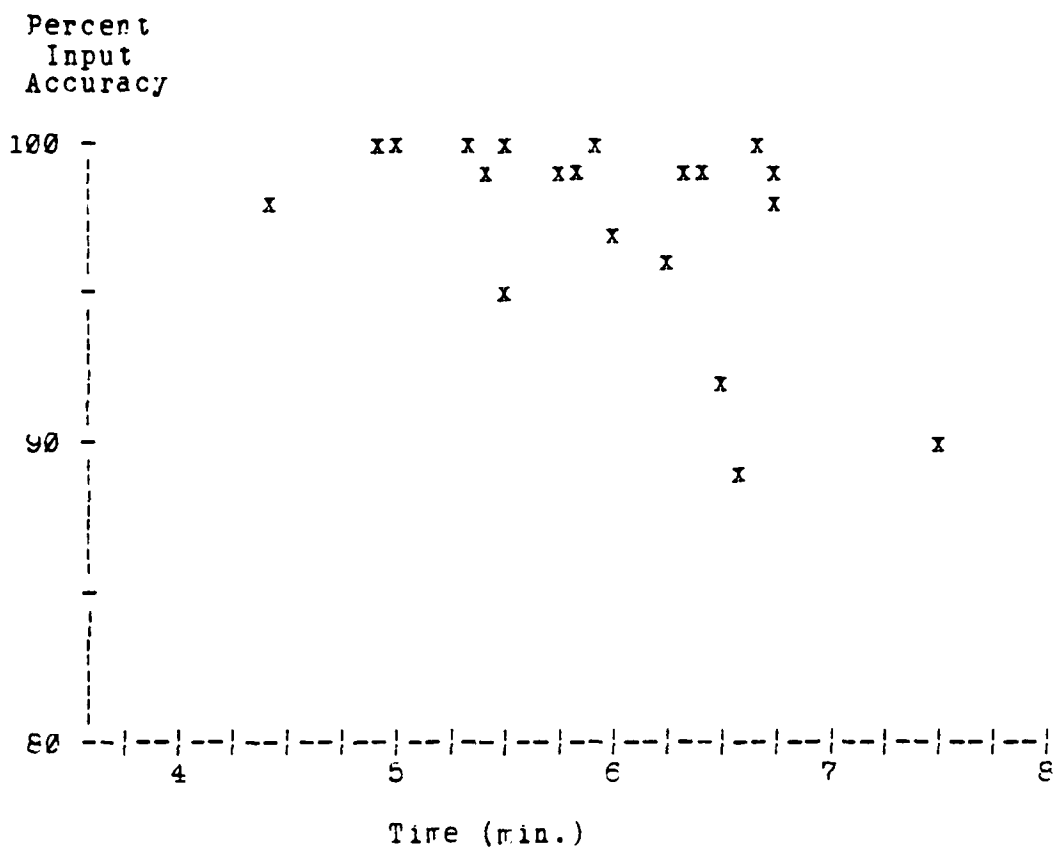
Figure 23. Percent Input Accuracy by Time (Single-Space)
