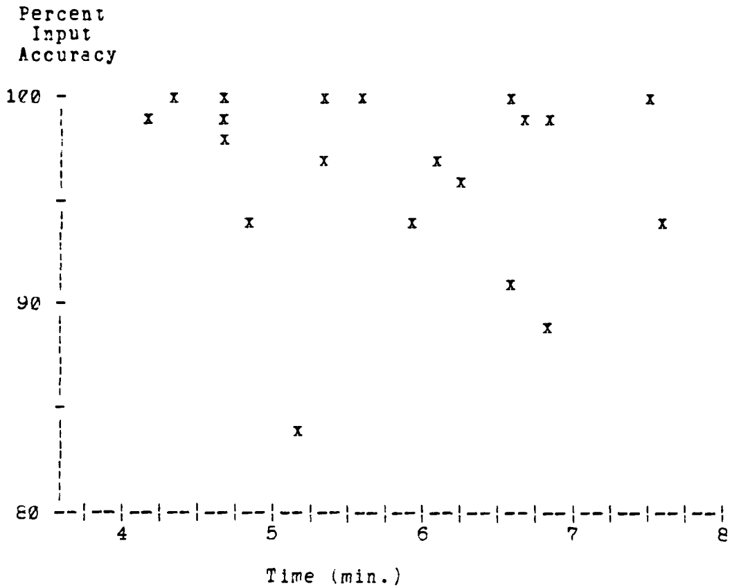
Figure 25. Percent Input Accuracy by Time (Inverse-Video)
