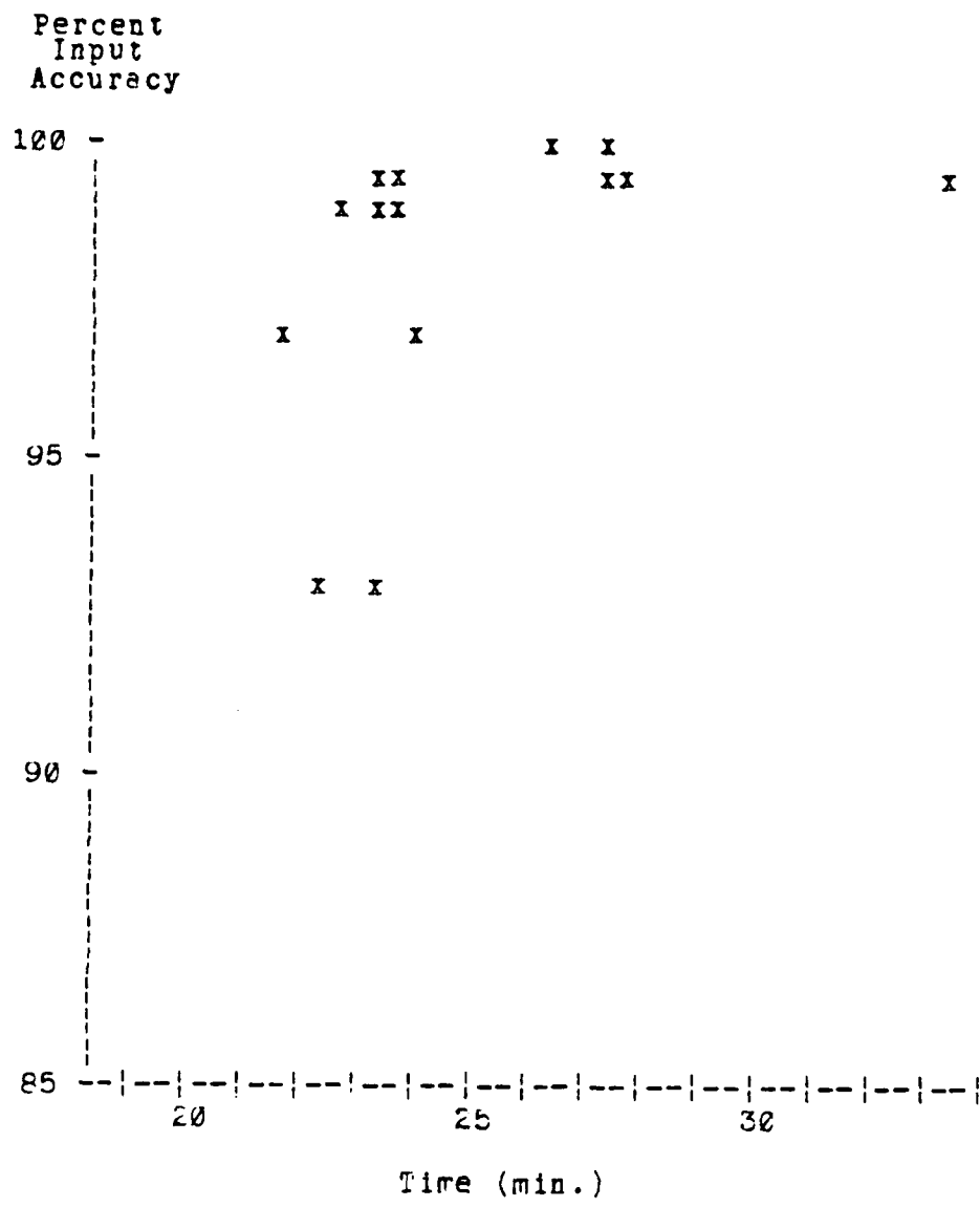
Figure 17. Percent Input Accuracy by Time For IKB
