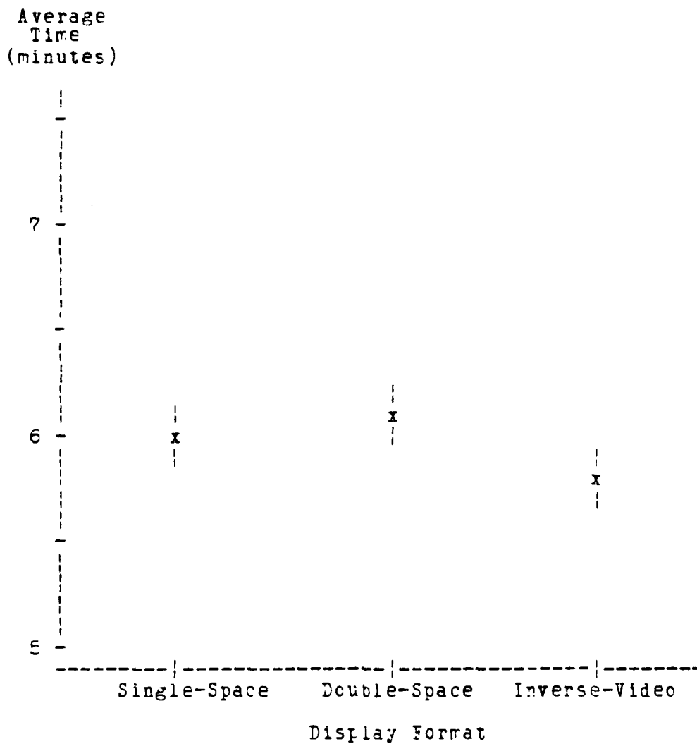
Figure 20. Mean Time And Standard Deviation to Complete Update Using Each Display Format
