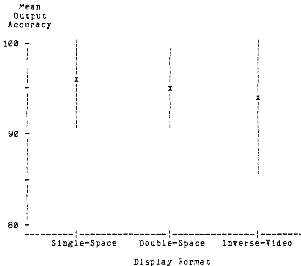
Figure 22. Mean Output Accuracy And Standard Deviation For Each Display Format
