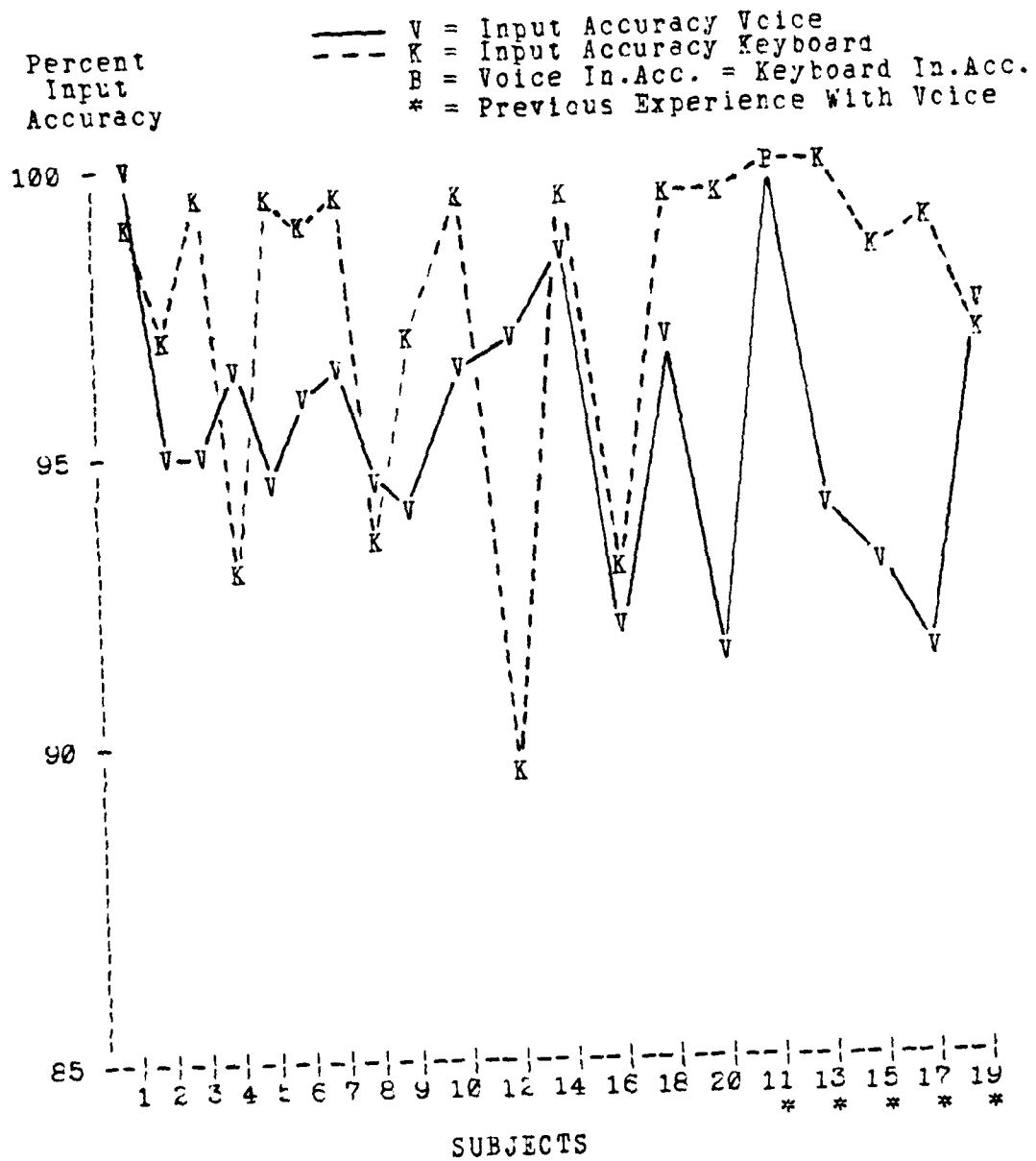
Figure 14. Input Accuracy by Subject
