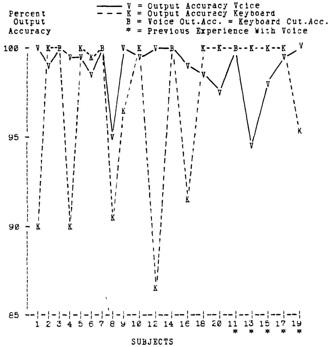
Figure 15. Output Accuracy by Subject
