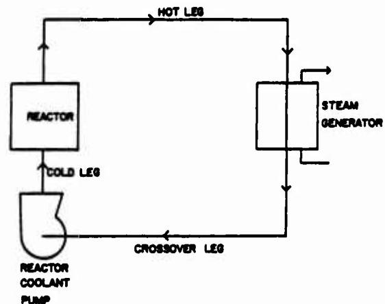
Figure 1. Typical Nuclear Steam Supply System
