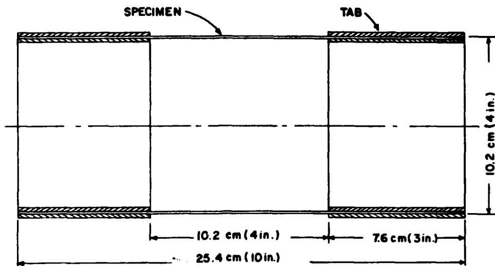
Figure 1. Tubular Specimen Geometry
