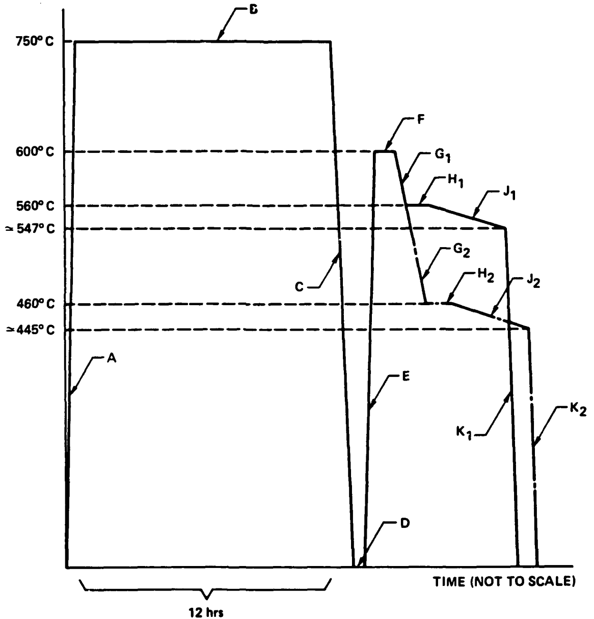
Fig. 2. Temperature-time profile of the LPE growth cycle of Al_xGa_{1-x}As_{1-y}Sb_y
